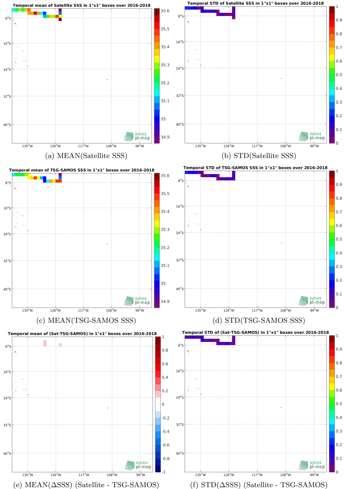
Figure 6: Temporal mean (left) and STD (right) of SSS from SMAP-L3-RSS-V3-8DAY-RUNNING-70KM (top), TSG-SAMOS (middle), and of \Delta SSS (Satellite - TSG-SAMOS). Only match-up pairs are used to generate these maps.
