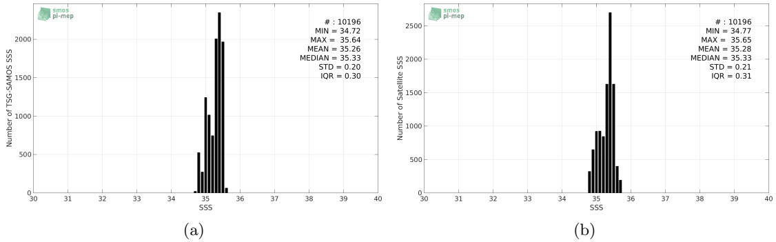
Figure 2: Histograms of SSS from TSG-SAMOS (a) and SMAP-L3-RSS-V3-8DAY-RUNNING-70KM (b) considering all match-up pairs per bins of 0.1 over the OTT zone Pi-MEP region and for the full satellite product period.
