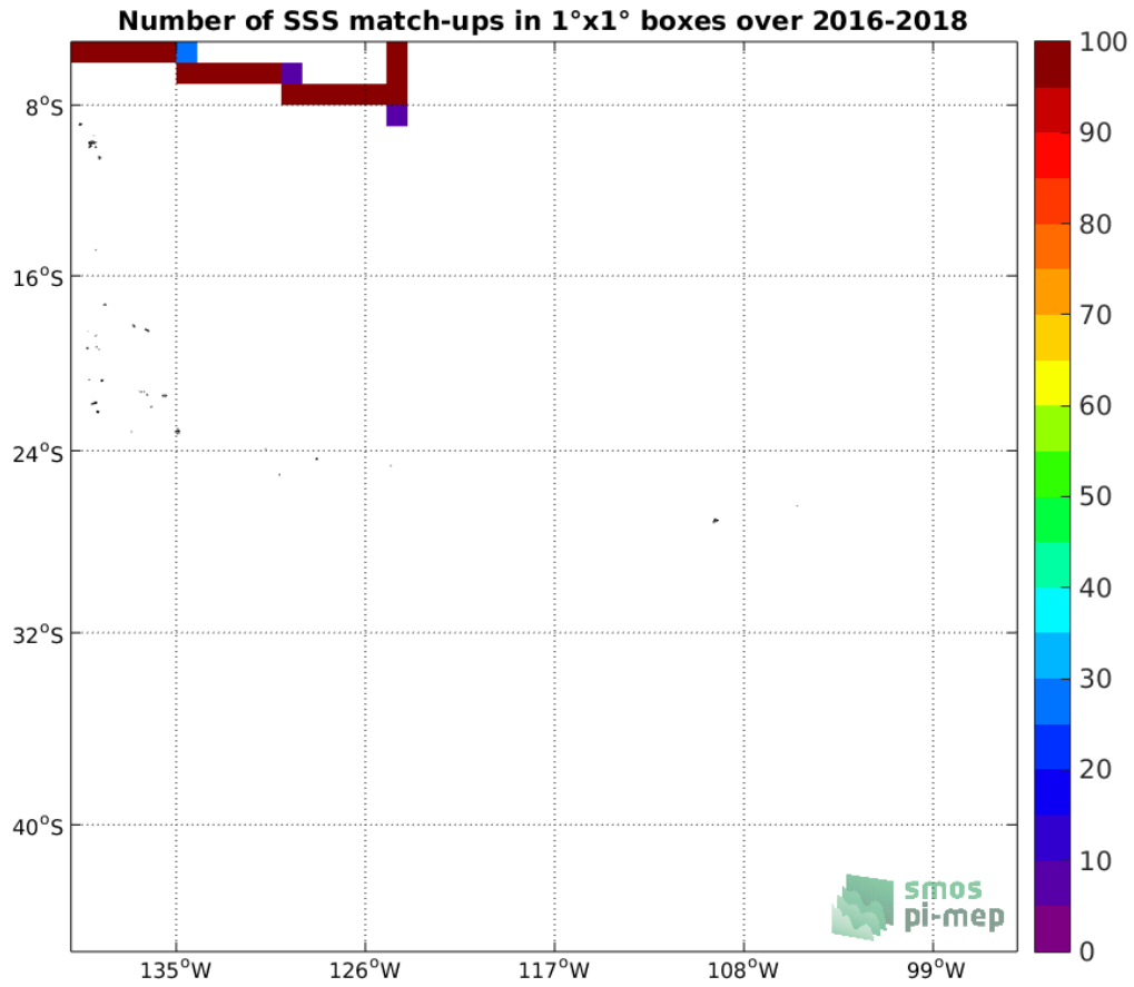
Figure 4: Number of SSS match-ups between TSG-SAMOS SSS and the SMAP-L3-RSS-V3-8DAY-RUNNING-70KM SSS product for the OTT zone Pi-MEP region over 1°x1° boxes and for the full satellite product period.
