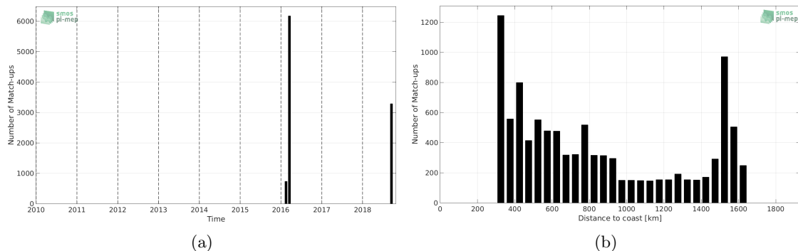
Figure 1: Number of match-ups between TSG-SAMOS and SMAP-L3-RSS-V3-8DAY-RUNNING-70KM SSS as a function of time (a) and as function of the distance to coast (b) over the OTT zone Pi-MEP region and for the full satellite product period.
