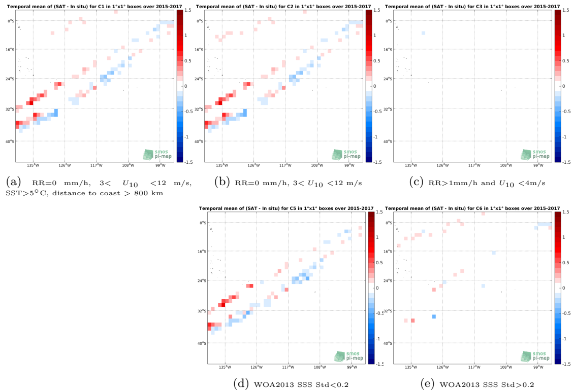
Figure 12: Temporal mean gridded over spatial boxes of size 1^\circ \times 1^\circ of \Delta SSS (SMAP-L3-RSS-V3-8DAY-RUNNING-70KM - TSG-LEGOS-DM) for 5 different subdatasets corresponding to:RR=0 mm/h, 3 < U_{10} < 12 m/s, SST >5^\circ\text{C} , distance to coast > 800 km (a), RR=0 mm/h, 3 < U_{10} < 12 m/s (b), RR >1 mm/h and U_{10} < 4 m/s (c), WOA2013 SSS Std <0.2 (d), WOA2013 SSS Std >0.2 (e).
