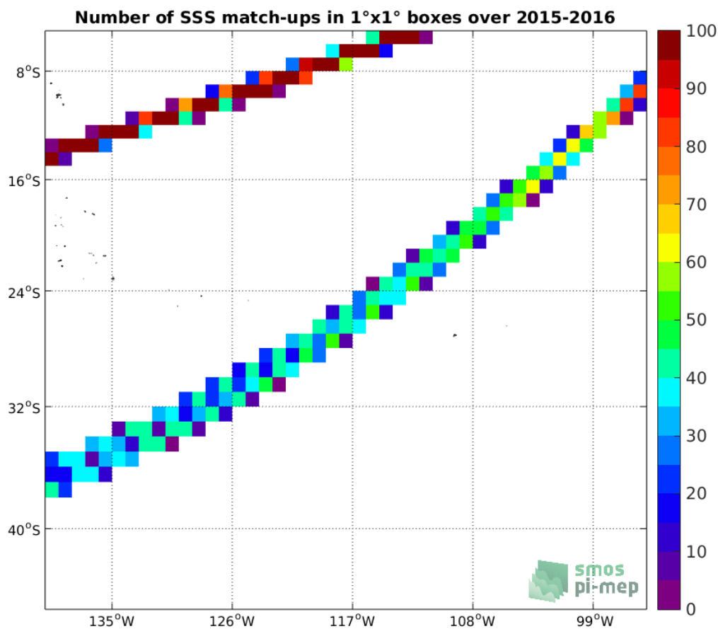
Figure 4: Number of SSS match-ups between TSG-LEGOS-DM SSS and the SMAP-L3-RSS-V3-8DAY-RUNNING-70KM SSS product for the OTT zone Pi-MEP region over 1°x1° boxes and for the full satellite product period.
