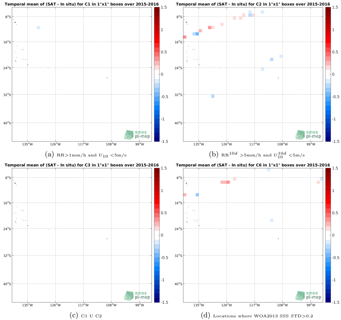
Figure 12: Temporal mean gridded over spatial boxes of size 1^\circ \times 1^\circ of \Delta SSS (SMAP-L3-RSS-V3-8DAY-RUNNING-70KM - TSG-LEGOS-DM) for 4 different subdatasets corresponding to: RR > 1\text{mm/h} and U_{10} < 5\text{m/s} (a), RR^{10d} > 5\text{mm/h} and U_{10}^{10d} < 5\text{m/s} (b), C1 U C2 (c), Locations where WOA2013 SSS STD > 0.2 (d).
