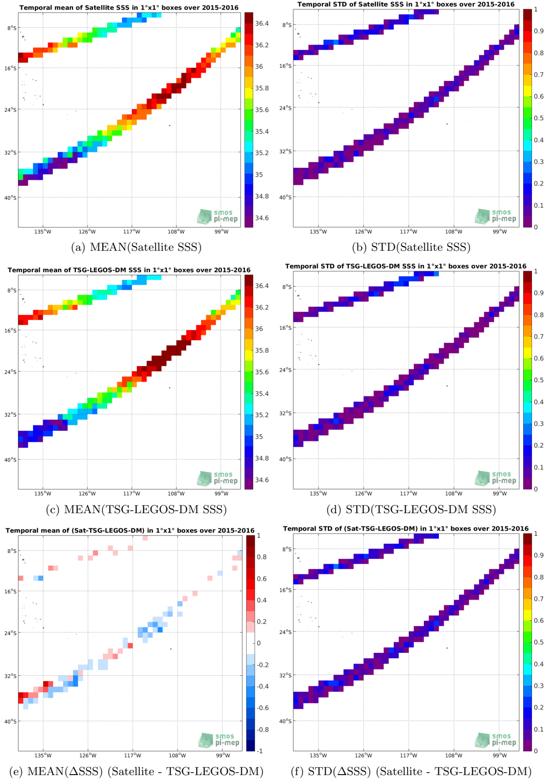
Figure 6: Temporal mean (left) and STD (right) of SSS from SMAP-L3-RSS-V3-8DAY-RUNNING-70KM (top), TSG-LEGOS-DM (middle), and of \Delta SSS (Satellite - TSG-LEGOS-DM). Only match-up pairs are used to generate these maps.
