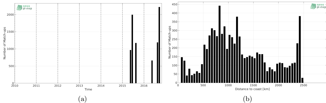
Figure 1: Number of match-ups between TSG-LEGOS-DM and SMAP-L3-RSS-V3-8DAY-RUNNING-70KM SSS as a function of time (a) and as function of the distance to coast (b) over the OTT zone Pi-MEP region and for the full satellite product period.
