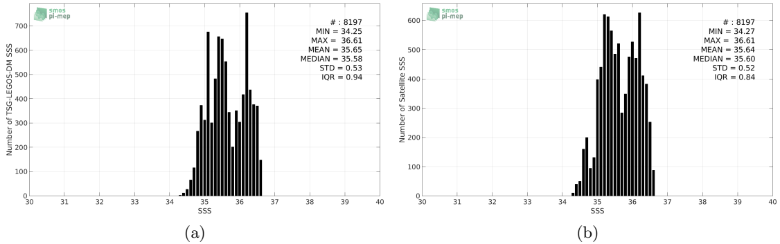
Figure 2: Histograms of SSS from TSG-LEGOS-DM (a) and SMAP-L3-RSS-V3-8DAY-RUNNING-70KM (b) considering all match-up pairs per bins of 0.1 over the OTT zone Pi-MEP region and for the full satellite product period.
