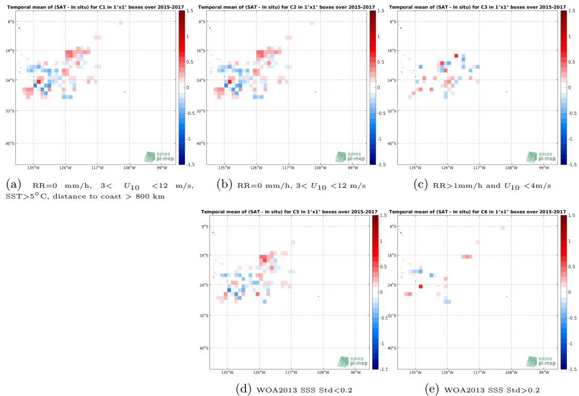
Figure 11: Temporal mean gridded over spatial boxes of size 1^\circ \times 1^\circ of \Delta SSS (SMAP-L3-RSS-V3-8DAY-RUNNING-70KM - Surface drifters) for 5 different subdatasets corresponding to:RR=0 mm/h, 3 < U_{10} < 12 m/s, SST >5^\circ C, distance to coast > 800 km (a), RR=0 mm/h, 3 < U_{10} < 12 m/s (b), RR >1 mm/h and U_{10} < 4 m/s (c), WOA2013 SSS Std <0.2 (d), WOA2013 SSS Std >0.2 (e).
