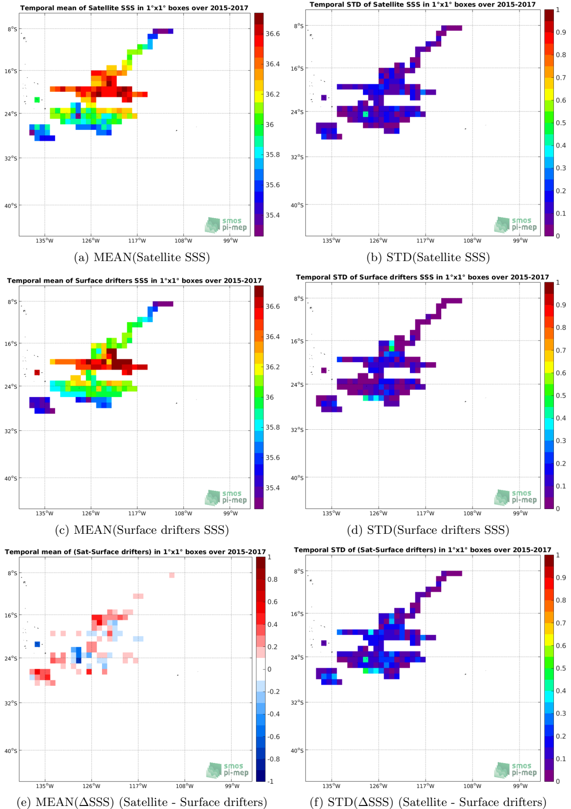
Figure 5: Temporal mean (left) and STD (right) of SSS from SMAP-L3-RSS-V3-8DAY-RUNNING-70KM (top), Surface drifters (middle), and of \Delta SSS (Satellite - Surface drifters). Only match-up pairs are used to generate these maps.
