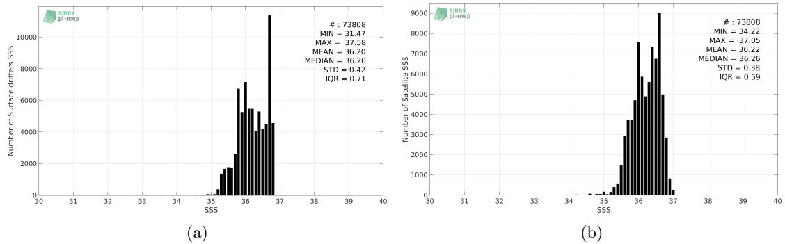
Figure 2: Histograms of SSS from Surface drifters (a) and SMAP-L3-RSS-V3-8DAY-RUNNING-70KM (b) considering all match-up pairs per bins of 0.1 over the OTT zone Pi-MEP region and for the full satellite product period.
