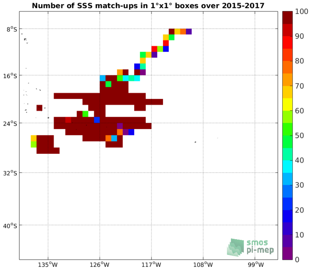
Figure 3: Number of SSS match-ups between Surface drifters SSS and the SMAP-L3-RSS-V3-8DAY-RUNNING-70KM SSS product for the OTT zone Pi-MEP region over 1°x1° boxes and for the full satellite product period.
