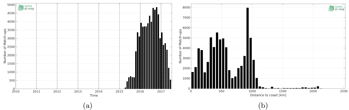
Figure 1: Number of match-ups between Surface drifters and SMAP-L3-RSS-V3-8DAY-RUNNING-70KM SSS as a function of time (a) and as function of the distance to coast (b) over the OTT zone Pi-MEP region and for the full satellite product period.
