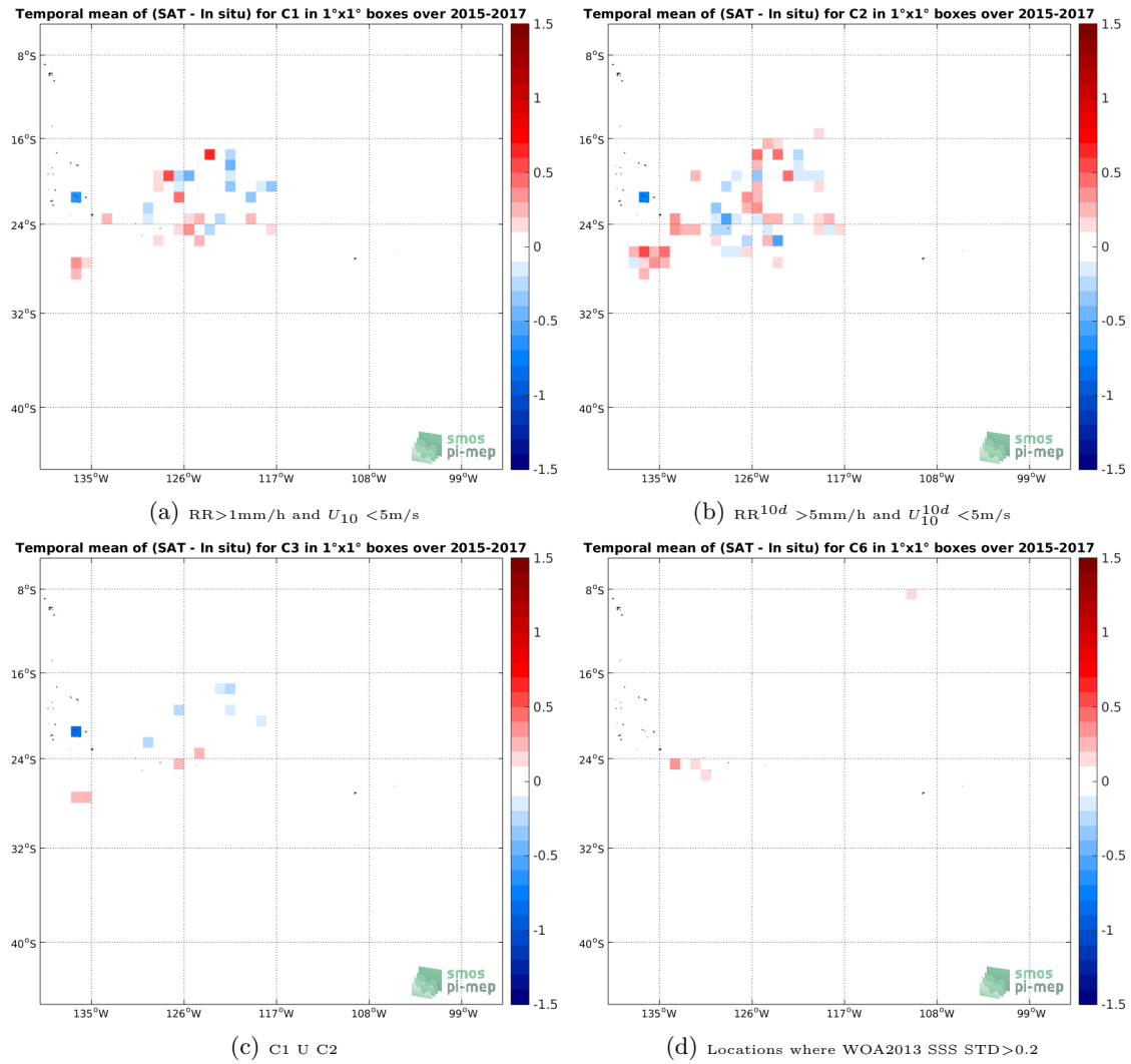
Figure 11: Temporal mean gridded over spatial boxes of size 1^\circ \times 1^\circ of \Delta SSS (SMAP-L3-RSS-V3-8DAY-RUNNING-70KM - Surface drifters) for 4 different subdatasets corresponding to: RR > 1\text{mm/h} and U_{10} < 5\text{m/s} (a), RR^{10d} > 5\text{mm/h} and U_{10}^{10d} < 5\text{m/s} (b), C1 U C2 (c), Locations where WOA2013 SSS STD > 0.2 (d).
