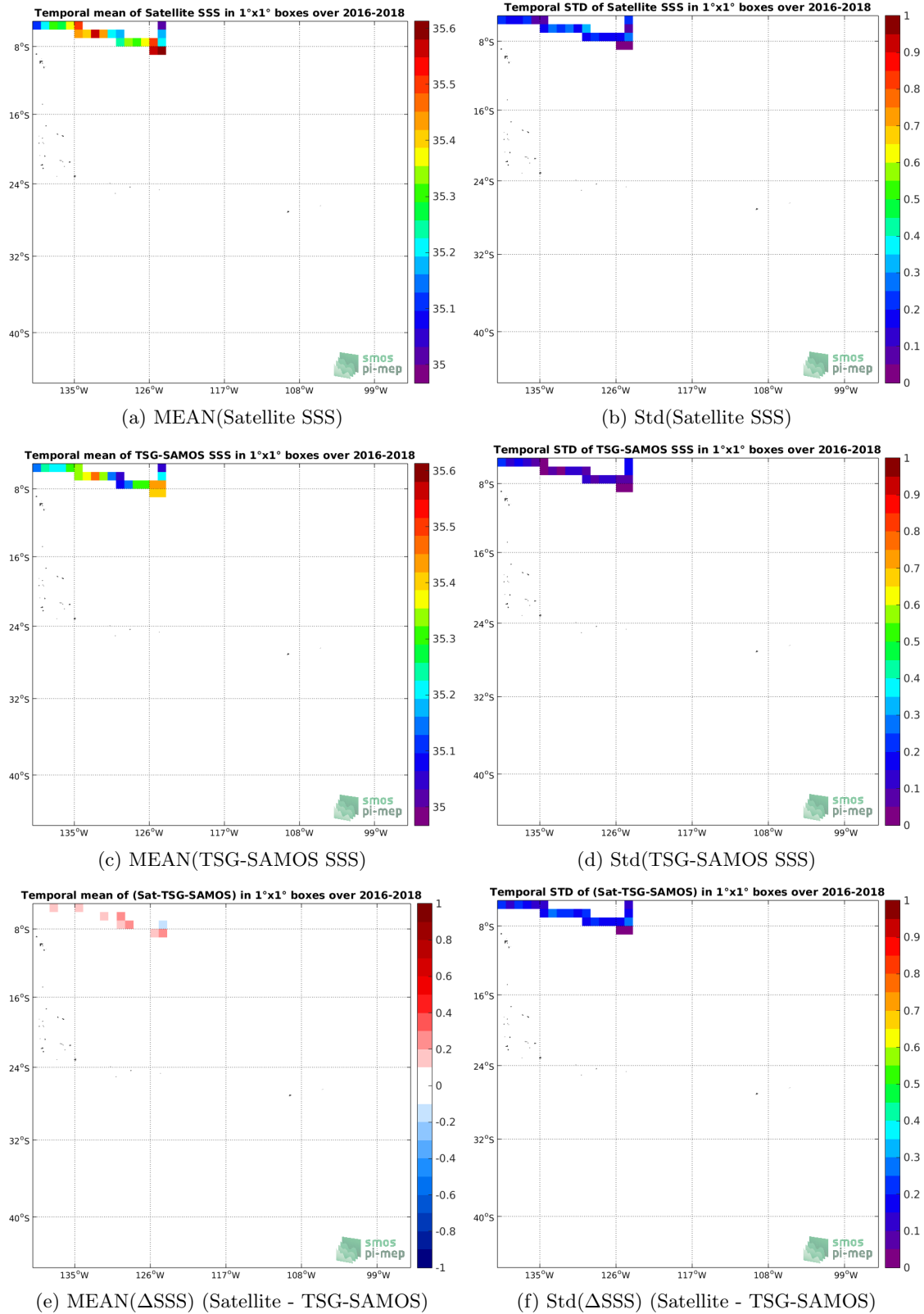
Figure 6: Temporal mean (left) and Std (right) of SSS from SMAP-L3-RSS-V3-8DAY-RUNNING-40KM (top), TSG-SAMOS (middle), and of \Delta SSS (Satellite - TSG-SAMOS). Only match-up pairs are used to generate these maps.
