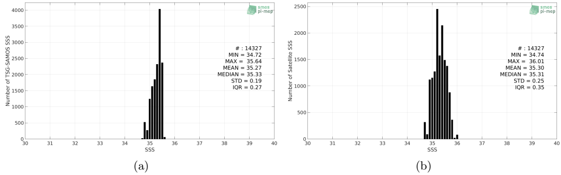
Figure 2: Histograms of SSS from TSG-SAMOS (a) and SMAP-L3-RSS-V3-8DAY-RUNNING-40KM (b) considering all match-up pairs per bins of 0.1 over the OTT zone Pi-MEP region and for the full satellite product period.
