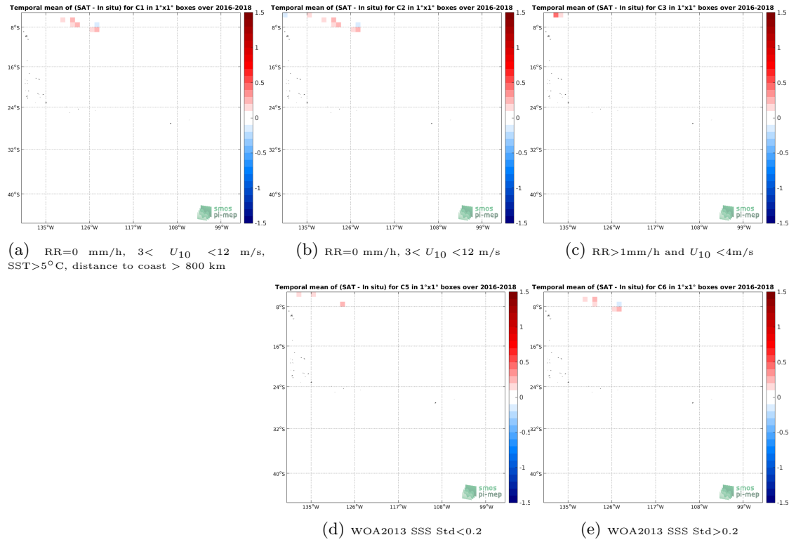
Figure 12: Temporal mean gridded over spatial boxes of size 1^\circ \times 1^\circ of \Delta SSS (SMAP-L3-RSS-V3-8DAY-RUNNING-40KM - TSG-SAMOS) for 5 different subdatasets corresponding to:RR=0 mm/h, 3 < U_{10} < 12 m/s, SST >5^\circ C, distance to coast > 800 km (a), RR=0 mm/h, 3 < U_{10} < 12 m/s (b), RR >1 mm/h and U_{10} < 4 m/s (c), WOA2013 SSS Std <0.2 (d), WOA2013 SSS Std >0.2 (e).
