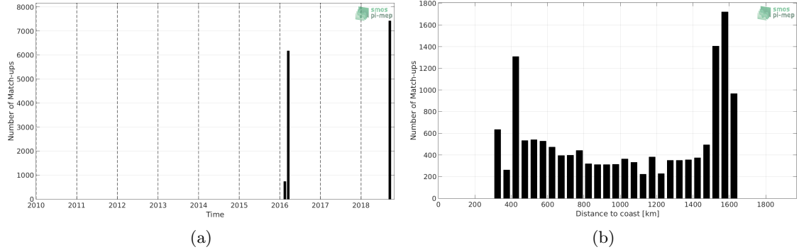
Figure 1: Number of match-ups between TSG-SAMOS and SMAP-L3-RSS-V3-8DAY-RUNNING-40KM SSS as a function of time (a) and as function of the distance to coast (b) over the OTT zone Pi-MEP region and for the full satellite product period.
