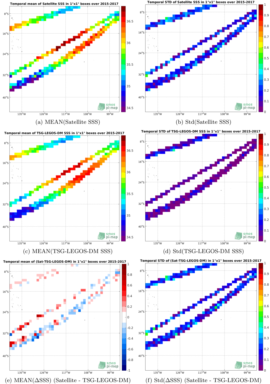
Figure 6: Temporal mean (left) and Std (right) of SSS from SMAP-L3-RSS-V3-8DAY-RUNNING-40KM (top), TSG-LEGOS-DM (middle), and of \Delta SSS (Satellite - TSG-LEGOS-DM). Only match-up pairs are used to generate these maps.
