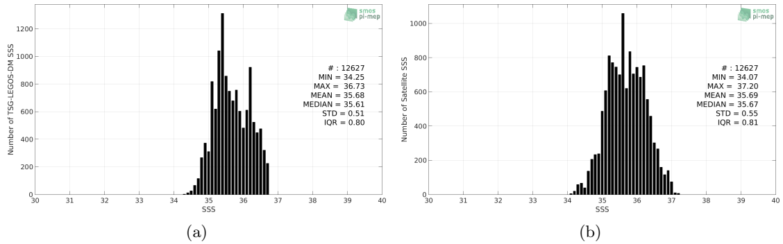
Figure 2: Histograms of SSS from TSG-LEGOS-DM (a) and SMAP-L3-RSS-V3-8DAY-RUNNING-40KM (b) considering all match-up pairs per bins of 0.1 over the OTT zone Pi-MEP region and for the full satellite product period.
