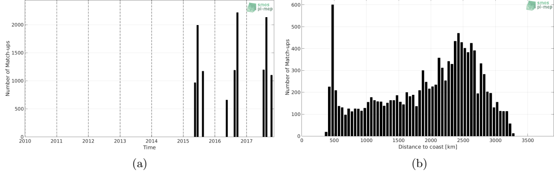
Figure 1: Number of match-ups between TSG-LEGOS-DM and SMAP-L3-RSS-V3-8DAY-RUNNING-40KM SSS as a function of time (a) and as function of the distance to coast (b) over the OTT zone Pi-MEP region and for the full satellite product period.
