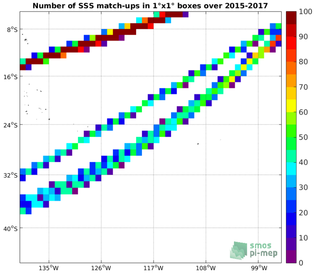
Figure 4: Number of SSS match-ups between TSG-LEGOS-DM SSS and the SMAP-L3-RSS-V3-8DAY-RUNNING-40KM SSS product for the OTT zone Pi-MEP region over 1°x1° boxes and for the full satellite product period.
