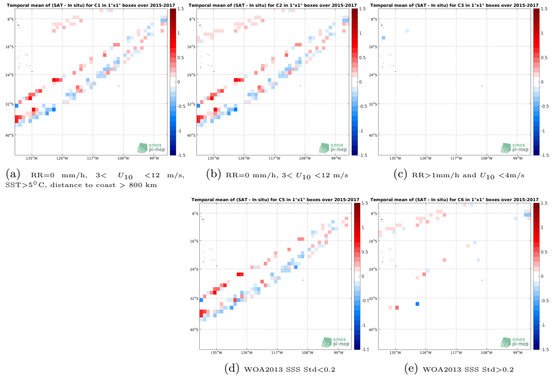
Figure 12: Temporal mean gridded over spatial boxes of size 1^\circ \times 1^\circ of \Delta SSS (SMAP-L3-RSS-V3-8DAY-RUNNING-40KM - TSG-LEGOS-DM) for 5 different subdatasets corresponding to:RR=0 mm/h, 3 < U_{10} < 12 m/s, SST >5^\circ C, distance to coast > 800 km (a), RR=0 mm/h, 3 < U_{10} < 12 m/s (b), RR >1 mm/h and U_{10} < 4 m/s (c), WOA2013 SSS Std <0.2 (d), WOA2013 SSS Std >0.2 (e).
