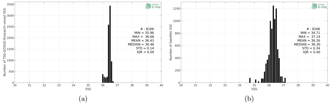
Figure 2: Histograms of SSS from TSG-GOSUD-Research-vessel (a) and SMAP-L3-RSS-V3-8DAY-RUNNING-40KM (b) considering all match-up pairs per bins of 0.1 over the OTT zone Pi-MEP region and for the full satellite product period.
