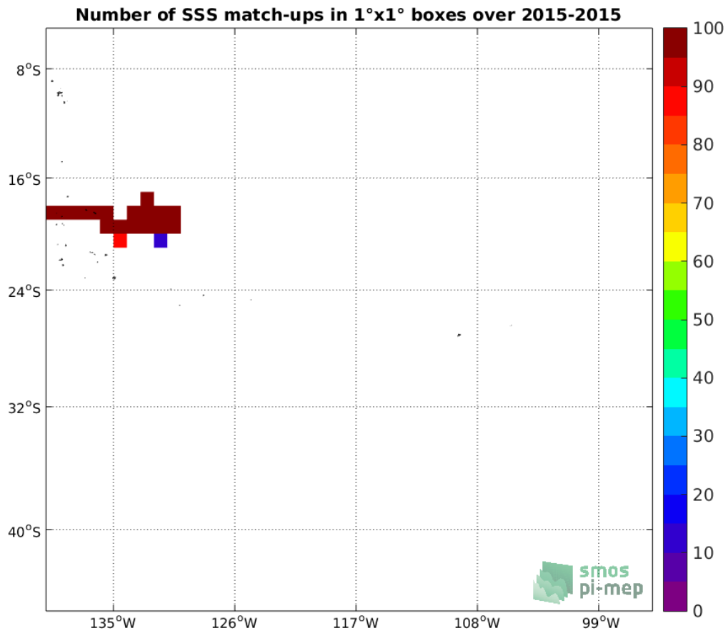
Figure 4: Number of SSS match-ups between TSG-GOSUD-Research-vessel SSS and the SMAP-L3-RSS-V3-8DAY-RUNNING-40KM SSS product for the OTT zone Pi-MEP region over 1°x1° boxes and for the full satellite product period.
