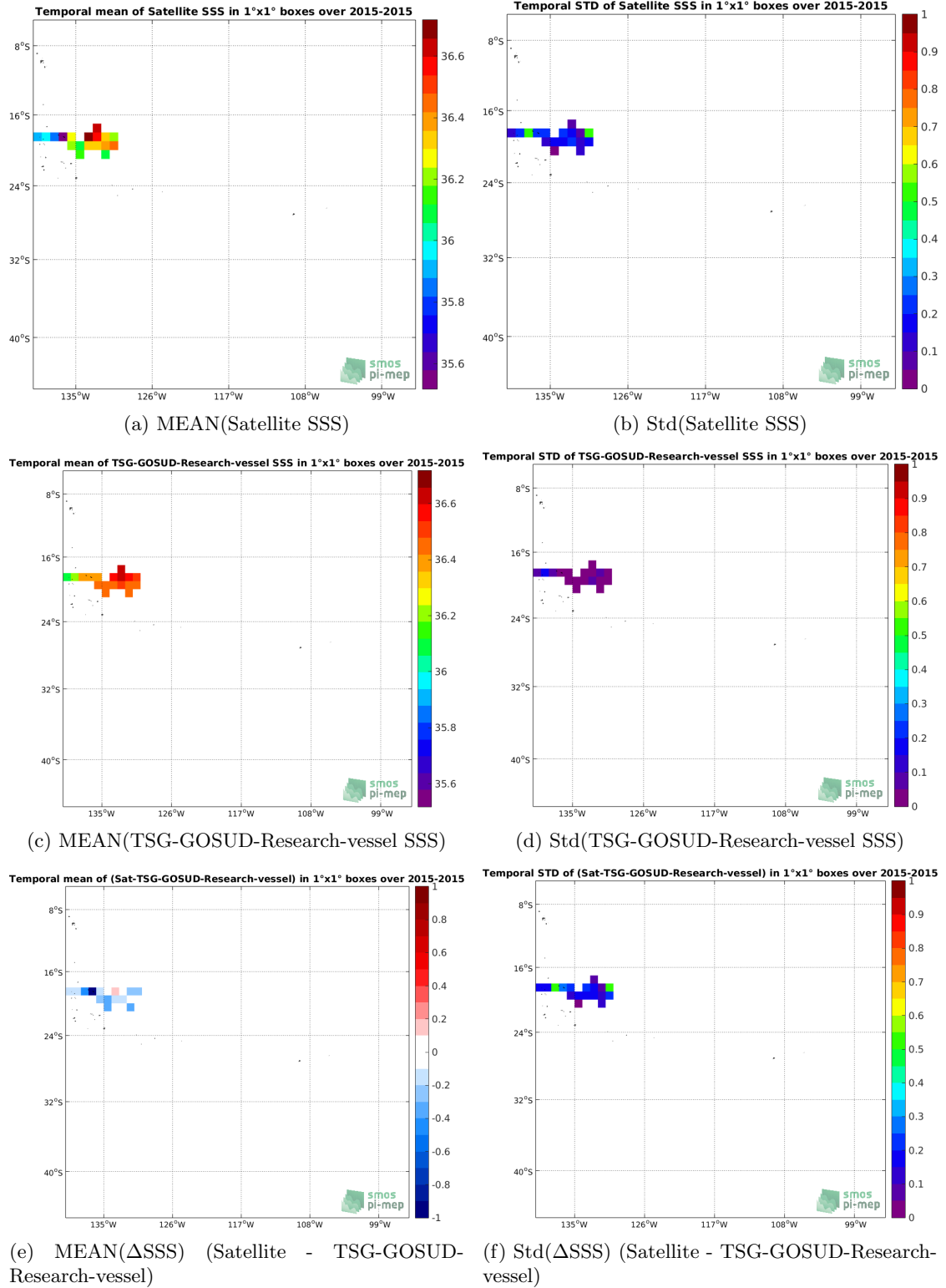
Figure 6: Temporal mean (left) and Std (right) of SSS from SMAP-L3-RSS-V3-8DAY-RUNNING-40KM (top), TSG-GOSUD-Research-vessel (middle), and of \Delta SSS (Satellite - TSG-GOSUD-Research-vessel). Only match-up pairs are used to generate these maps.
