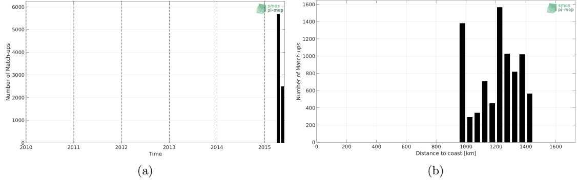
Figure 1: Number of match-ups between TSG-GOSUD-Research-vessel and SMAP-L3-RSS-V3-8DAY-RUNNING-40KM SSS as a function of time (a) and as function of the distance to coast (b) over the OTT zone Pi-MEP region and for the full satellite product period.
