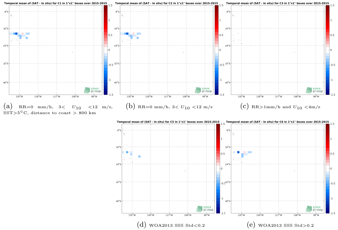
Figure 12: Temporal mean gridded over spatial boxes of size 1^\circ \times 1^\circ of \Delta SSS (SMAP-L3-RSS-V3-8DAY-RUNNING-40KM - TSG-GOSUD-Research-vessel) for 5 different subdatasets corresponding to: RR=0 mm/h, 3 < U_{10} < 12 m/s, SST >5^\circ\text{C} , distance to coast > 800 km (a), RR=0 mm/h, 3 < U_{10} < 12 m/s (b), RR >1 mm/h and U_{10} < 4 m/s (c), WOA2013 SSS Std <0.2 (d), WOA2013 SSS Std >0.2 (e).
