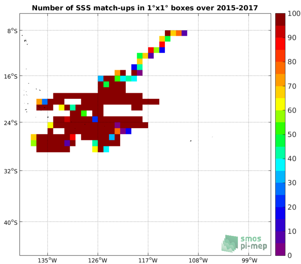
Figure 3: Number of SSS match-ups between Surface drifters SSS and the SMAP-L3-RSS-V3-8DAY-RUNNING-40KM SSS product for the OTT zone Pi-MEP region over 1°x1° boxes and for the full satellite product period.
