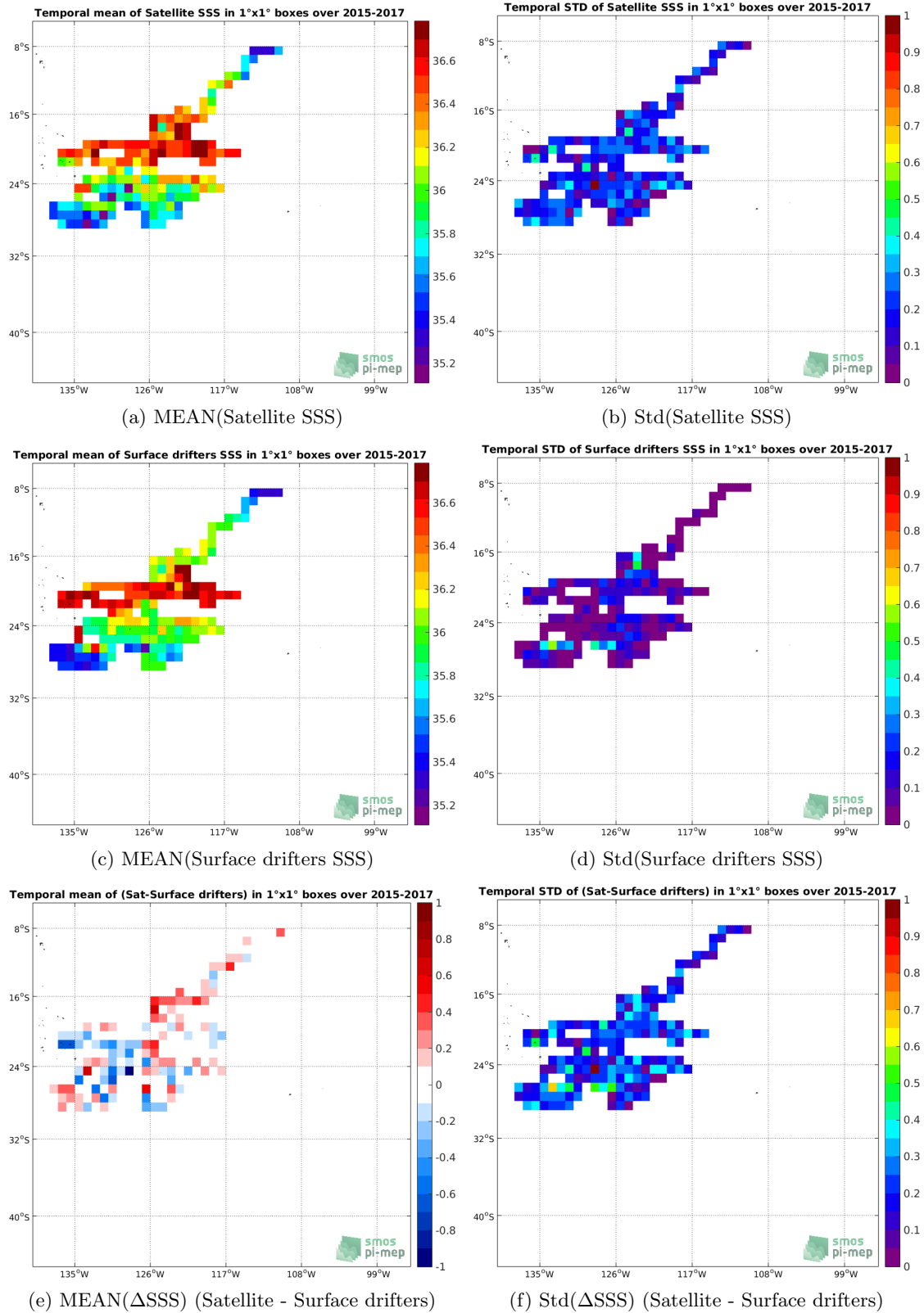
Figure 5: Temporal mean (left) and Std (right) of SSS from SMAP-L3-RSS-V3-8DAY-RUNNING-40KM (top), Surface drifters (middle), and of \Delta SSS (Satellite - Surface drifters). Only match-up pairs are used to generate these maps.
