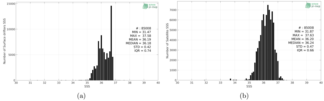
Figure 2: Histograms of SSS from Surface drifters (a) and SMAP-L3-RSS-V3-8DAY-RUNNING-40KM (b) considering all match-up pairs per bins of 0.1 over the OTT zone Pi-MEP region and for the full satellite product period.
