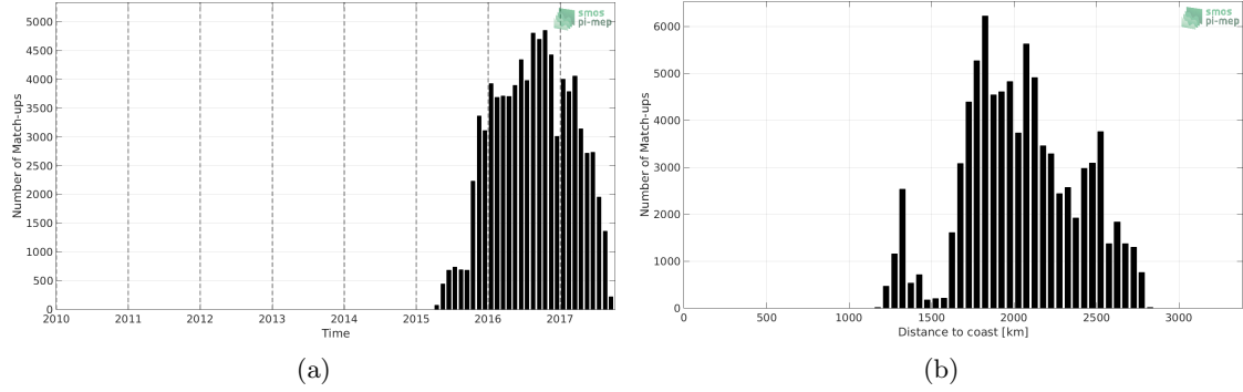
Figure 1: Number of match-ups between Surface drifters and SMAP-L3-RSS-V3-8DAY-RUNNING-40KM SSS as a function of time (a) and as function of the distance to coast (b) over the OTT zone Pi-MEP region and for the full satellite product period.
