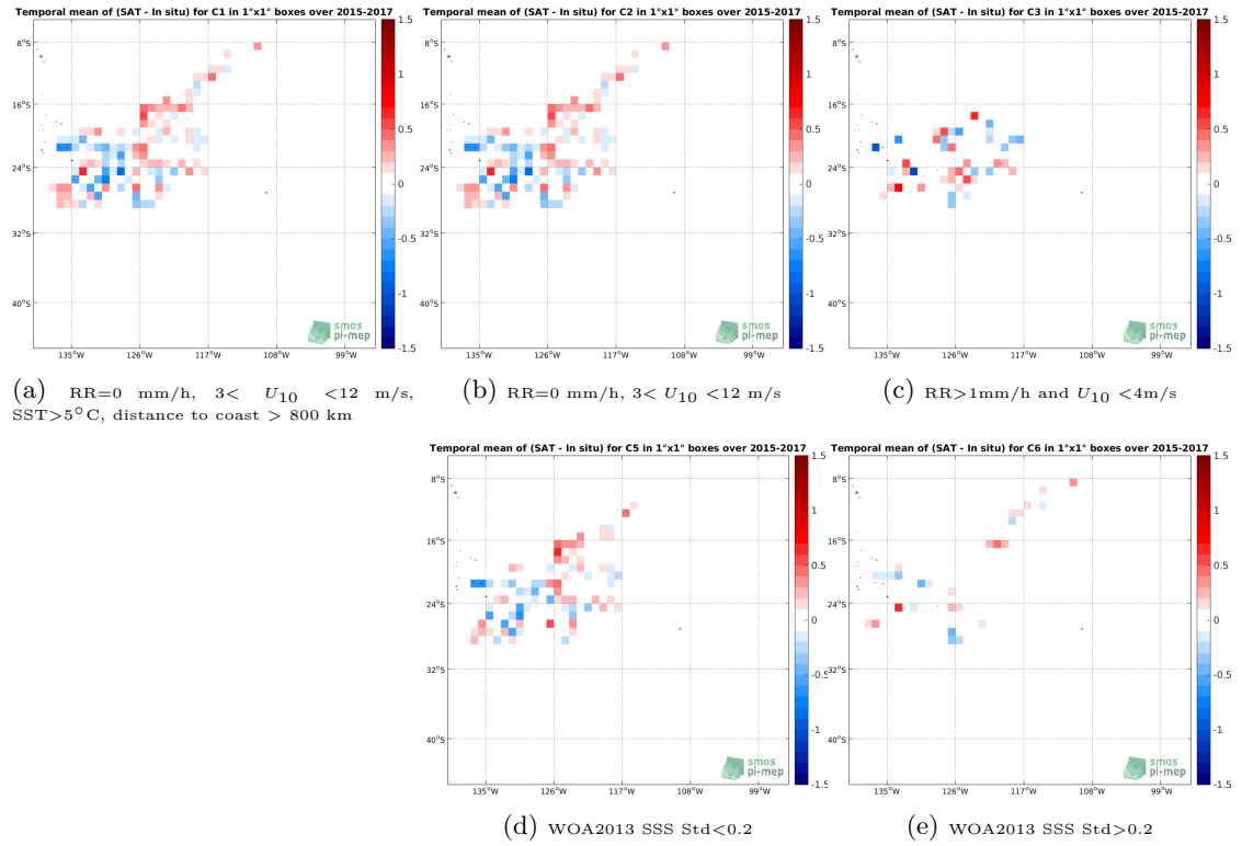
Figure 11: Temporal mean gridded over spatial boxes of size 1^\circ \times 1^\circ of \Delta SSS (SMAP-L3-RSS-V3-8DAY-RUNNING-40KM - Surface drifters) for 5 different subdatasets corresponding to:RR=0 mm/h, 3 < U_{10} < 12 m/s, SST >5^\circ\text{C} , distance to coast > 800 km (a), RR=0 mm/h, 3 < U_{10} < 12 m/s (b), RR >1 mm/h and U_{10} < 4 m/s (c), WOA2013 SSS Std <0.2 (d), WOA2013 SSS Std >0.2 (e).
