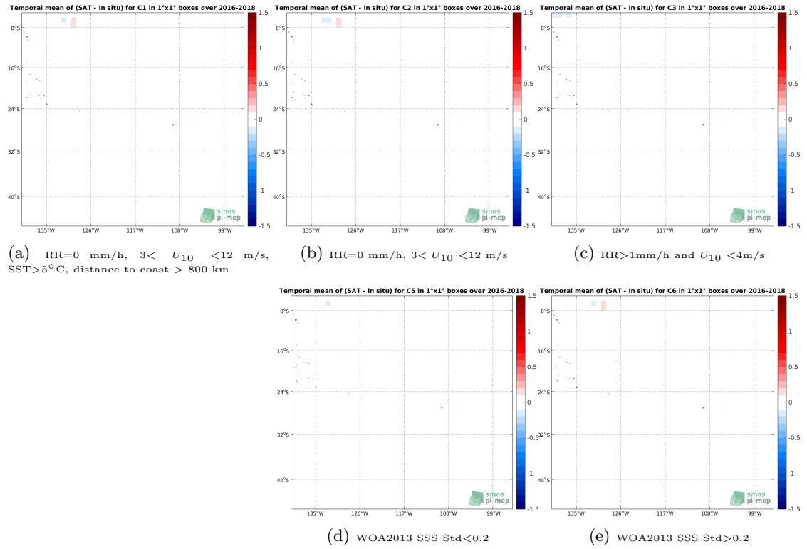
Figure 12: Temporal mean gridded over spatial boxes of size 1^\circ \times 1^\circ of \Delta SSS (SMAP-L3-RSS-V3-MONTHLY-70KM - TSG-SAMOS) for 5 different subdatasets corresponding to:RR=0 mm/h, 3 < U_{10} < 12 m/s, SST >5^\circ C, distance to coast > 800 km (a), RR=0 mm/h, 3 < U_{10} < 12 m/s (b), RR >1 mm/h and U_{10} < 4 m/s (c), WOA2013 SSS Std <0.2 (d), WOA2013 SSS Std >0.2 (e).
