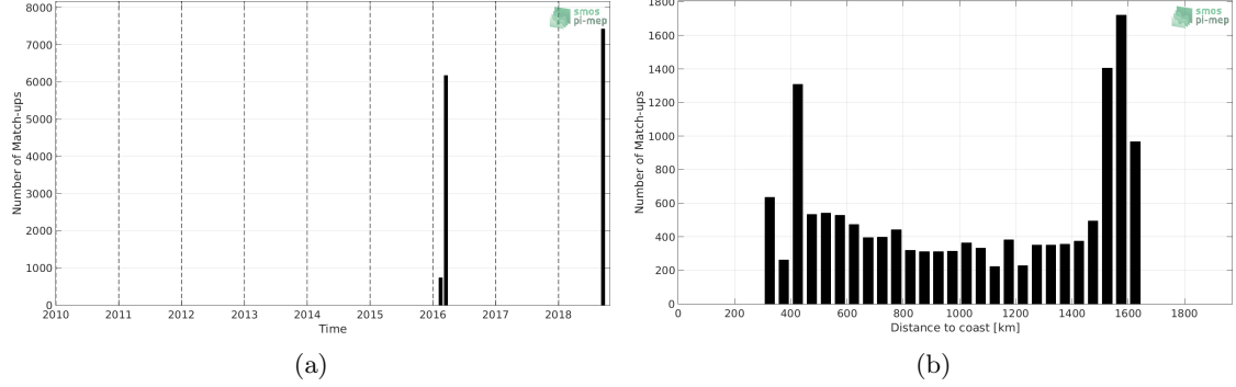
Figure 1: Number of match-ups between TSG-SAMOS and SMAP-L3-RSS-V3-MONTHLY-70KM SSS as a function of time (a) and as function of the distance to coast (b) over the OTT zone Pi-MEP region and for the full satellite product period.
