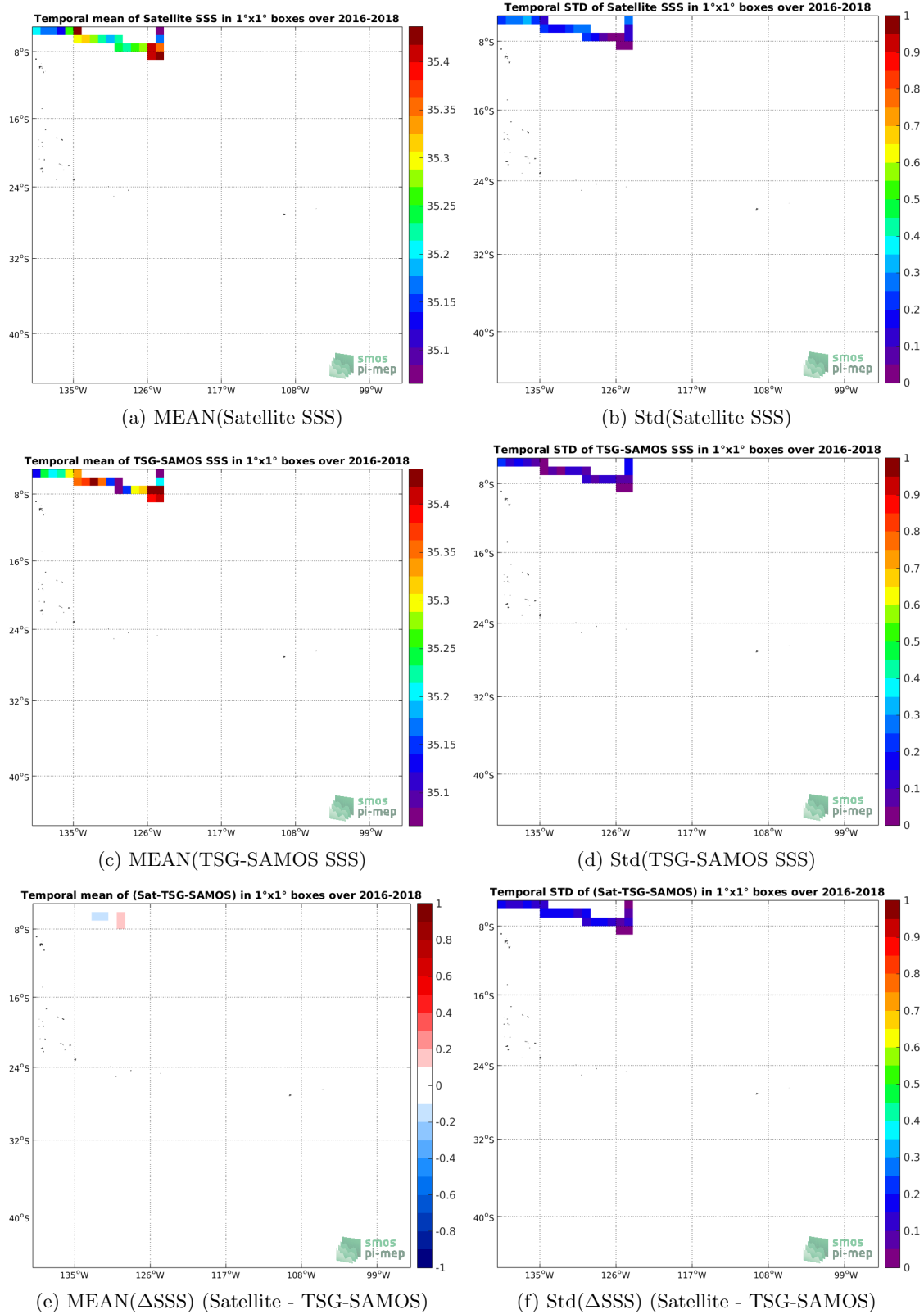
Figure 6: Temporal mean (left) and Std (right) of SSS from SMAP-L3-RSS-V3-MONTHLY-70KM (top), TSG-SAMOS (middle), and of \Delta SSS (Satellite - TSG-SAMOS). Only match-up pairs are used to generate these maps.
