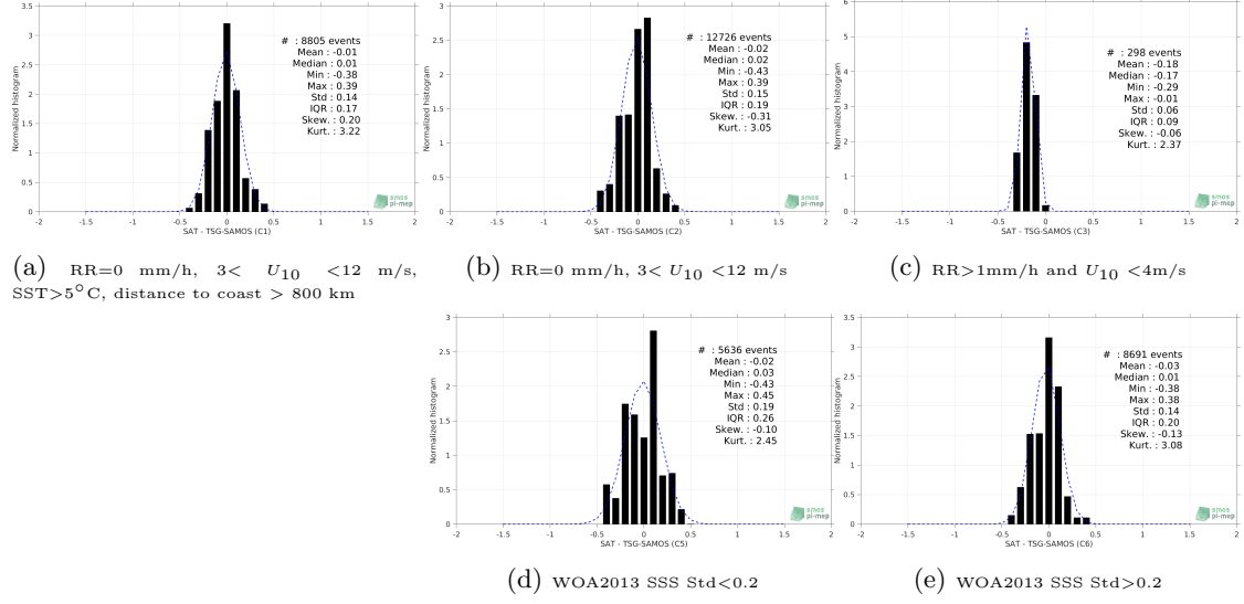
Figure 13: Normalized histogram of \Delta\text{SSS} (SMAP-L3-RSS-V3-MONTHLY-70KM - TSG-SAMOS) for 5 different subdatasets corresponding to: RR=0 mm/h, 3 < U_{10} < 12 m/s, SST > 5^\circ\text{C} , distance to coast > 800 km (a), RR=0 mm/h, 3 < U_{10} < 12 m/s (b), RR > 1 mm/h and U_{10} < 4 m/s (c), WOA2013 SSS Std < 0.2 (d), WOA2013 SSS Std > 0.2 (e).
