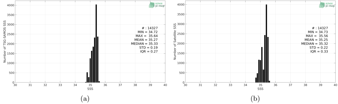
Figure 2: Histograms of SSS from TSG-SAMOS (a) and SMAP-L3-RSS-V3-MONTHLY-70KM (b) considering all match-up pairs per bins of 0.1 over the OTT zone Pi-MEP region and for the full satellite product period.
