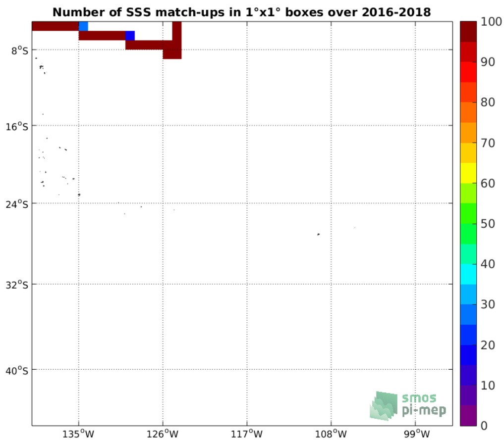
Figure 4: Number of SSS match-ups between TSG-SAMOS SSS and the SMAP-L3-RSS-V3-MONTHLY-70KM SSS product for the OTT zone Pi-MEP region over 1°x1° boxes and for the full satellite product period.
