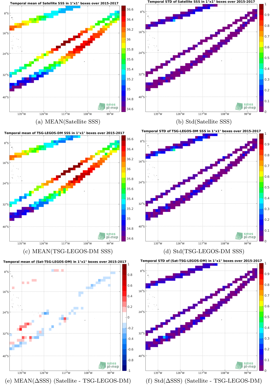
Figure 6: Temporal mean (left) and Std (right) of SSS from SMAP-L3-RSS-V3-MONTHLY-70KM (top), TSG-LEGOS-DM (middle), and of \Delta SSS (Satellite - TSG-LEGOS-DM). Only match-up pairs are used to generate these maps.
