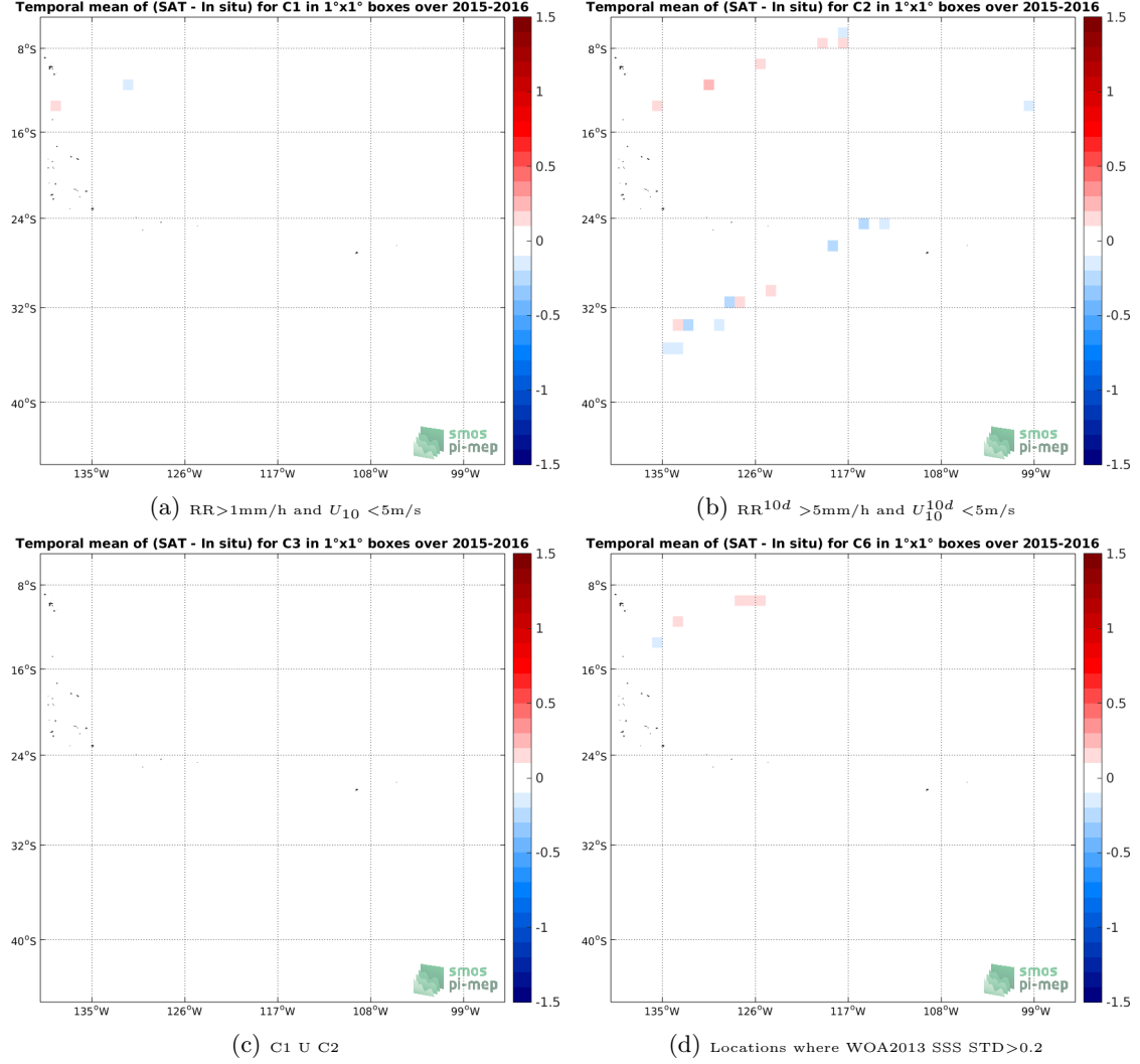
Figure 12: Temporal mean gridded over spatial boxes of size 1^\circ \times 1^\circ of \Delta SSS (SMAP-L3-RSS-V3-MONTHLY-70KM - TSG-LEGOS-DM) for 4 different subdatasets corresponding to: RR > 1\text{mm/h} and U_{10} < 5\text{m/s} (a), RR^{10d} > 5\text{mm/h} and U_{10}^{10d} < 5\text{m/s} (b), C1 U C2 (c), Locations where WOA2013 SSS STD > 0.2 (d).
