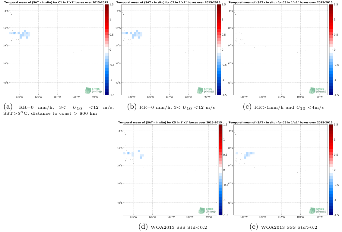
Figure 12: Temporal mean gridded over spatial boxes of size 1^\circ \times 1^\circ of \Delta SSS (SMAP-L3-RSS-V3-MONTHLY-70KM - TSG-GOSUD-Research-vessel) for 5 different subdatasets corresponding to: RR=0 mm/h, 3 < U_{10} < 12 m/s, SST >5^\circ C, distance to coast > 800 km (a), RR=0 mm/h, 3 < U_{10} < 12 m/s (b), RR >1 mm/h and U_{10} < 4 m/s (c), WOA2013 SSS Std <0.2 (d), WOA2013 SSS Std >0.2 (e).
