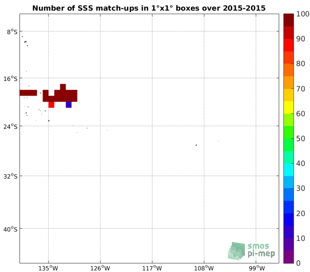
Figure 4: Number of SSS match-ups between TSG-GOSUD-Research-vessel SSS and the SMAP-L3-RSS-V3-MONTHLY-70KM SSS product for the OTT zone Pi-MEP region over 1°x1° boxes and for the full satellite product period.
