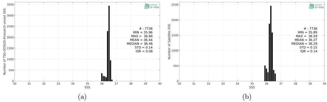
Figure 2: Histograms of SSS from TSG-GOSUD-Research-vessel (a) and SMAP-L3-RSS-V3-MONTHLY-70KM (b) considering all match-up pairs per bins of 0.1 over the OTT zone Pi-MEP region and for the full satellite product period.
