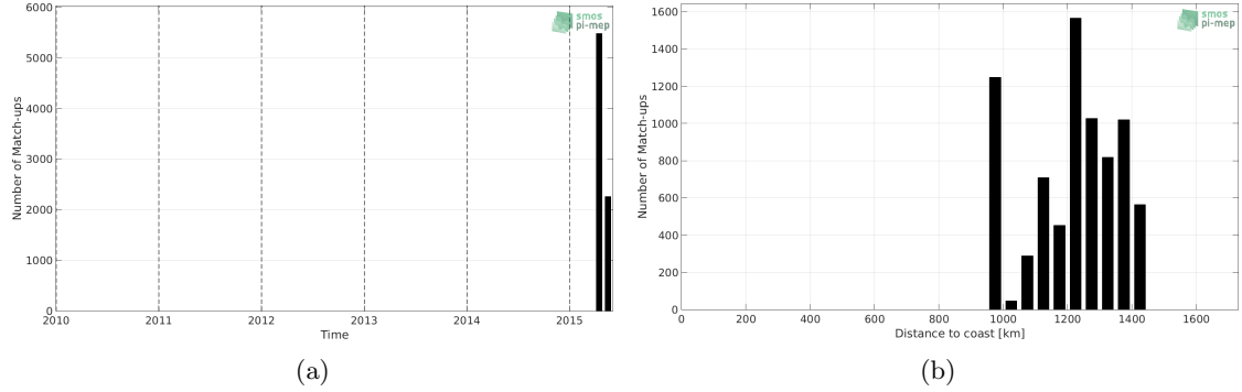
Figure 1: Number of match-ups between TSG-GOSUD-Research-vessel and SMAP-L3-RSS-V3-MONTHLY-70KM SSS as a function of time (a) and as function of the distance to coast (b) over the OTT zone Pi-MEP region and for the full satellite product period.
