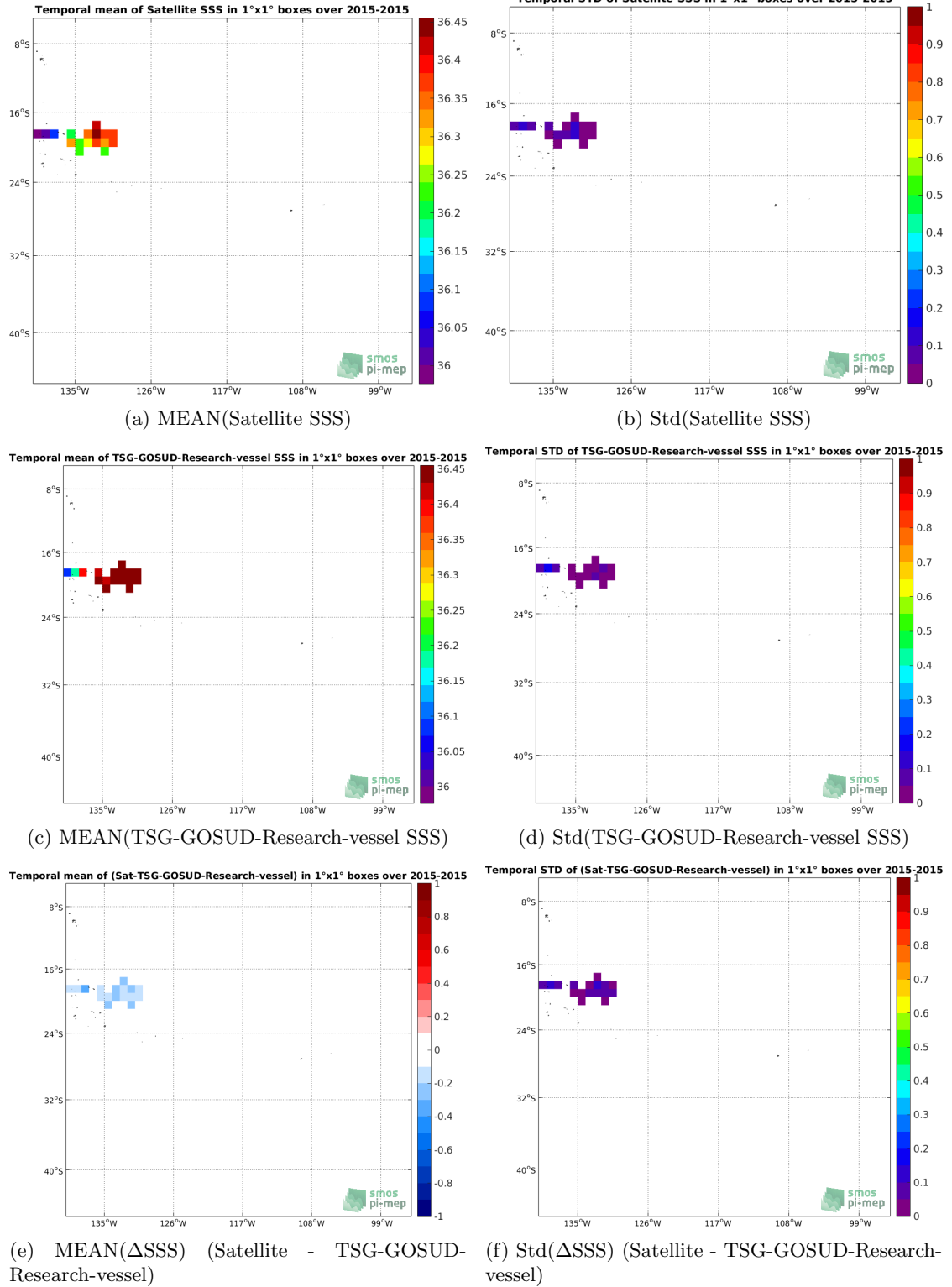
Figure 6: Temporal mean (left) and Std (right) of SSS from SMAP-L3-RSS-V3-MONTHLY-70KM (top), TSG-GOSUD-Research-vessel (middle), and of \Delta SSS (Satellite - TSG-GOSUD-Research-vessel). Only match-up pairs are used to generate these maps.
