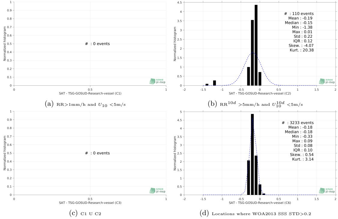
Figure 13: Normalized histogram of \Delta\text{SSS} (SMAP-L3-RSS-V3-MONTHLY-70KM - TSG-GOSUD-Research-vessel) for 6 different subdatasets corresponding to: RR > 1\text{mm/h} and U_{10} < 5\text{m/s} (a), RR^{10d} > 5\text{mm/h} and U_{10}^{10d} < 5\text{m/s} (b), C1 \cup C2 (c), Locations where WOA2013 SSS STD > 0.2 (d).
