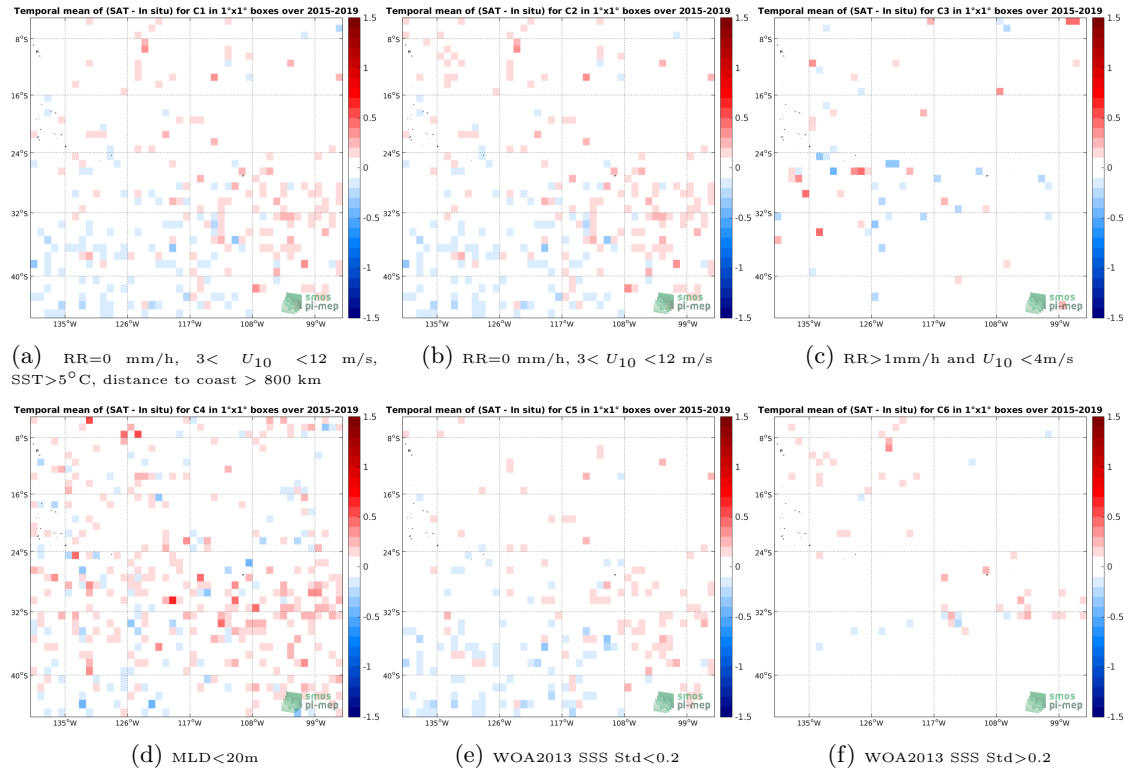
Figure 12: Temporal mean gridded over spatial boxes of size 1^\circ \times 1^\circ of \Delta SSS (SMAP-L3-RSS-V3-MONTHLY-70KM - Argo) for 6 different subdatasets corresponding to:RR=0 mm/h, 3 < U_{10} < 12 m/s, SST >5^\circ C, distance to coast > 800 km (a), RR=0 mm/h, 3 < U_{10} < 12 m/s (b), RR >1 mm/h and U_{10} < 4 m/s (c),MLD <20 m (d),WOA2013 SSS Std <0.2 (e),WOA2013 SSS Std >0.2 (f).
