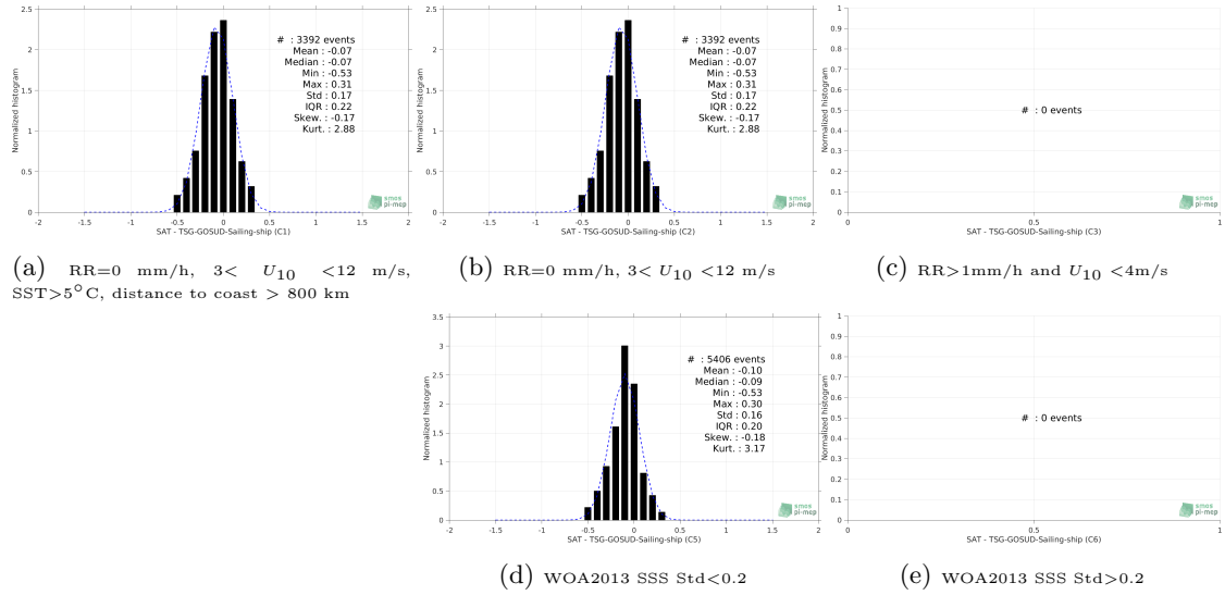
Figure 13: Normalized histogram of \Delta SSS (SMAP-L3-RSS-V3-MONTHLY-0.25DEG-40KM - TSG-GOSUD-Sailing-ship) for 5 different subdatasets corresponding to: RR=0 mm/h, 3 < U_{10} < 12 m/s, SST > 5°C, distance to coast > 800 km (a), RR=0 mm/h, 3 < U_{10} < 12 m/s (b), RR > 1mm/h and U_{10} < 4 m/s (c), WOA2013 SSS Std < 0.2 (d), WOA2013 SSS Std > 0.2 (e).
