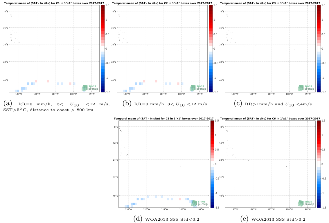
Figure 12: Temporal mean gridded over spatial boxes of size 1^\circ \times 1^\circ of \Delta SSS (SMAP-L3-RSS-V3-MONTHLY-0.25DEG-40KM - TSG-GOSUD-Sailing-ship) for 5 different subdatasets corresponding to:RR=0 mm/h, 3 < U_{10} < 12 m/s, SST >5^\circ C, distance to coast > 800 km (a), RR=0 mm/h, 3 < U_{10} < 12 m/s (b), RR >1 mm/h and U_{10} < 4 m/s (c), WOA2013 SSS Std <0.2 (d), WOA2013 SSS Std >0.2 (e).
