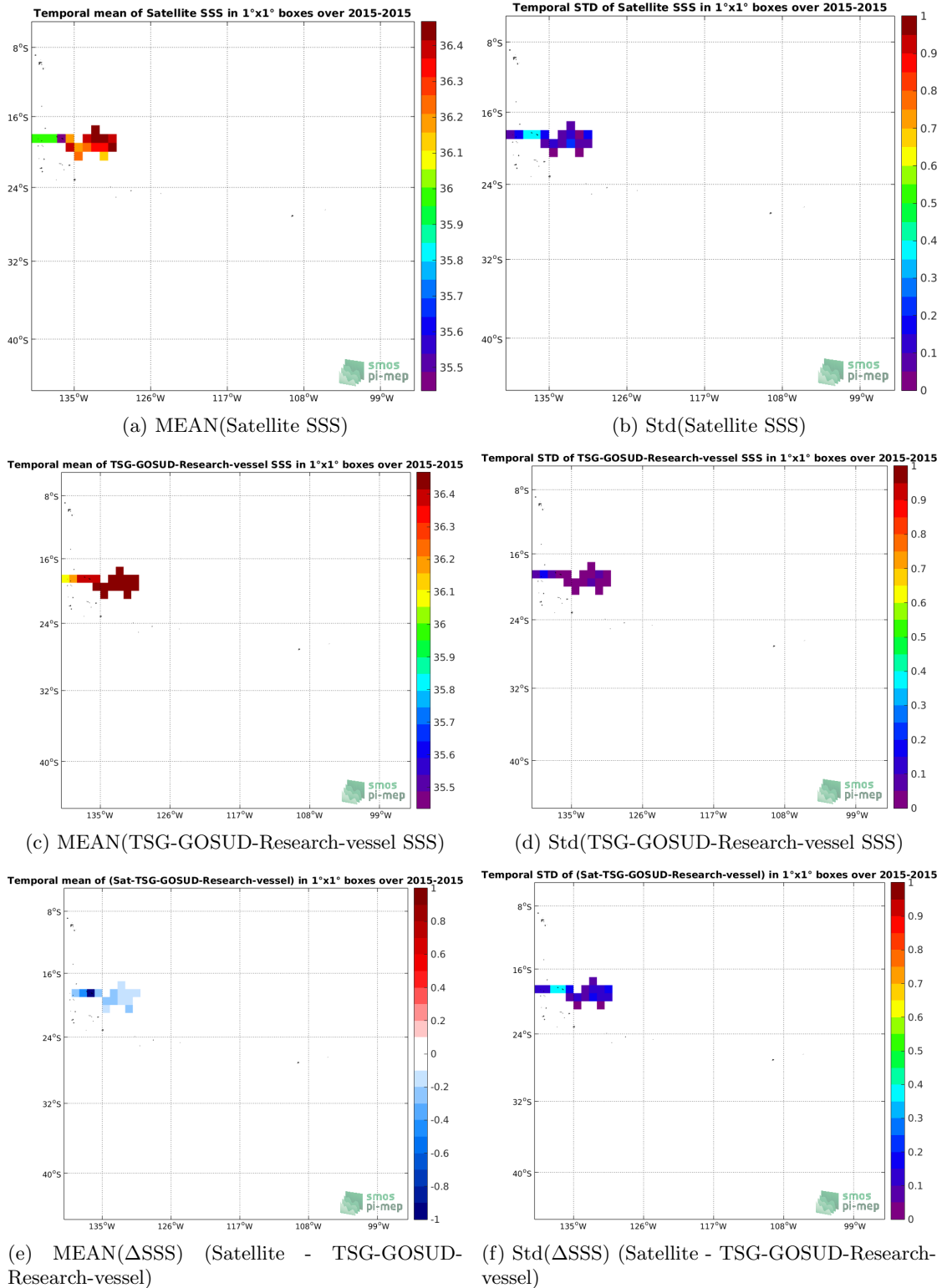
Figure 6: Temporal mean (left) and Std (right) of SSS from SMAP-L3-RSS-V3-MONTHLY-0.25DEG-40KM (top), TSG-GOSUD-Research-vessel (middle), and of \Delta SSS (Satellite - TSG-GOSUD-Research-vessel). Only match-up pairs are used to generate these maps.
