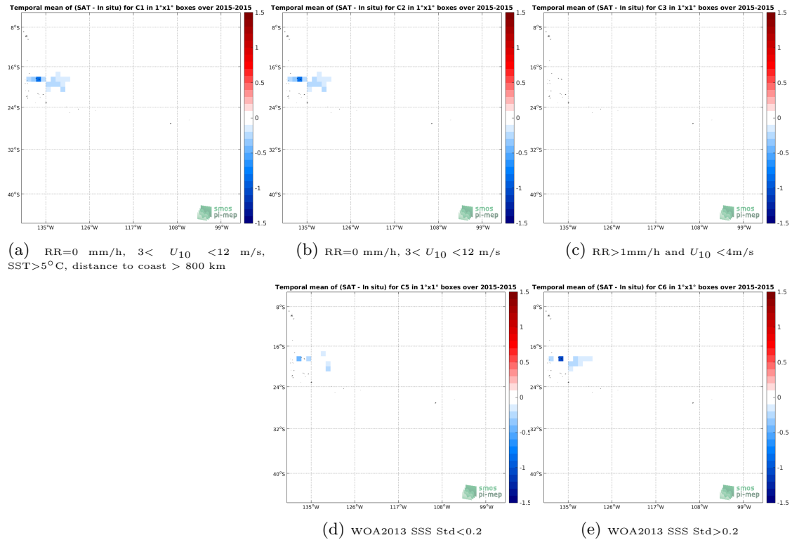
Figure 12: Temporal mean gridded over spatial boxes of size 1^\circ \times 1^\circ of \Delta SSS (SMAP-L3-RSS-V3-MONTHLY-0.25DEG-40KM - TSG-GOSUD-Research-vessel) for 5 different subdatasets corresponding to:RR=0 mm/h, 3 < U_{10} < 12 m/s, SST >5^\circ C, distance to coast > 800 km (a), RR=0 mm/h, 3 < U_{10} < 12 m/s (b), RR >1 mm/h and U_{10} < 4 m/s (c), WOA2013 SSS Std <0.2 (d), WOA2013 SSS Std >0.2 (e).
