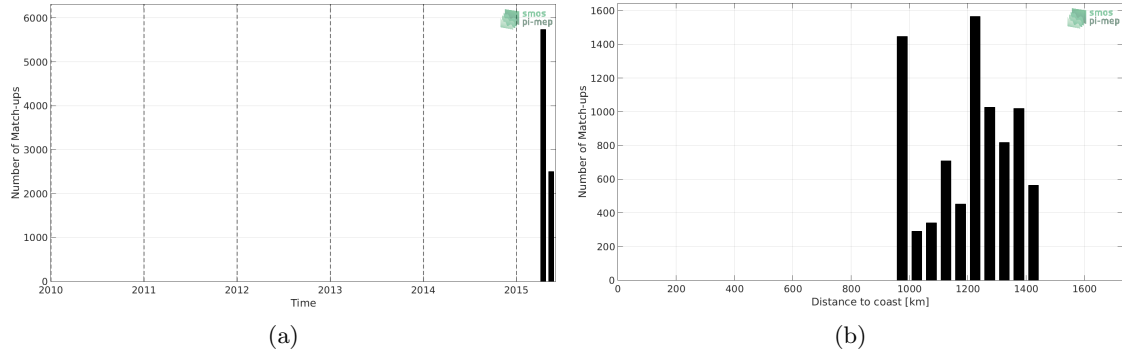
Figure 1: Number of match-ups between TSG-GOSUD-Research-vessel and SMAP-L3-RSS-V3-MONTHLY-0.25DEG-40KM SSS as a function of time (a) and as function of the distance to coast (b) over the OTT zone Pi-MEP region and for the full satellite product period.
