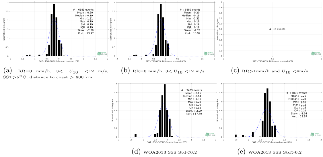
Figure 13: Normalized histogram of \Delta SSS (SMAP-L3-RSS-V3-MONTHLY-0.25DEG-40KM - TSG-GOSUD-Research-vessel) for 5 different subdatasets corresponding to: RR=0 mm/h, 3 < U_{10} < 12 m/s, SST>5°C, distance to coast > 800 km (a), RR=0 mm/h, 3 < U_{10} < 12 m/s (b), RR>1mm/h and U_{10} < 4 m/s (c), WOA2013 SSS Std<0.2 (d), WOA2013 SSS Std>0.2 (e).
