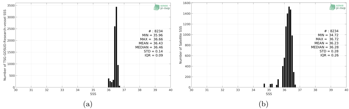
Figure 2: Histograms of SSS from TSG-GOSUD-Research-vessel (a) and SMAP-L3-RSS-V3-MONTHLY-0.25DEG-40KM (b) considering all match-up pairs per bins of 0.1 over the OTT zone Pi-MEP region and for the full satellite product period.
