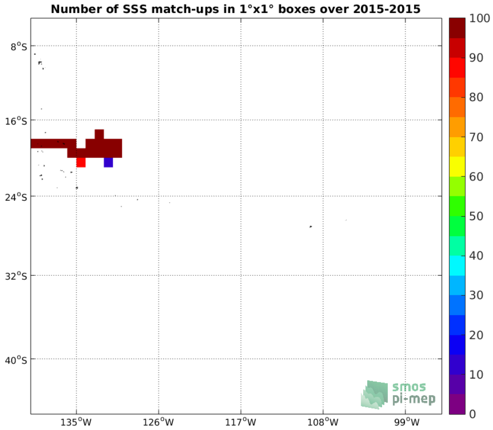
Figure 4: Number of SSS match-ups between TSG-GOSUD-Research-vessel SSS and the SMAP-L3-RSS-V3-MONTHLY-0.25DEG-40KM SSS product for the OTT zone Pi-MEP region over 1°x1° boxes and for the full satellite product period.
