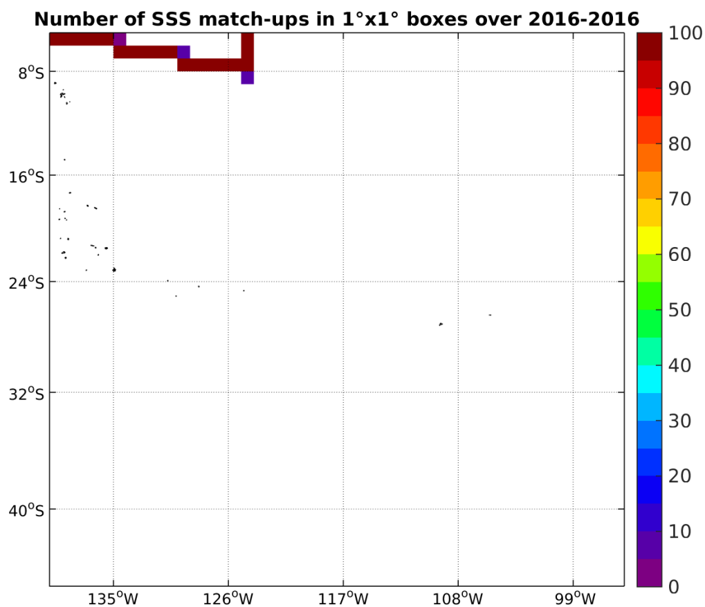
Figure 4: Number of SSS match-ups between TSG-SAMOS SSS and the SMAP-L3-RSS-V2-8DAY-RUNNING-40KM SSS product for the OTT zone Pi-MEP region over 1°x1° boxes and for the full satellite product period.
