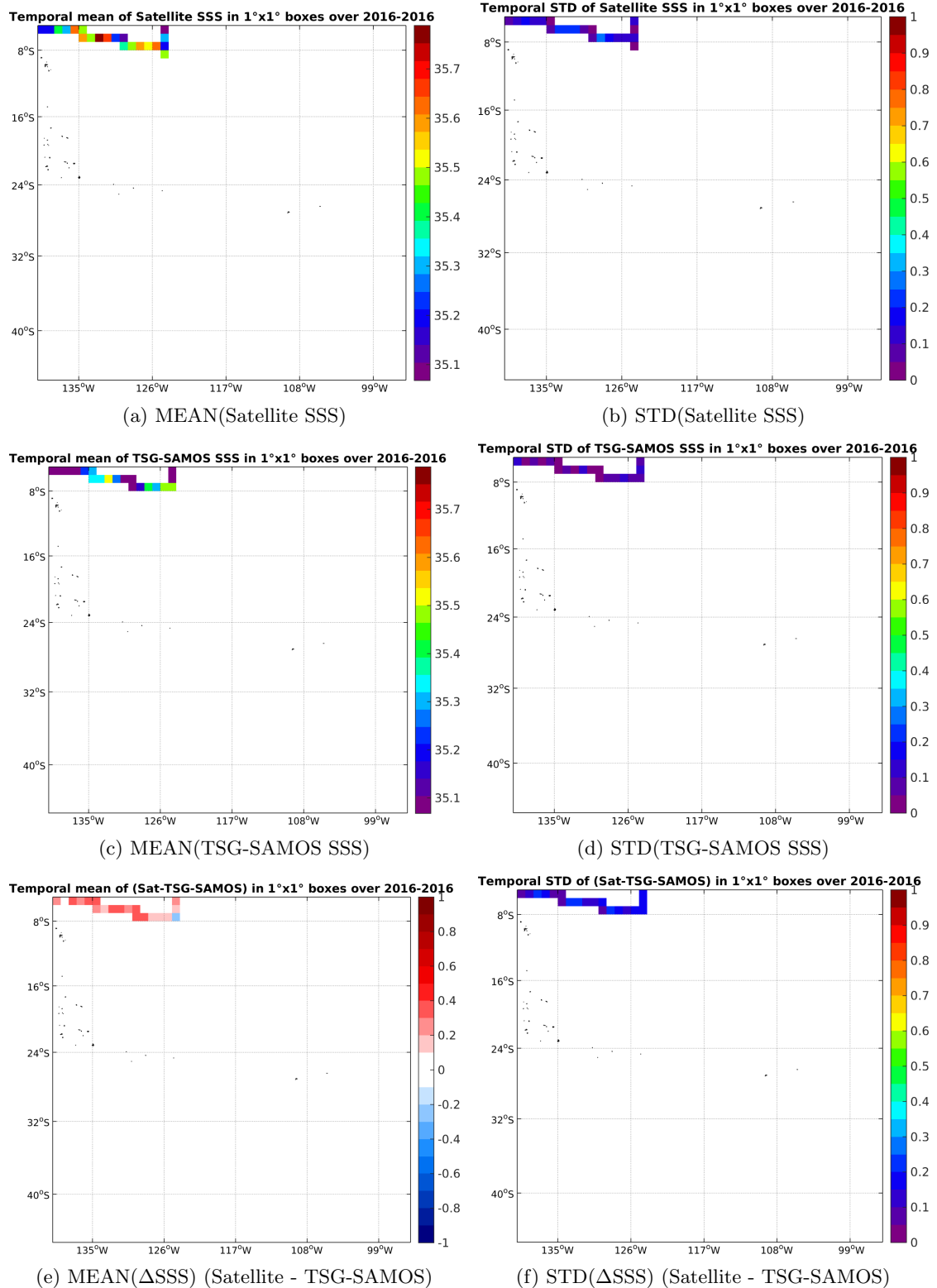
Figure 6: Temporal mean (left) and STD (right) of SSS from SMAP-L3-RSS-V2-8DAY-RUNNING-40KM (top), TSG-SAMOS (middle), and of \Delta SSS (Satellite - TSG-SAMOS). Only match-up pairs are used to generate these maps.
