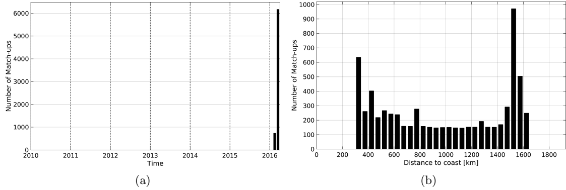
Figure 1: Number of match-ups between TSG-SAMOS and SMAP-L3-RSS-V2-8DAY-RUNNING-40KM SSS as a function of time (a) and as function of the distance to coast (b) over the OTT zone Pi-MEP region and for the full satellite product period.
