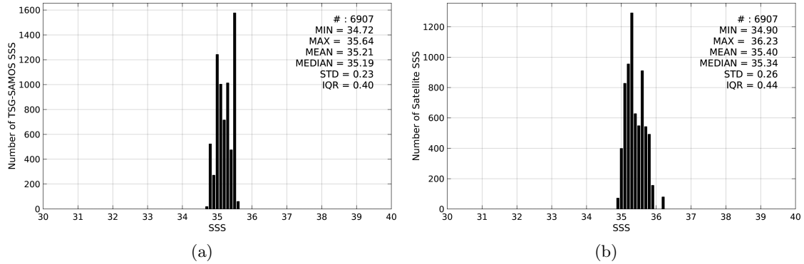
Figure 2: Histograms of SSS from TSG-SAMOS (a) and SMAP-L3-RSS-V2-8DAY-RUNNING-40KM (b) considering all match-up pairs per bins of 0.1 over the OTT zone Pi-MEP region and for the full satellite product period.
