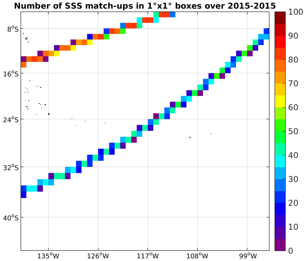
Figure 4: Number of SSS match-ups between TSG-LEGOS-DM SSS and the SMAP-L3-RSS-V2-8DAY-RUNNING-40KM SSS product for the OTT zone Pi-MEP region over 1°x1° boxes and for the full satellite product period.
