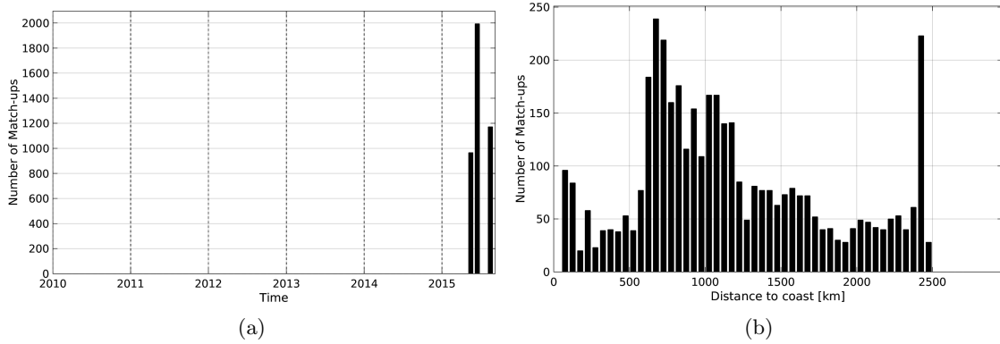
Figure 1: Number of match-ups between TSG-LEGOS-DM and SMAP-L3-RSS-V2-8DAY-RUNNING-40KM SSS as a function of time (a) and as function of the distance to coast (b) over the OTT zone Pi-MEP region and for the full satellite product period.
