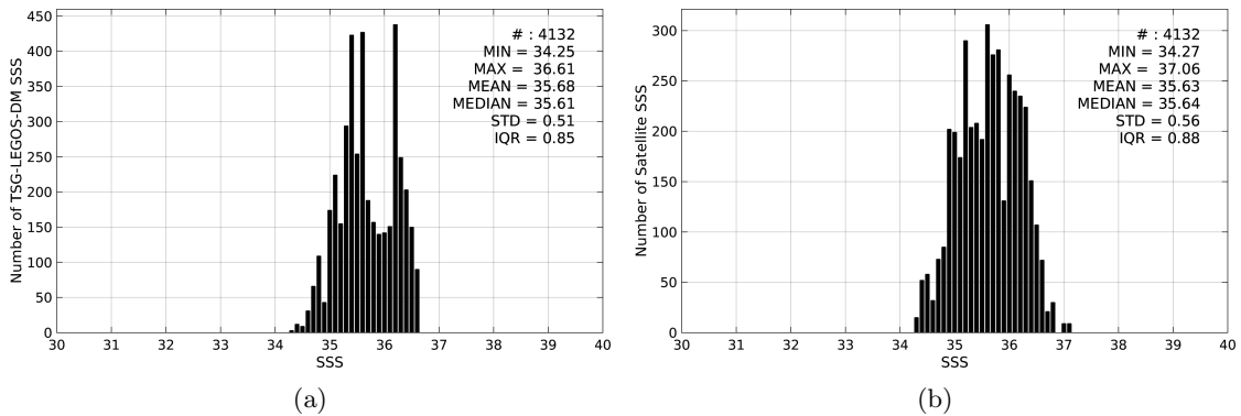
Figure 2: Histograms of SSS from TSG-LEGOS-DM (a) and SMAP-L3-RSS-V2-8DAY-RUNNING-40KM (b) considering all match-up pairs per bins of 0.1 over the OTT zone Pi-MEP region and for the full satellite product period.
