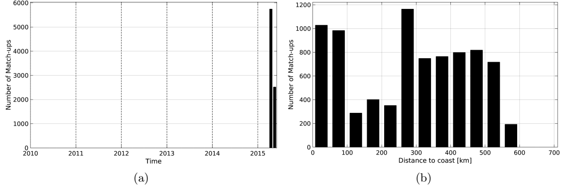
Figure 1: Number of match-ups between TSG-GOSUD-Research-vessel and SMAP-L3-RSS-V2-8DAY-RUNNING-40KM SSS as a function of time (a) and as function of the distance to coast (b) over the OTT zone Pi-MEP region and for the full satellite product period.
