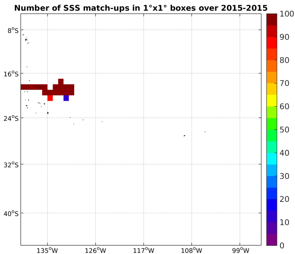
Figure 4: Number of SSS match-ups between TSG-GOSUD-Research-vessel SSS and the SMAP-L3-RSS-V2-8DAY-RUNNING-40KM SSS product for the OTT zone Pi-MEP region over 1°x1° boxes and for the full satellite product period.
