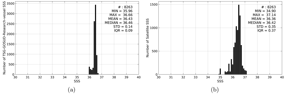
Figure 2: Histograms of SSS from TSG-GOSUD-Research-vessel (a) and SMAP-L3-RSS-V2-8DAY-RUNNING-40KM (b) considering all match-up pairs per bins of 0.1 over the OTT zone Pi-MEP region and for the full satellite product period.
