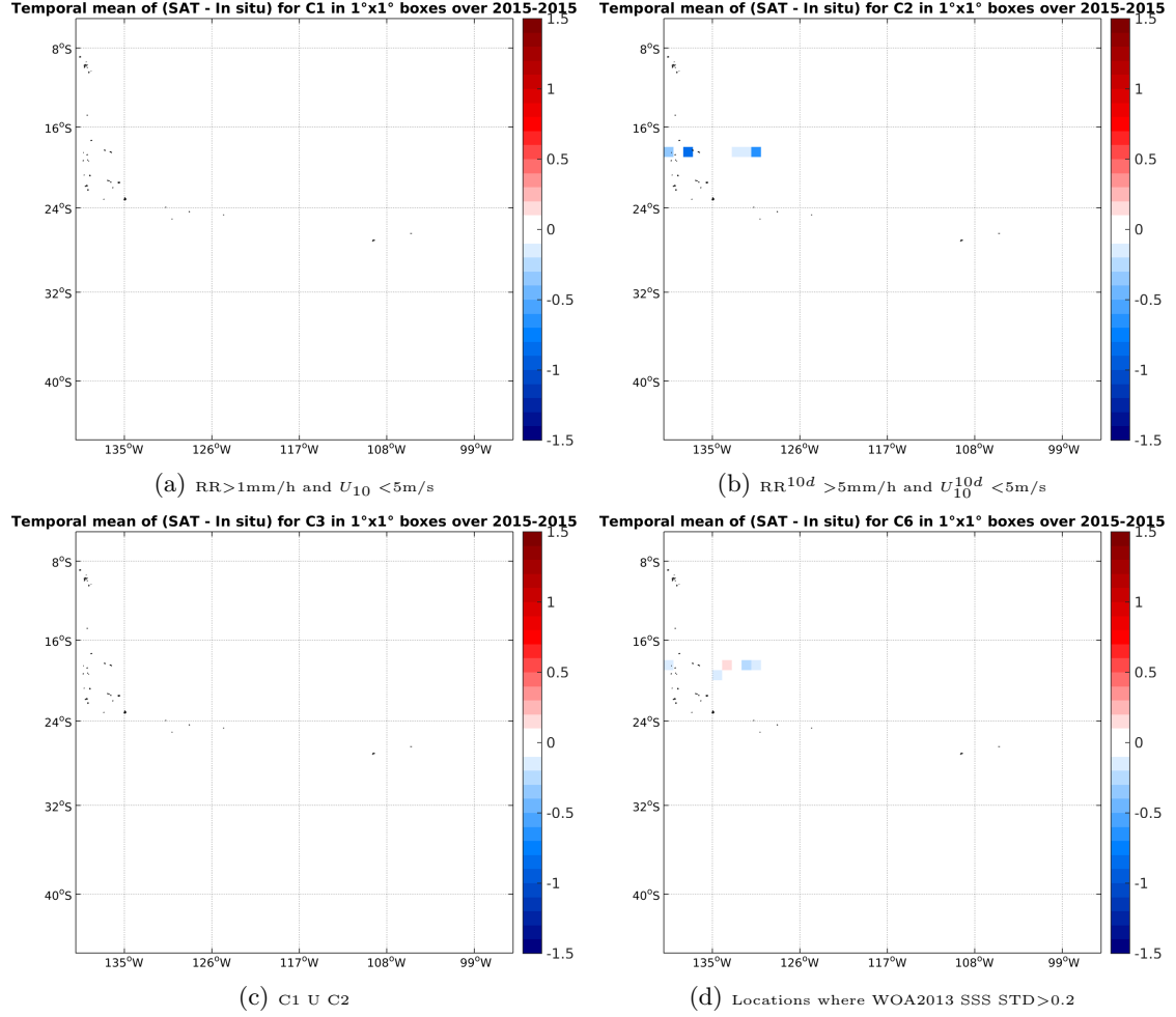
Figure 12: Temporal mean gridded over spatial boxes of size 1^\circ \times 1^\circ of \Delta SSS (SMAP-L3-RSS-V2-8DAY-RUNNING-40KM - TSG-GOSUD-Research-vessel) for 4 different subdatasets corresponding to: RR > 1\text{mm/h} and U_{10} < 5\text{m/s} (a), RR^{10d} > 5\text{mm/h} and U_{10}^{10d} < 5\text{m/s} (b), C1 U C2 (c), Locations where WOA2013 SSS STD > 0.2 (d).
