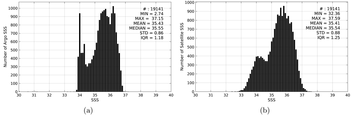
Figure 2: Histograms of SSS from Argo (a) and SMAP-L3-RSS-V2-8DAY-RUNNING-40KM (b) considering all match-up pairs per bins of 0.1 over the OTT zone Pi-MEP region and for the full satellite product period.
