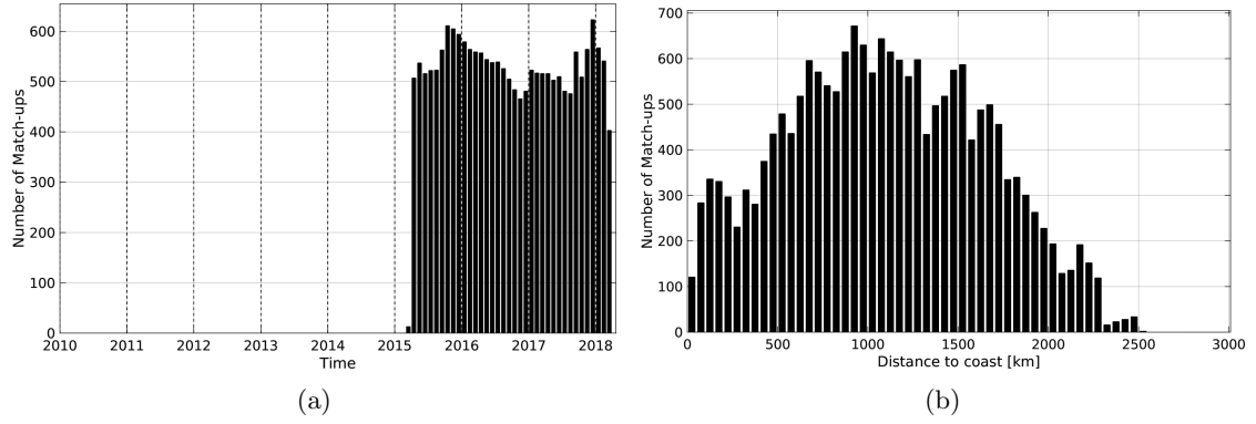
Figure 1: Number of match-ups between Argo and SMAP-L3-RSS-V2-8DAY-RUNNING-40KM SSS as a function of time (a) and as function of the distance to coast (b) over the OTT zone Pi-MEP region and for the full satellite product period.
