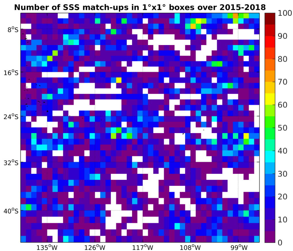
Figure 4: Number of SSS match-ups between Argo SSS and the SMAP-L3-RSS-V2-8DAY-RUNNING-40KM SSS product for the OTT zone Pi-MEP region over 1°x1° boxes and for the full satellite product period.
