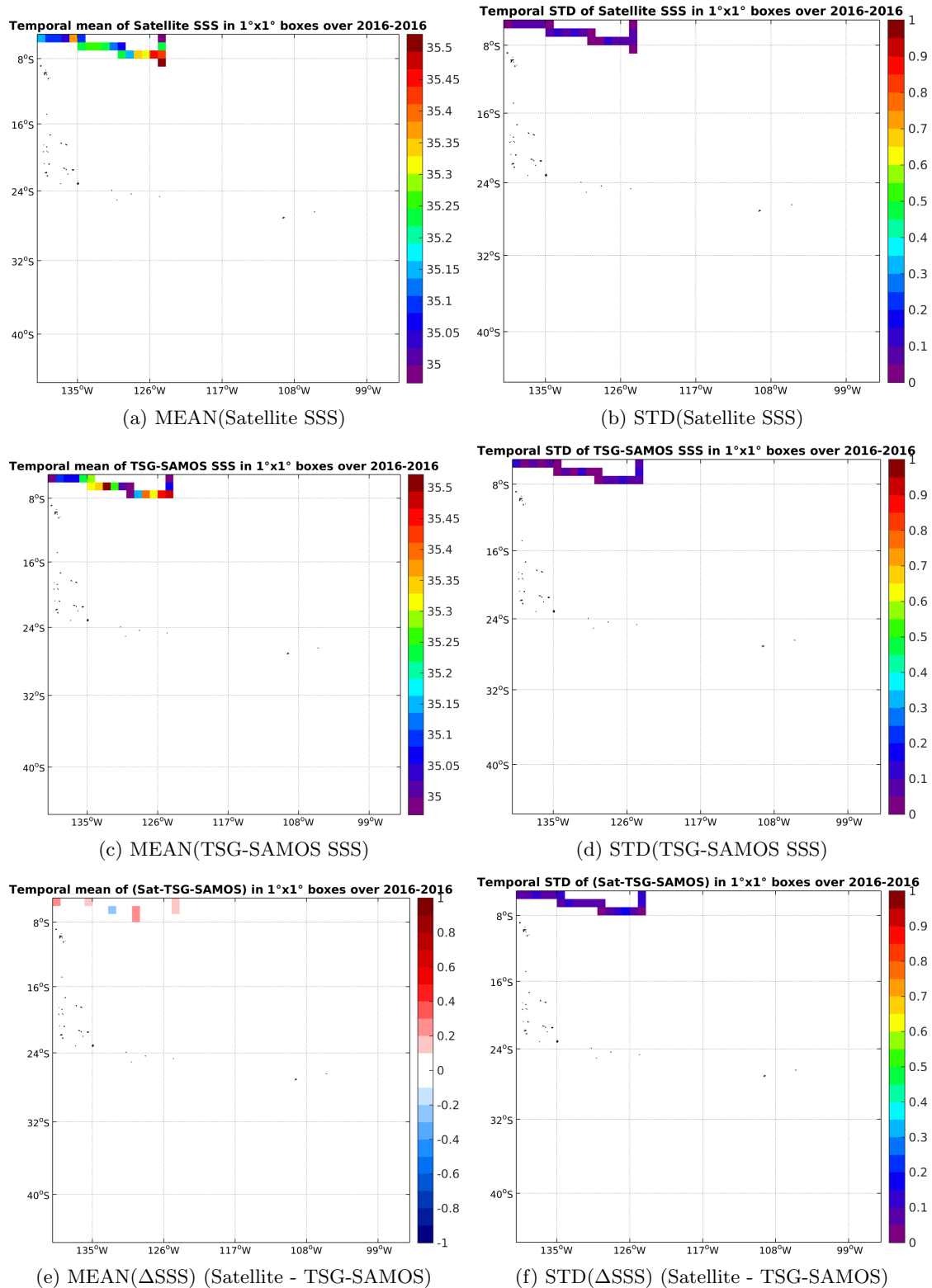
Figure 6: Temporal mean (left) and STD (right) of SSS from SMAP-L3-RSS-V2-MONTHLY-0.25DEG-40KM (top), TSG-SAMOS (middle), and of \Delta SSS (Satellite - TSG-SAMOS). Only match-up pairs are used to generate these maps.
