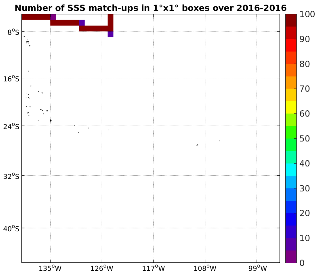
Figure 4: Number of SSS match-ups between TSG-SAMOS SSS and the SMAP-L3-RSS-V2-MONTHLY-0.25DEG-40KM SSS product for the OTT zone Pi-MEP region over 1°x1° boxes and for the full satellite product period.
