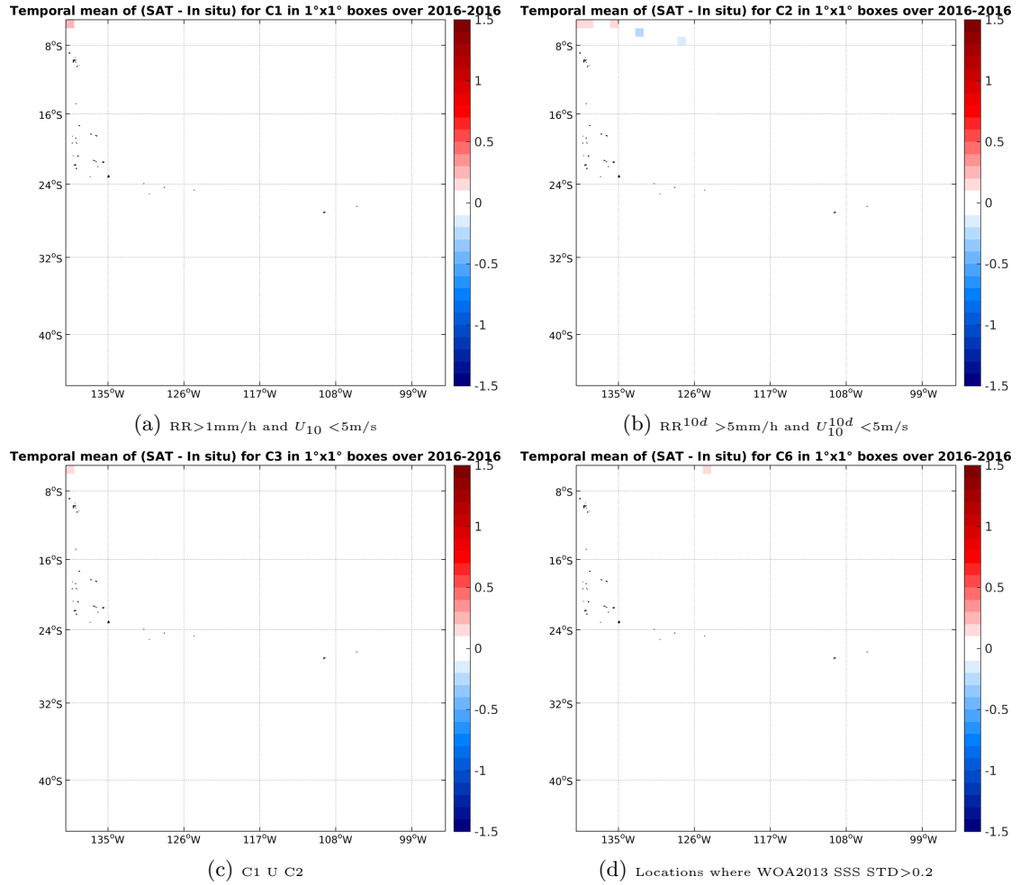
Figure 12: Temporal mean gridded over spatial boxes of size 1^\circ \times 1^\circ of \Delta SSS (SMAP-L3-RSS-V2-MONTHLY-0.25DEG-40KM - TSG-SAMOS) for 4 different subdatasets corresponding to: RR > 1\text{mm/h} and U_{10} < 5\text{m/s} (a), RR^{10d} > 5\text{mm/h} and U_{10}^{10d} < 5\text{m/s} (b), C1 U C2 (c), Locations where WOA2013 SSS STD > 0.2 (d).
