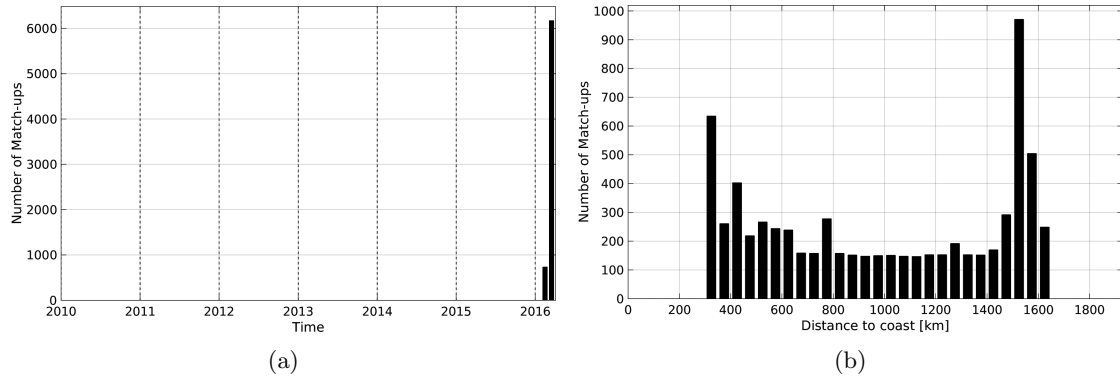
Figure 1: Number of match-ups between TSG-SAMOS and SMAP-L3-RSS-V2-MONTHLY-0.25DEG-40KM SSS as a function of time (a) and as function of the distance to coast (b) over the OTT zone Pi-MEP region and for the full satellite product period.
