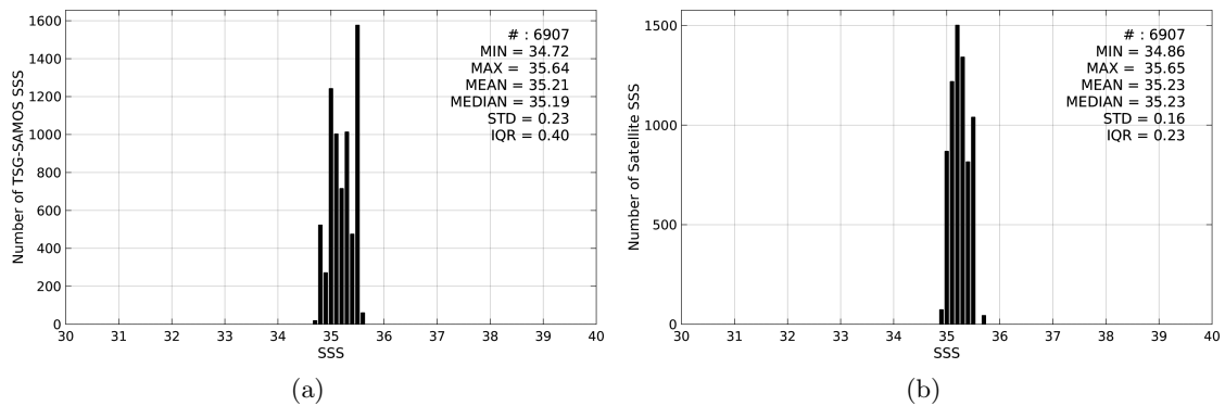
Figure 2: Histograms of SSS from TSG-SAMOS (a) and SMAP-L3-RSS-V2-MONTHLY-0.25DEG-40KM (b) considering all match-up pairs per bins of 0.1 over the OTT zone Pi-MEP region and for the full satellite product period.
