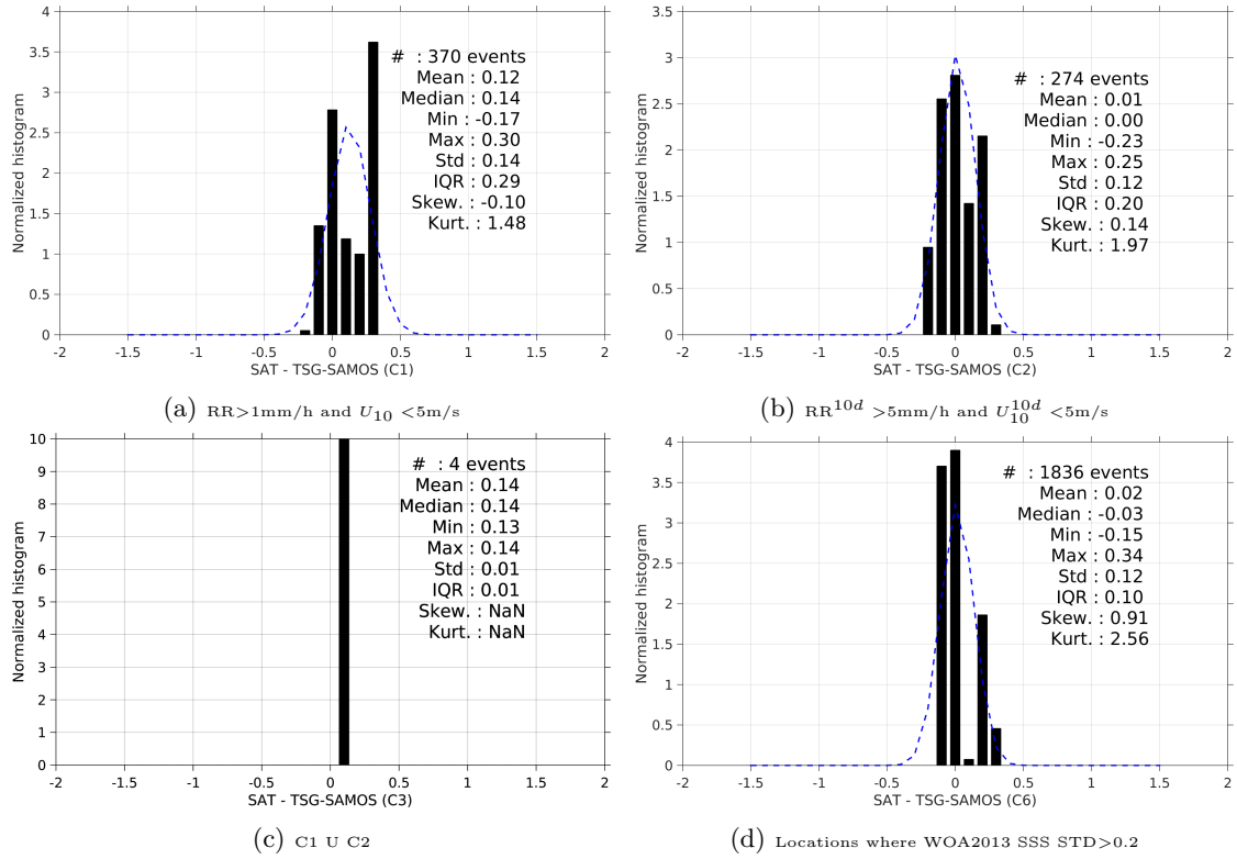
Figure 13: Normalized histogram of \Delta\text{SSS} (SMAP-L3-RSS-V2-MONTHLY-0.25DEG-40KM - TSG-SAMOS) for 6 different subdatasets corresponding to: RR > 1\text{mm/h} and U_{10} < 5\text{m/s} (a), RR^{10d} > 5\text{mm/h} and U_{10}^{10d} < 5\text{m/s} (b), C1 U C2 (c), Locations where WOA2013 SSS STD > 0.2 (d).
