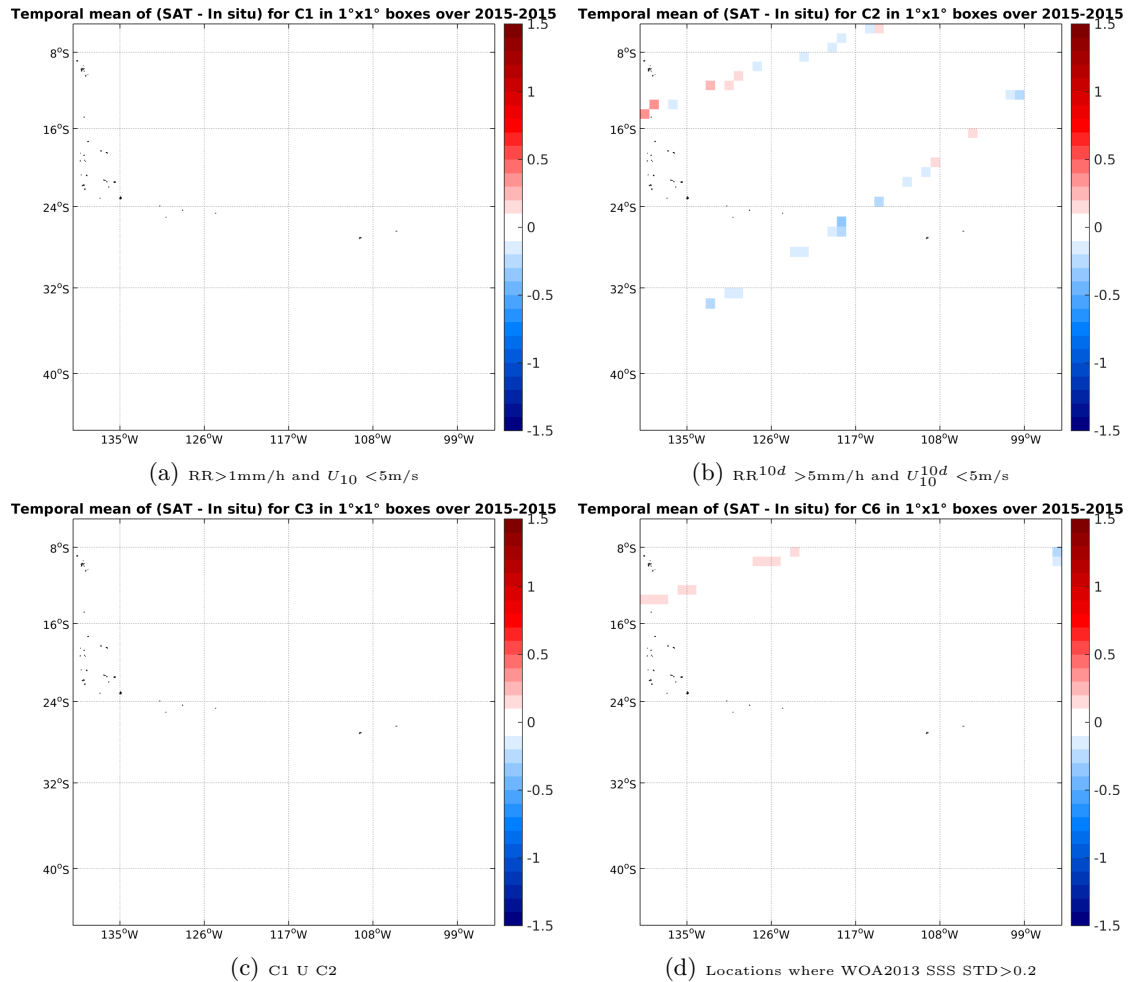
Figure 12: Temporal mean gridded over spatial boxes of size 1^\circ \times 1^\circ of \Delta SSS (SMAP-L3-RSS-V2-MONTHLY-0.25DEG-40KM - TSG-LEGOS-DM) for 4 different subdatasets corresponding to: RR > 1mm/h and U_{10} < 5\text{m/s} (a), RR^{10d} > 5\text{mm/h} and U_{10}^{10d} < 5\text{m/s} (b), C1 U C2 (c), Locations where WOA2013 SSS STD > 0.2 (d).
