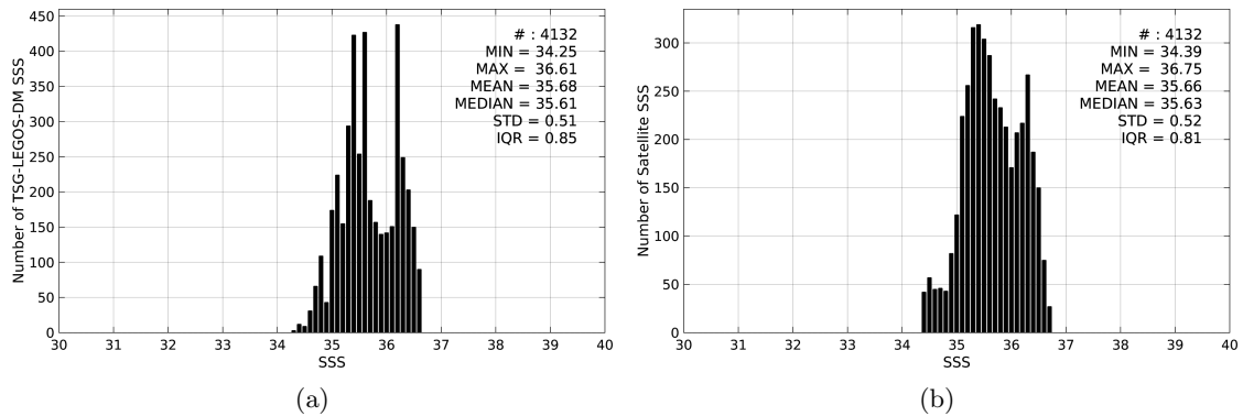
Figure 2: Histograms of SSS from TSG-LEGOS-DM (a) and SMAP-L3-RSS-V2-MONTHLY-0.25DEG-40KM (b) considering all match-up pairs per bins of 0.1 over the OTT zone Pi-MEP region and for the full satellite product period.
