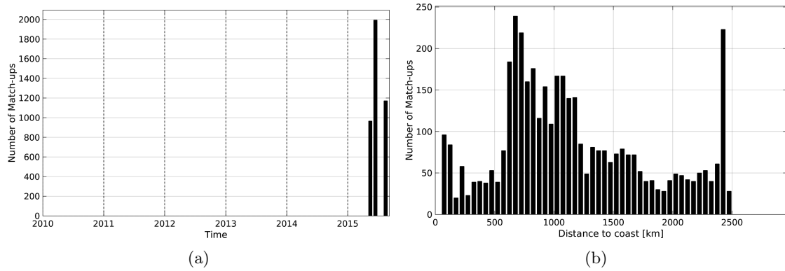
Figure 1: Number of match-ups between TSG-LEGOS-DM and SMAP-L3-RSS-V2-MONTHLY-0.25DEG-40KM SSS as a function of time (a) and as function of the distance to coast (b) over the OTT zone Pi-MEP region and for the full satellite product period.
