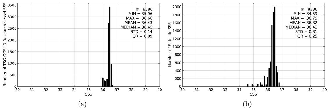
Figure 2: Histograms of SSS from TSG-GOSUD-Research-vessel (a) and SMAP-L3-RSS-V2-MONTHLY-0.25DEG-40KM (b) considering all match-up pairs per bins of 0.1 over the OTT zone Pi-MEP region and for the full satellite product period.
