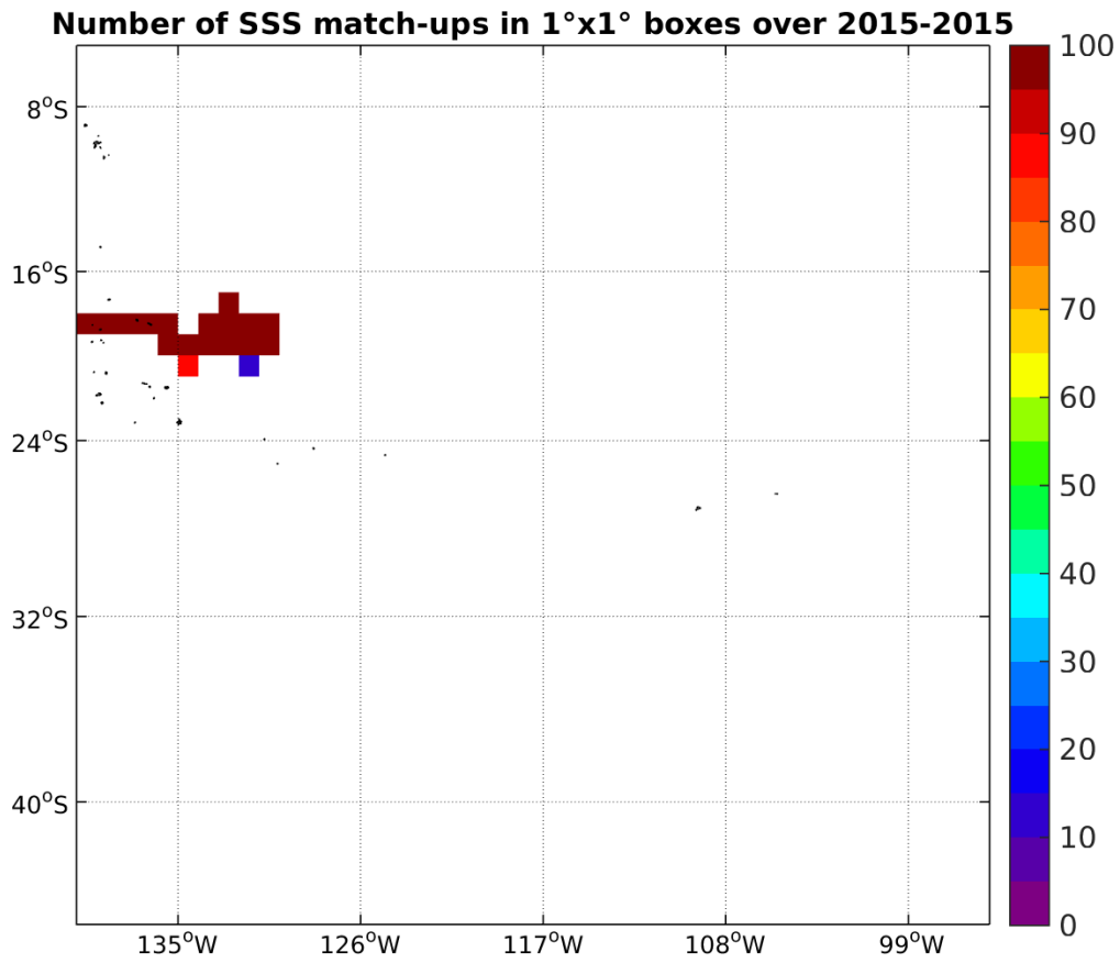
Figure 4: Number of SSS match-ups between TSG-GOSUD-Research-vessel SSS and the SMAP-L3-RSS-V2-MONTHLY-0.25DEG-40KM SSS product for the OTT zone Pi-MEP region over 1°x1° boxes and for the full satellite product period.
