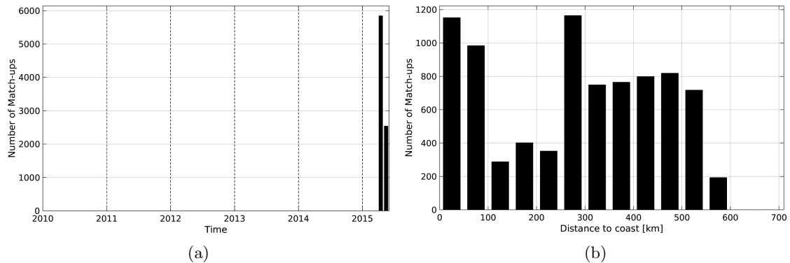
Figure 1: Number of match-ups between TSG-GOSUD-Research-vessel and SMAP-L3-RSS-V2-MONTHLY-0.25DEG-40KM SSS as a function of time (a) and as function of the distance to coast (b) over the OTT zone Pi-MEP region and for the full satellite product period.
