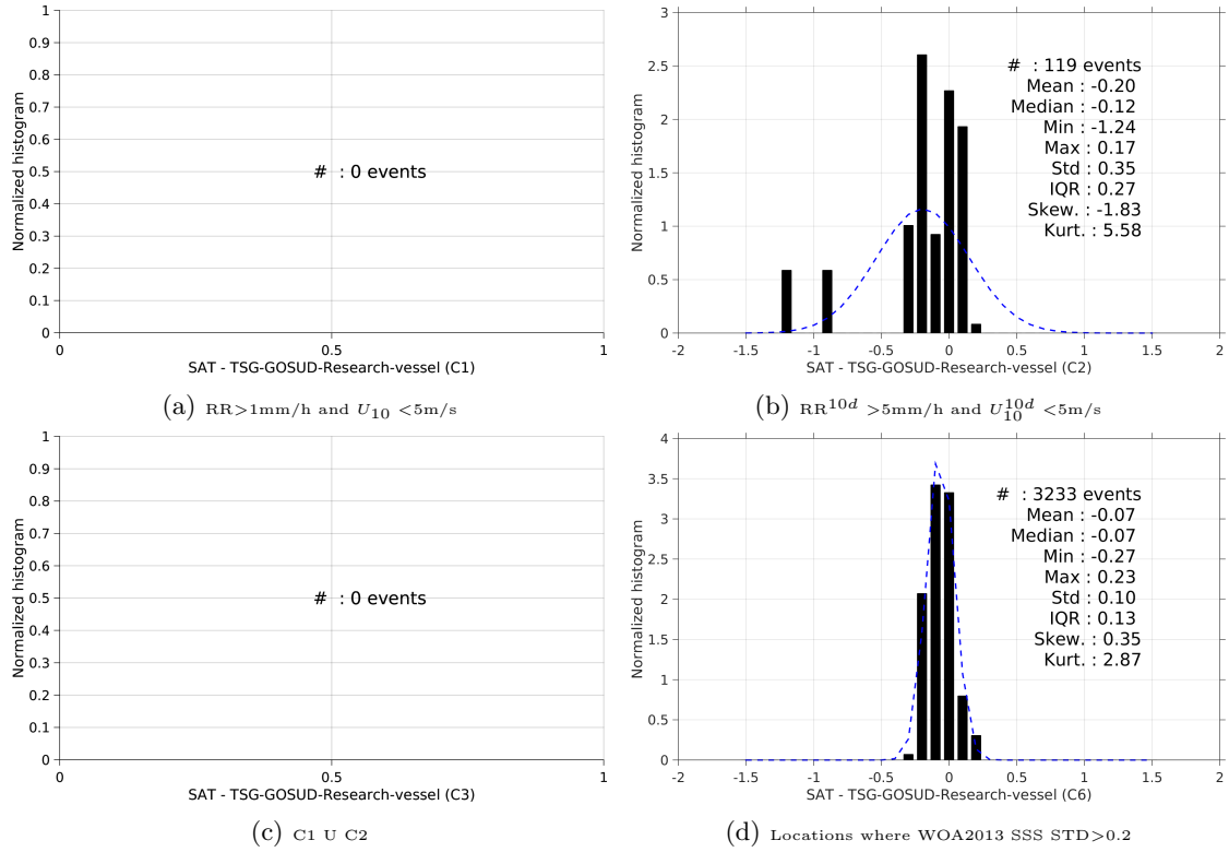
Figure 13: Normalized histogram of \Delta\text{SSS} (SMAP-L3-RSS-V2-MONTHLY-0.25DEG-40KM - TSG-GOSUD-Research-vessel) for 6 different subdatasets corresponding to: RR > 1\text{mm/h} and U_{10} < 5\text{m/s} (a), RR^{10d} > 5\text{mm/h} and U_{10}^{10d} < 5\text{m/s} (b), C1 \cup C2 (c), Locations where WOA2013 SSS STD > 0.2 (d).
