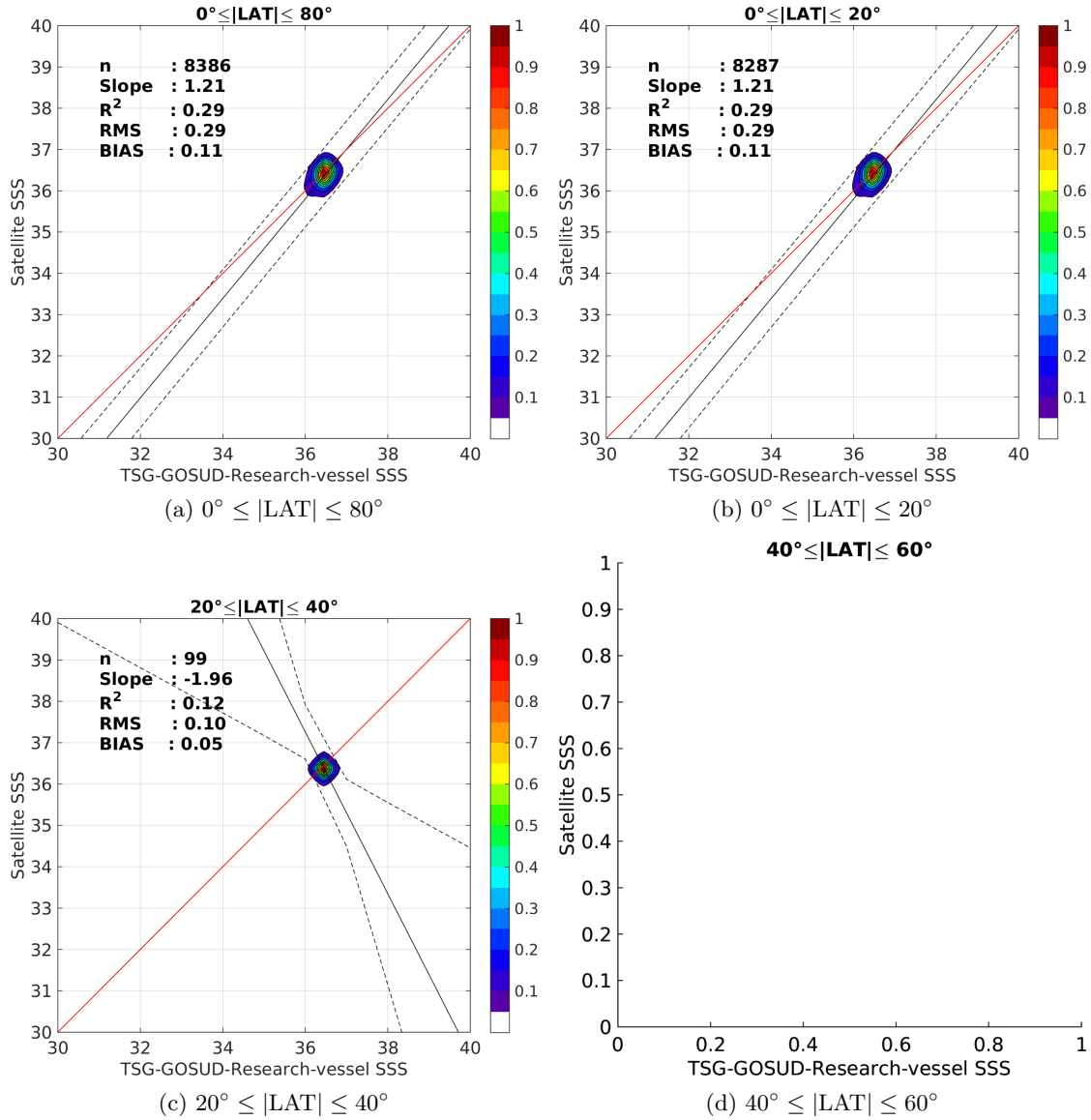
Figure 9: Contour maps of the concentration of SMAP-L3-RSS-V2-MONTHLY-0.25DEG-40KM SSS (y-axis) versus TSG-GOSUD-Research-vessel SSS (x-axis) at match-up pairs for different latitude bands. For each plot, the red line shows x=y . The black thin and dashed lines indicate a linear fit through the data cloud and the \pm 95\% confidence levels, respectively. The number match-up pairs n , the slope and R^2 coefficient of the linear fit, the root mean square (RMS) and the mean bias between satellite and in situ data are indicated for each latitude band in each plots.
