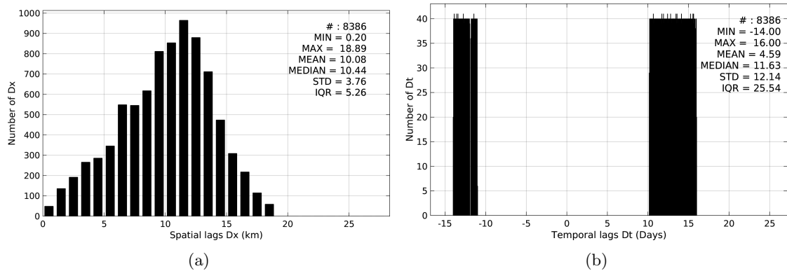
Figure 5: Histograms of the spatial (a) and temporal (b) lags between the time of the TSG-GOSUD-Research-vessel measurements and the date of the corresponding SMAP-L3-RSS-V2-MONTHLY-0.25DEG-40KM SSS product.
