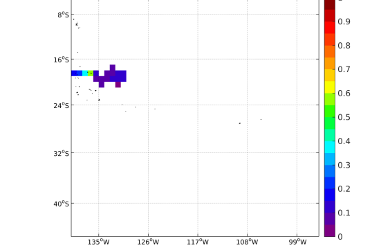
(f) STD( \Delta SSS) (Satellite - TSG-GOSUD-Research-vessel)
