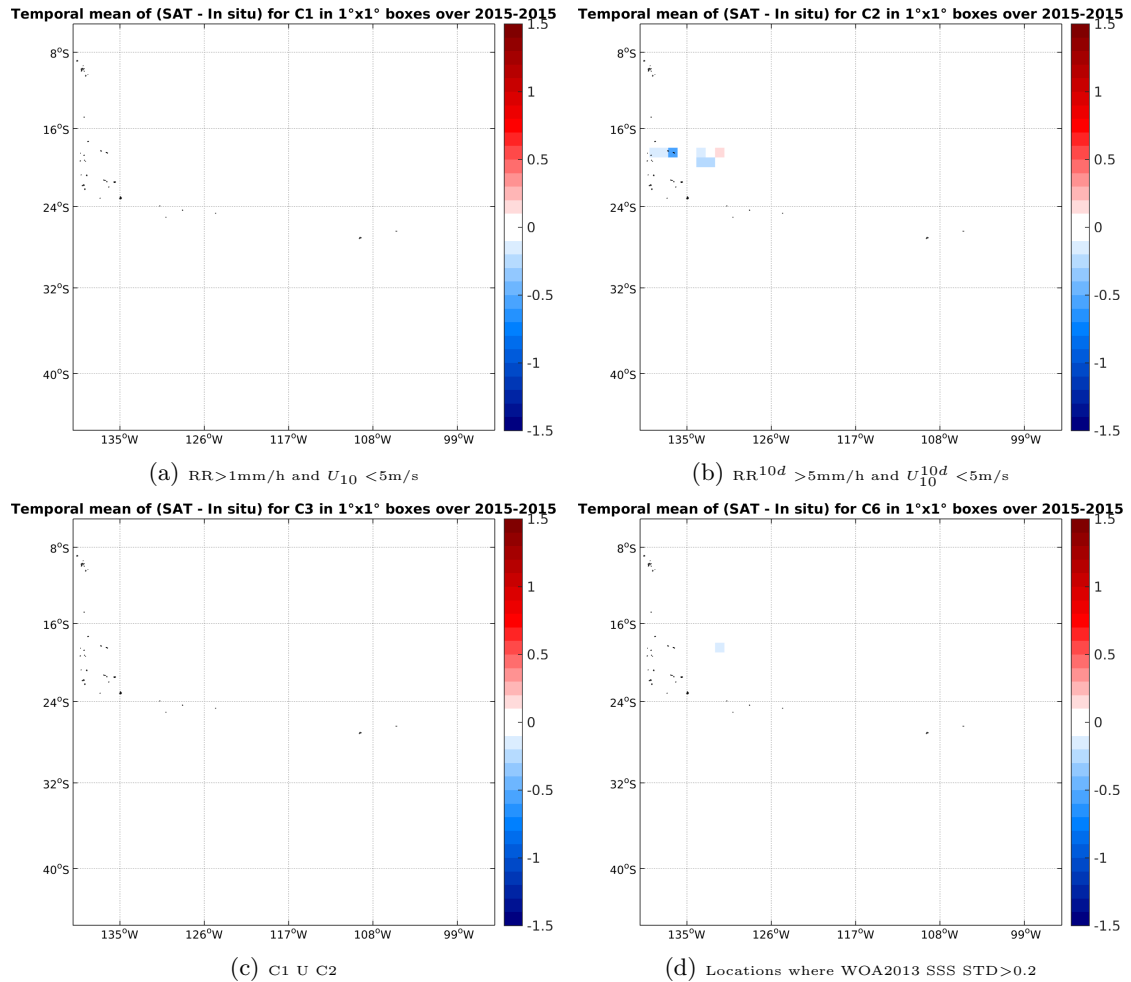
Figure 12: Temporal mean gridded over spatial boxes of size 1^\circ \times 1^\circ of \Delta SSS (SMAP-L3-RSS-V2-MONTHLY-0.25DEG-40KM - TSG-GOSUD-Research-vessel) for 4 different subdatasets corresponding to: RR > 1\text{mm/h} and U_{10} < 5\text{m/s} (a), RR^{10d} > 5\text{mm/h} and U_{10}^{10d} < 5\text{m/s} (b), C1 U C2 (c), Locations where WOA2013 SSS STD > 0.2 (d).
