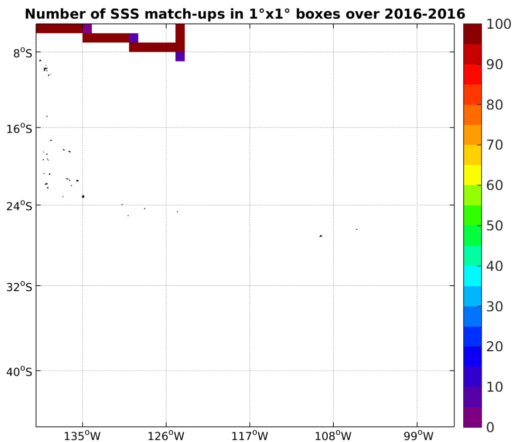
Figure 4: Number of SSS match-ups between TSG-SAMOS SSS and the SMAP-L3-RSS-V2-MONTHLY-70KM SSS product for the OTT zone Pi-MEP region over 1°x1° boxes and for the full satellite product period.
