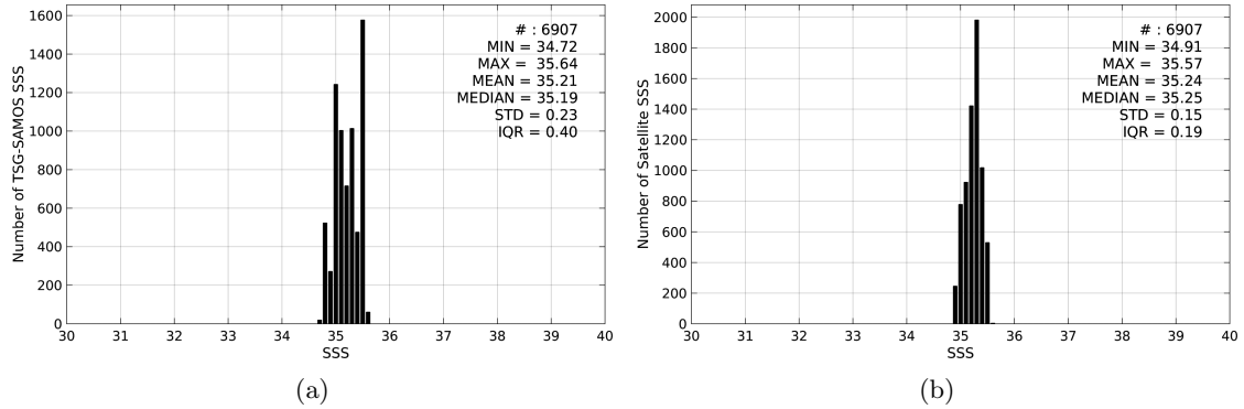
Figure 2: Histograms of SSS from TSG-SAMOS (a) and SMAP-L3-RSS-V2-MONTHLY-70KM (b) considering all match-up pairs per bins of 0.1 over the OTT zone Pi-MEP region and for the full satellite product period.
