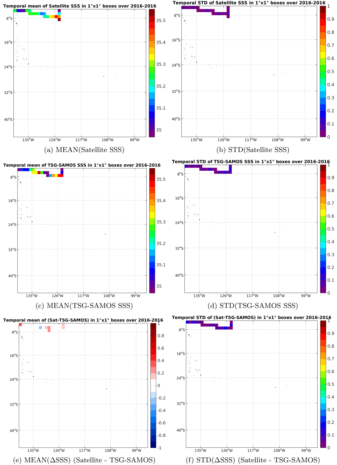
Figure 6: Temporal mean (left) and STD (right) of SSS from SMAP-L3-RSS-V2-MONTHLY-70KM (top), TSG-SAMOS (middle), and of \Delta SSS (Satellite - TSG-SAMOS). Only match-up pairs are used to generate these maps.
