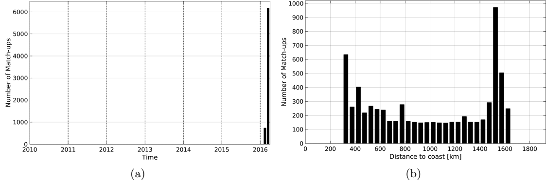
Figure 1: Number of match-ups between TSG-SAMOS and SMAP-L3-RSS-V2-MONTHLY-70KM SSS as a function of time (a) and as function of the distance to coast (b) over the OTT zone Pi-MEP region and for the full satellite product period.
