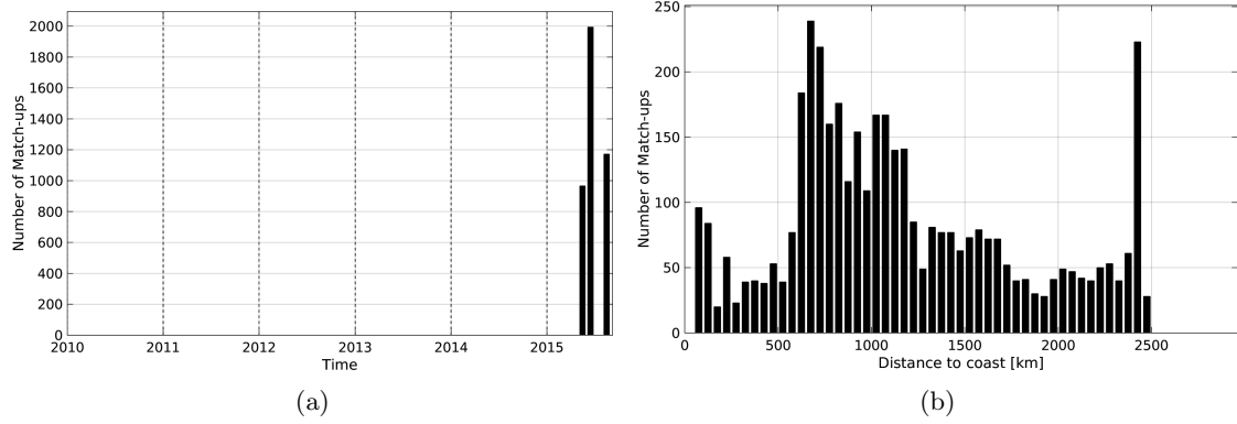
Figure 1: Number of match-ups between TSG-LEGOS-DM and SMAP-L3-RSS-V2-MONTHLY-70KM SSS as a function of time (a) and as function of the distance to coast (b) over the OTT zone Pi-MEP region and for the full satellite product period.
