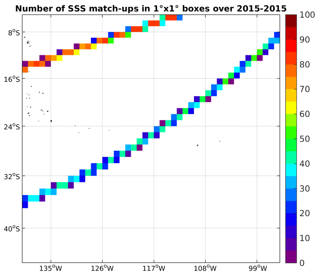
Figure 4: Number of SSS match-ups between TSG-LEGOS-DM SSS and the SMAP-L3-RSS-V2-MONTHLY-70KM SSS product for the OTT zone Pi-MEP region over 1°x1° boxes and for the full satellite product period.
