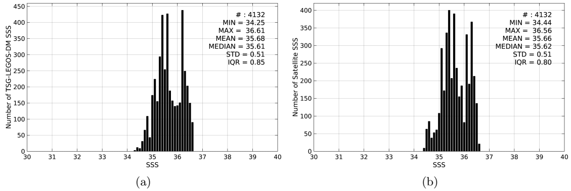
Figure 2: Histograms of SSS from TSG-LEGOS-DM (a) and SMAP-L3-RSS-V2-MONTHLY-70KM (b) considering all match-up pairs per bins of 0.1 over the OTT zone Pi-MEP region and for the full satellite product period.
