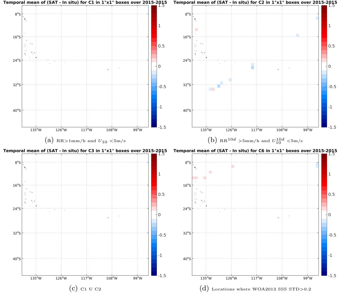
Figure 12: Temporal mean gridded over spatial boxes of size 1^\circ \times 1^\circ of \Delta SSS (SMAP-L3-RSS-V2-MONTHLY-70KM - TSG-LEGOS-DM) for 4 different subdatasets corresponding to: RR > 1\text{mm/h} and U_{10} < 5\text{m/s} (a), RR^{10d} > 5\text{mm/h} and U_{10}^{10d} < 5\text{m/s} (b), C1 U C2 (c), Locations where WOA2013 SSS STD > 0.2 (d).
