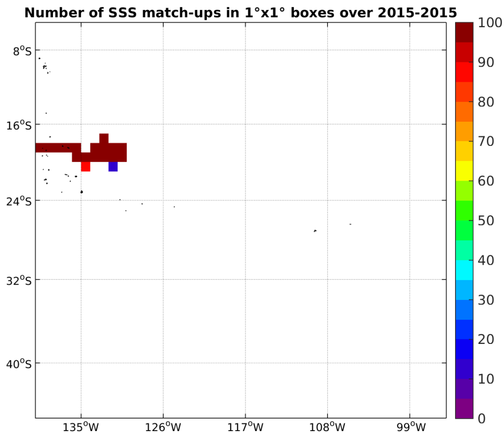
Figure 4: Number of SSS match-ups between TSG-GOSUD-Research-vessel SSS and the SMAP-L3-RSS-V2-MONTHLY-70KM SSS product for the OTT zone Pi-MEP region over 1°x1° boxes and for the full satellite product period.
