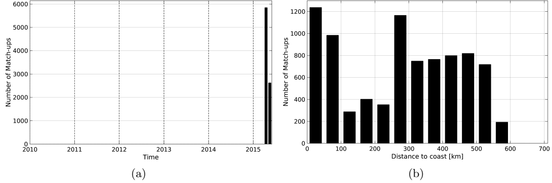
Figure 1: Number of match-ups between TSG-GOSUD-Research-vessel and SMAP-L3-RSS-V2-MONTHLY-70KM SSS as a function of time (a) and as function of the distance to coast (b) over the OTT zone Pi-MEP region and for the full satellite product period.
