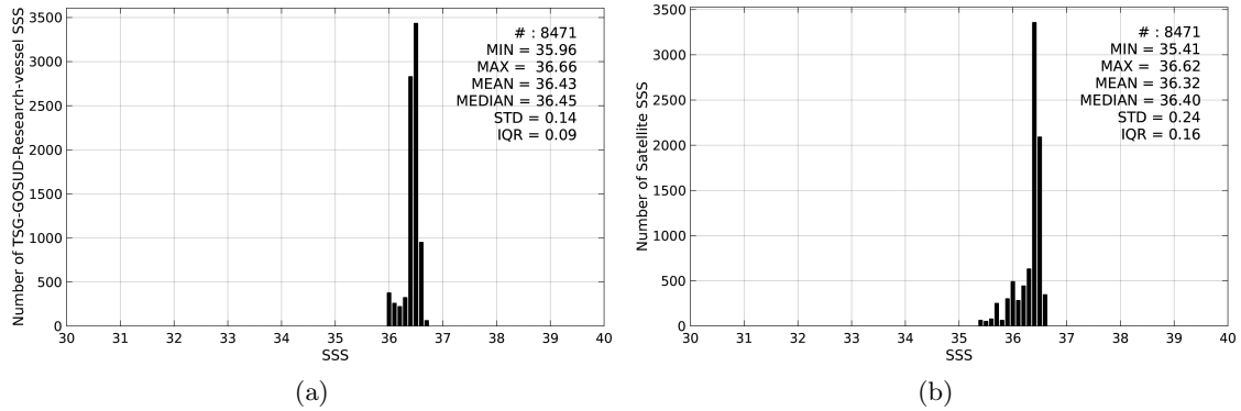
Figure 2: Histograms of SSS from TSG-GOSUD-Research-vessel (a) and SMAP-L3-RSS-V2-MONTHLY-70KM (b) considering all match-up pairs per bins of 0.1 over the OTT zone Pi-MEP region and for the full satellite product period.
