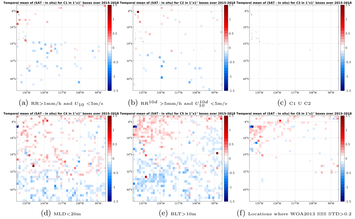
Figure 12: Temporal mean gridded over spatial boxes of size 1^\circ \times 1^\circ of \Delta SSS (SMAP-L3-RSS-V2-MONTHLY-70KM - Argo) for 6 different subdatasets corresponding to: RR > 1mm/h and U_{10} < 5\text{m/s} (a), RR^{10d} > 5\text{mm/h} and U_{10}^{10d} < 5\text{m/s} (b), C1 U C2 (c), MLD < 20m (d), BLT > 10m (e), Locations where WOA2013 SSS STD > 0.2 (f).
