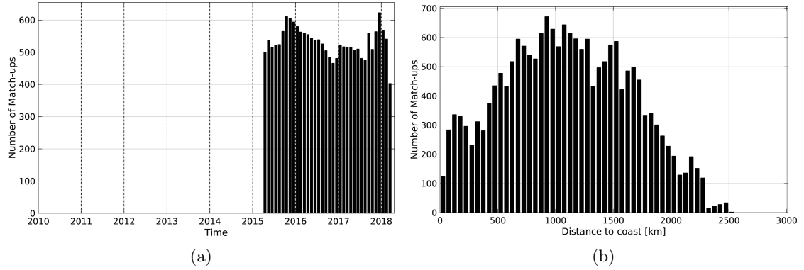
Figure 1: Number of match-ups between Argo and SMAP-L3-RSS-V2-MONTHLY-70KM SSS as a function of time (a) and as function of the distance to coast (b) over the OTT zone Pi-MEP region and for the full satellite product period.
