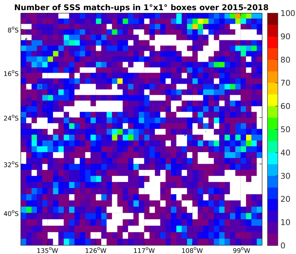
Figure 4: Number of SSS match-ups between Argo SSS and the SMAP-L3-RSS-V2-MONTHLY-70KM SSS product for the OTT zone Pi-MEP region over 1°x1° boxes and for the full satellite product period.
