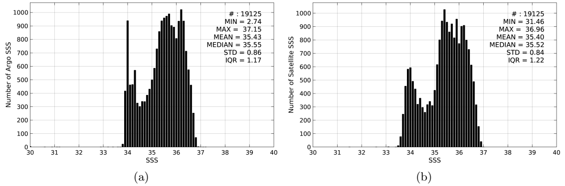
Figure 2: Histograms of SSS from Argo (a) and SMAP-L3-RSS-V2-MONTHLY-70KM (b) considering all match-up pairs per bins of 0.1 over the OTT zone Pi-MEP region and for the full satellite product period.
