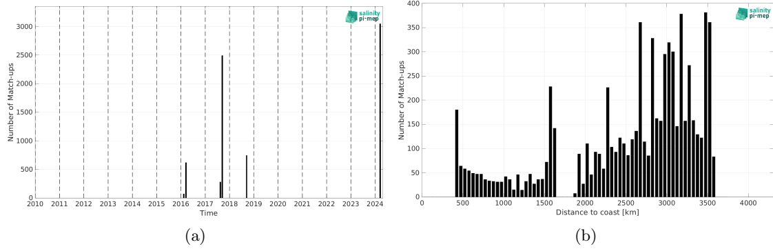
Figure 2: Number of match-ups between TSG (SAMOS) and SMAP SSS L3 v5.0 - 8-Day running (JPL) SSS as a function of time (a) and as function of the distance to coast (b) over the OTT zone Pi-MEP region and for the full satellite product period.
