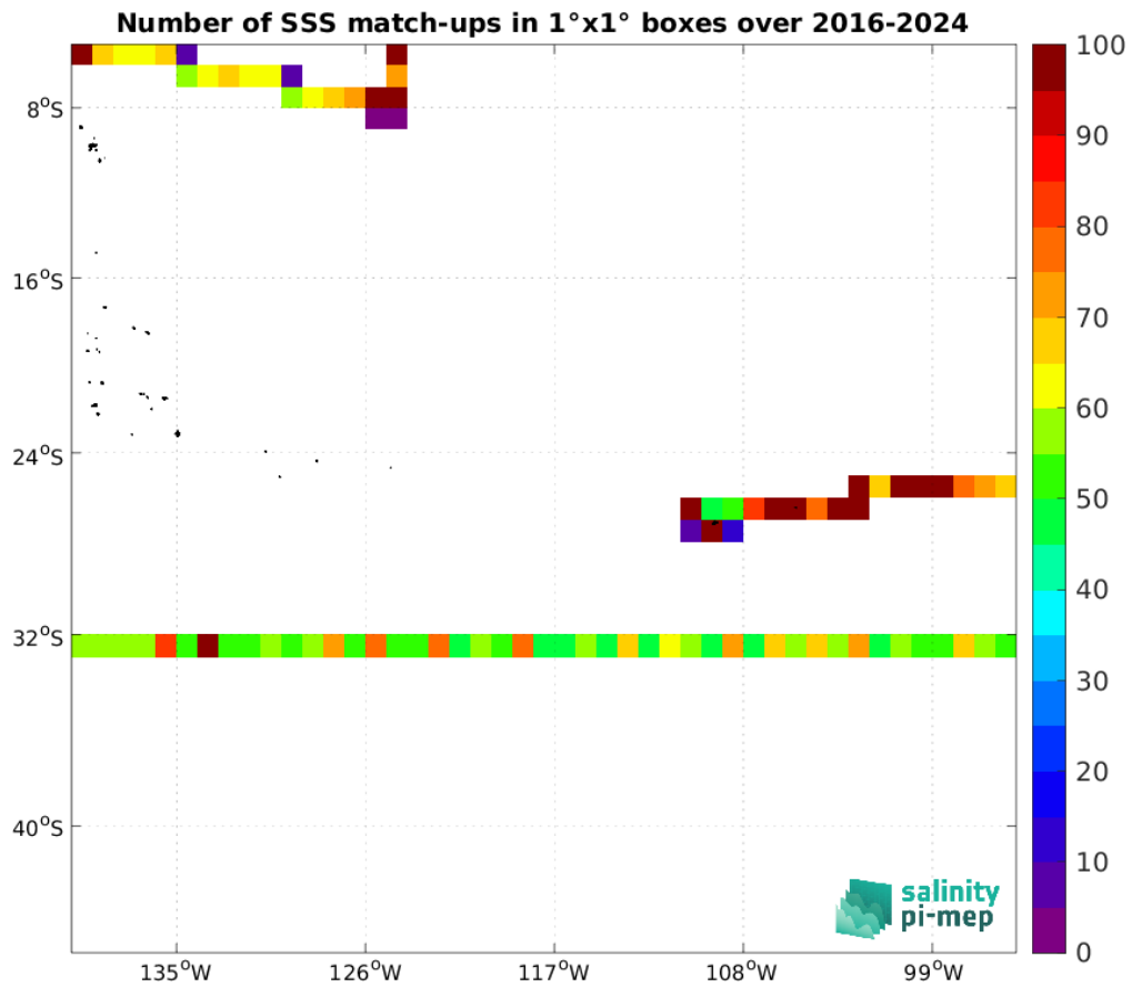
Figure 5: Number of SSS match-ups between TSG (SAMOS) SSS and the SMAP SSS L3 v5.0 - 8-Day running (JPL) SSS product for the OTT zone Pi-MEP region over 1^\circ \times 1^\circ boxes and for the full satellite product period.
