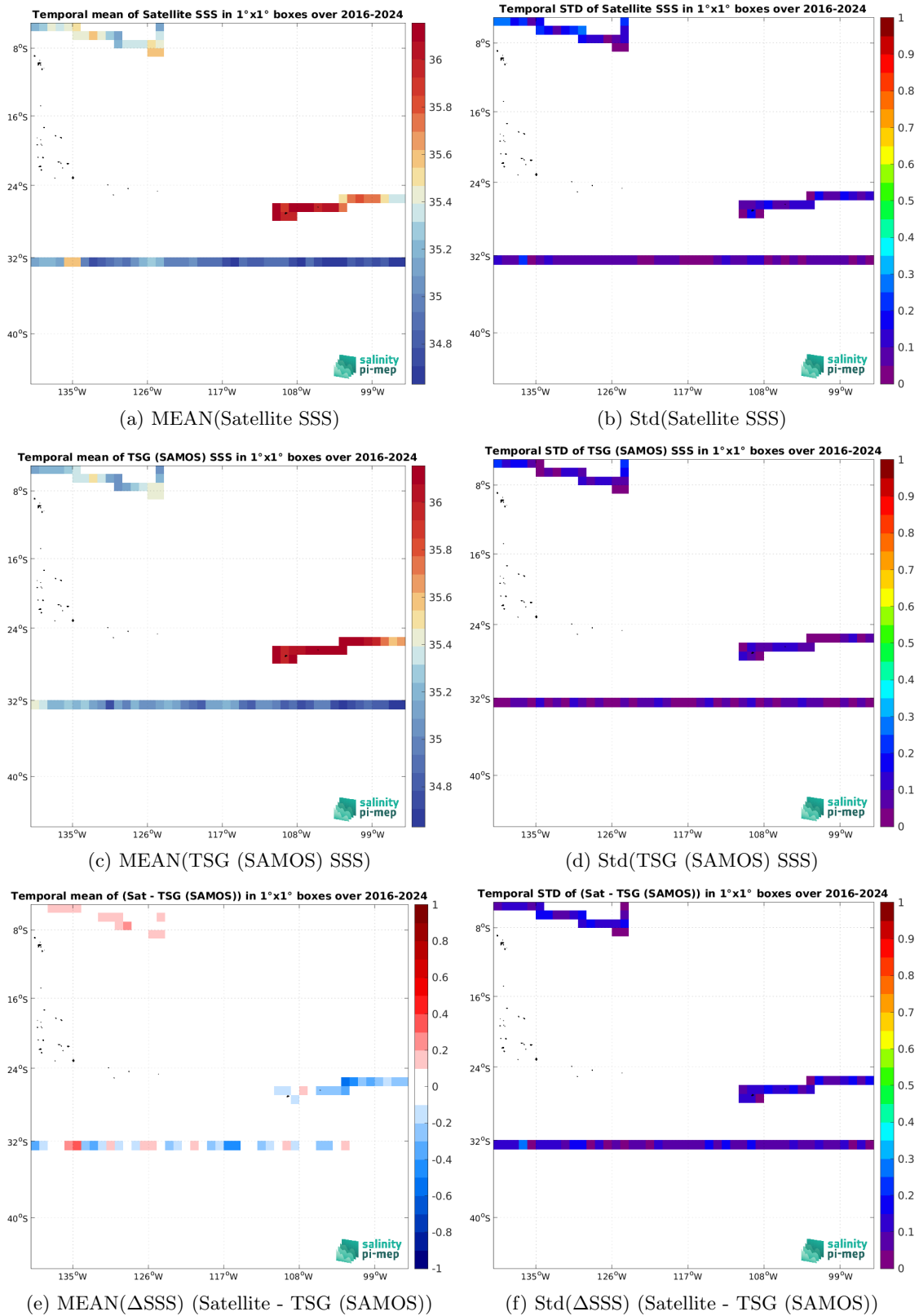
Figure 7: Temporal mean (left) and Std (right) of SSS from SMAP SSS L3 v5.0 - 8-Day running (JPL) (top), TSG (SAMOS) (middle), and of \Delta SSS (Satellite - TSG (SAMOS)). Only match-up pairs are used to generate these maps.
