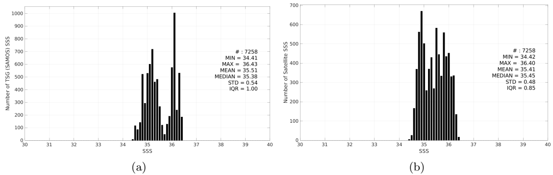
Figure 3: Histograms of SSS from TSG (SAMOS) (a) and SMAP SSS L3 v5.0 - 8-Day running (JPL) (b) considering all match-up pairs per bins of 0.1 over the OTT zone Pi-MEP region and for the full satellite product period.
