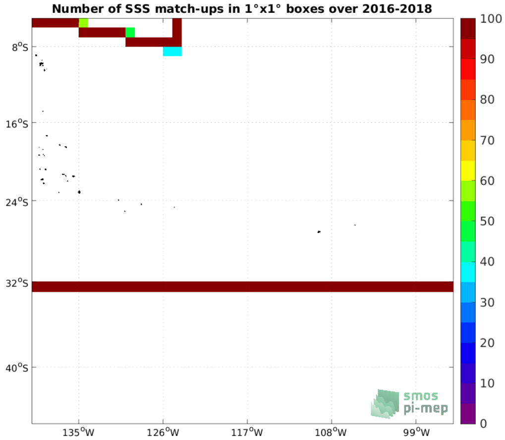
Figure 4: Number of SSS match-ups between TSG (SAMOS) SSS and the SMAP SSS L3 v5.0 - 8-Day running (JPL) SSS product for the OTT zone Pi-MEP region over 1^\circ \times 1^\circ boxes and for the full satellite product period.
