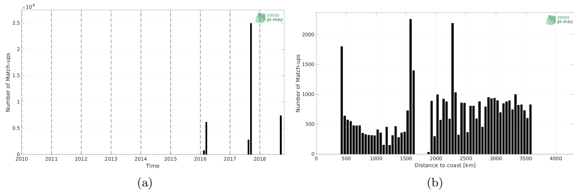
Figure 1: Number of match-ups between TSG (SAMOS) and SMAP SSS L3 v5.0 - 8-Day running (JPL) SSS as a function of time (a) and as function of the distance to coast (b) over the OTT zone Pi-MEP region and for the full satellite product period.
