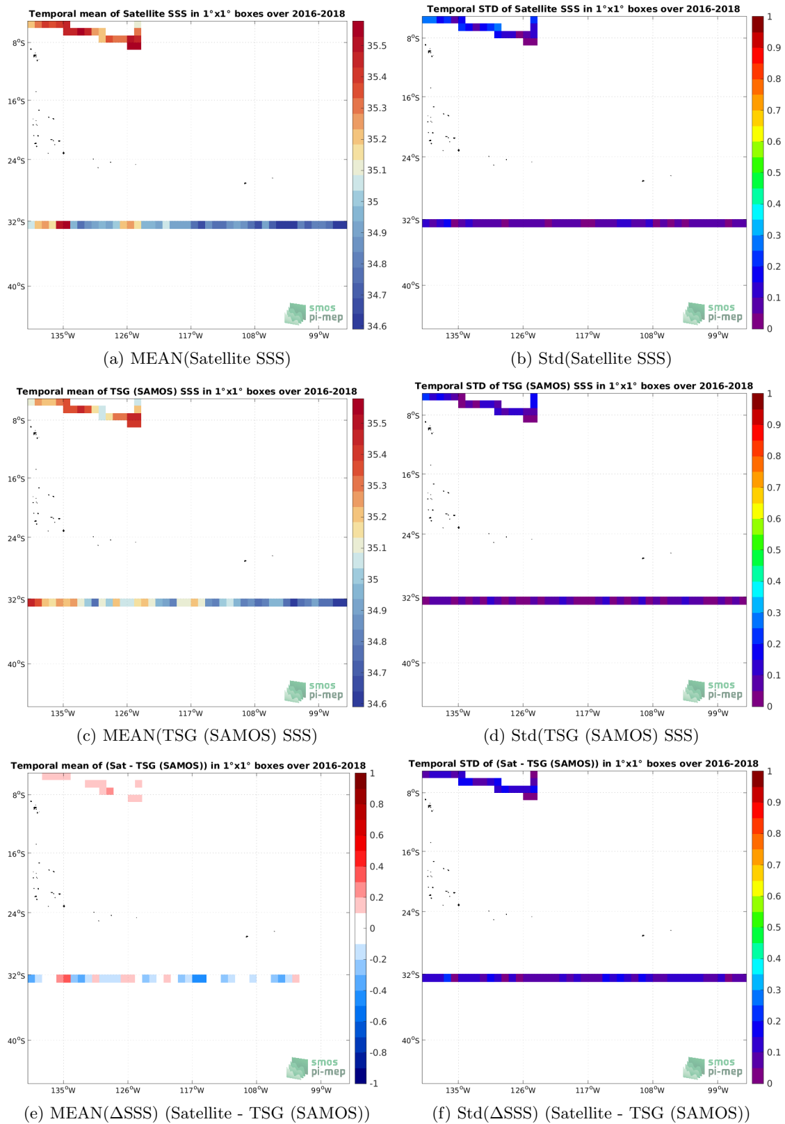
Figure 6: Temporal mean (left) and Std (right) of SSS from SMAP SSS L3 v5.0 - 8-Day running (JPL) (top), TSG (SAMOS) (middle), and of \Delta SSS (Satellite - TSG (SAMOS)). Only match-up pairs are used to generate these maps.
