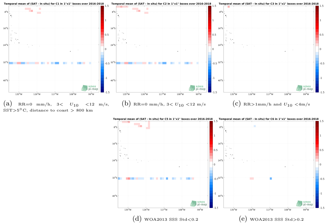
Figure 12: Temporal mean gridded over spatial boxes of size 1^\circ \times 1^\circ of \Delta SSS (SMAP SSS L3 v5.0 - 8-Day running (JPL) - TSG (SAMOS)) for 5 different subdatasets corresponding to: RR=0 mm/h, 3 < U_{10} < 12 m/s, SST > 5^\circ C , distance to coast > 800 km (a), RR=0 mm/h, 3 < U_{10} < 12 m/s (b), RR > 1 mm/h and U_{10} < 4 m/s (c), WOA2013 SSS Std < 0.2 (d), WOA2013 SSS Std > 0.2 (e).
