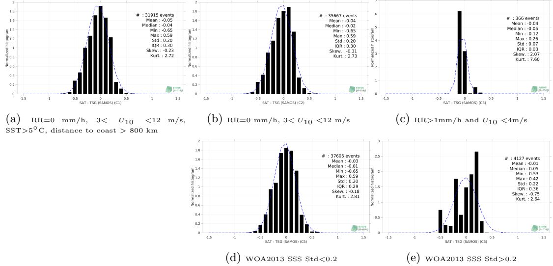
Figure 13: Normalized histogram of \Delta\text{SSS} (SMAP SSS L3 v5.0 - 8-Day running (JPL) - TSG (SAMOS)) for 5 different subdatasets corresponding to: RR=0 mm/h, 3 < U_{10} < 12 m/s, SST > 5^{\circ}\text{C} , distance to coast > 800 km (a), RR=0 mm/h, 3 < U_{10} < 12 m/s (b), RR > 1\text{mm/h} and U_{10} < 4\text{m/s} (c), WOA2013 SSS Std < 0.2 (d), WOA2013 SSS Std > 0.2 (e).
