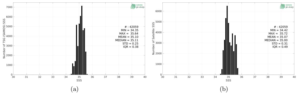
Figure 2: Histograms of SSS from TSG (SAMOS) (a) and SMAP SSS L3 v5.0 - 8-Day running (JPL) (b) considering all match-up pairs per bins of 0.1 over the OTT zone Pi-MEP region and for the full satellite product period.
