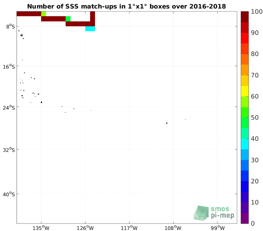
Figure 4: Number of SSS match-ups between TSG (SAMOS) SSS and the SMAP SSS L3 v5.0 - 8-Day running (JPL) SSS product for the OTT zone Pi-MEP region over 1°x1° boxes and for the full satellite product period.
