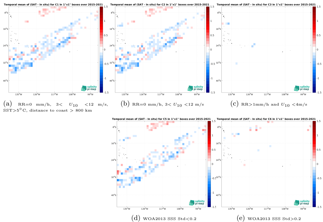
Figure 14: Temporal mean gridded over spatial boxes of size 1^\circ \times 1^\circ of \Delta\text{SSS} (SMAP SSS L3 v5.0 - 8-Day running (JPL) - TSG (LEGOS-DM)) for 5 different subdatasets corresponding to:RR=0 mm/h, 3 < U_{10} < 12 m/s, SST >5^\circ\text{C} , distance to coast > 800 km (a), RR=0 mm/h, 3 < U_{10} < 12 m/s (b), RR >1 mm/h and U_{10} < 4 m/s (c), WOA2013 SSS Std <0.2 (d), WOA2013 SSS Std >0.2 (e).
