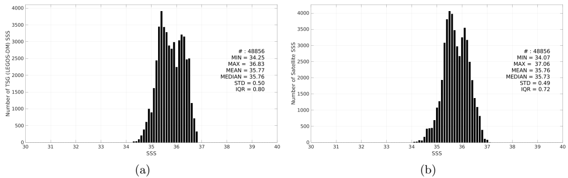
Figure 3: Histograms of SSS from TSG (LEGOS-DM) (a) and SMAP SSS L3 v5.0 - 8-Day running (JPL) (b) considering all match-up pairs per bins of 0.1 over the OTT zone Pi-MEP region and for the full satellite product period.
