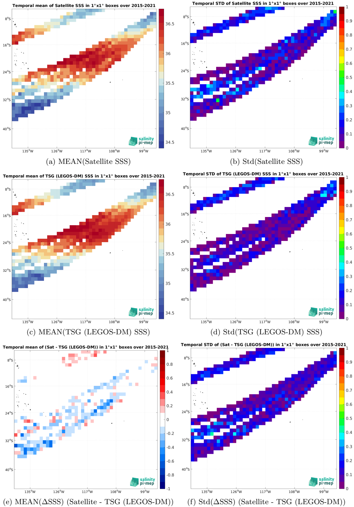
Figure 7: Temporal mean (left) and Std (right) of SSS from SMAP SSS L3 v5.0 - 8-Day running (JPL) (top), TSG (LEGOS-DM) (middle), and of \Delta SSS (Satellite - TSG (LEGOS-DM)). Only match-up pairs are used to generate these maps.
