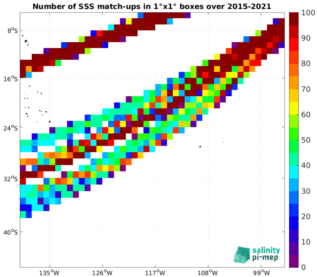
Figure 5: Number of SSS match-ups between TSG (LEGOS-DM) SSS and the SMAP SSS L3 v5.0 - 8-Day running (JPL) SSS product for the OTT zone Pi-MEP region over 1^\circ \times 1^\circ boxes and for the full satellite product period.
