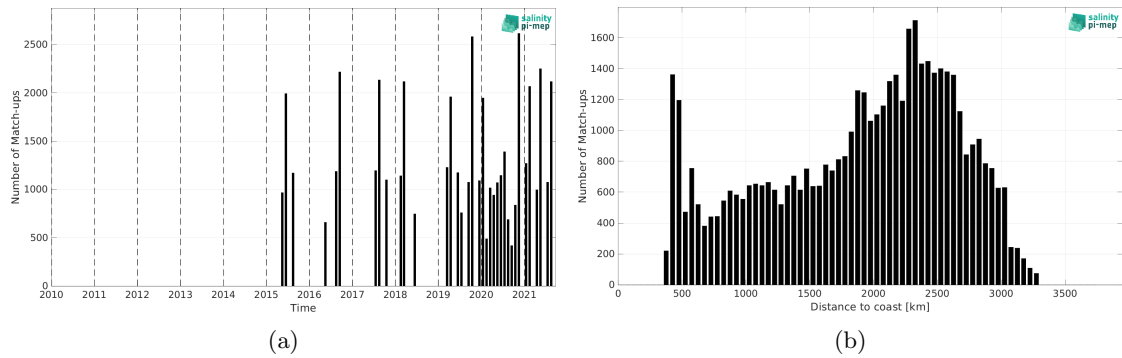
Figure 2: Number of match-ups between TSG (LEGOS-DM) and SMAP SSS L3 v5.0 - 8-Day running (JPL) SSS as a function of time (a) and as function of the distance to coast (b) over the OTT zone Pi-MEP region and for the full satellite product period.
