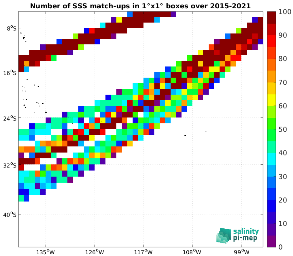
Figure 4: Number of SSS match-ups between TSG (LEGOS-DM) SSS and the SMAP SSS L3 v5.0 - 8-Day running (JPL) SSS product for the OTT zone Pi-MEP region over 1^{\circ} \times 1^{\circ} boxes and for the full satellite product period.
