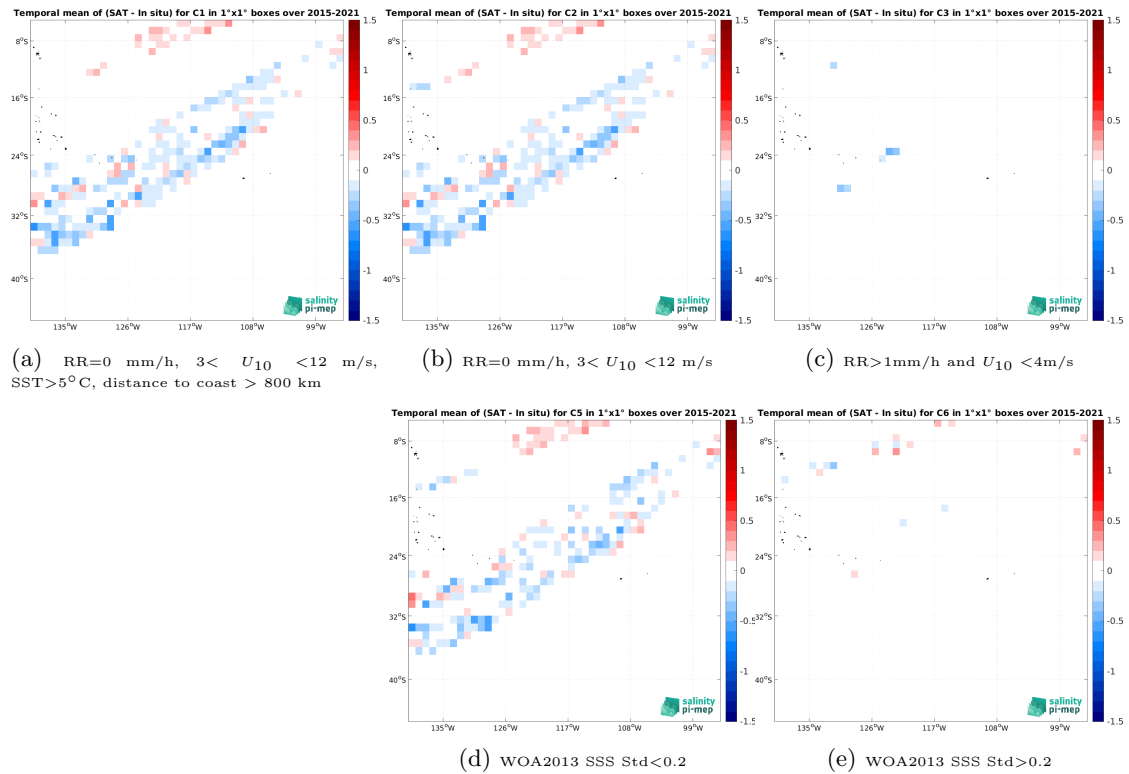
Figure 12: Temporal mean gridded over spatial boxes of size 1^\circ \times 1^\circ of \Delta\text{SSS} (SMAP SSS L3 v5.0 - 8-Day running (JPL) - TSG (LEGOS-DM)) for 5 different subdatasets corresponding to:RR=0 mm/h, 3 < U_{10} < 12 m/s, SST > 5^\circ\text{C} , distance to coast > 800 km (a), RR=0 mm/h, 3 < U_{10} < 12 m/s (b), RR > 1 mm/h and U_{10} < 4 m/s (c), WOA2013 SSS Std < 0.2 (d), WOA2013 SSS Std > 0.2 (e).
