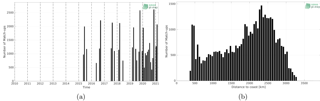
Figure 1: Number of match-ups between TSG (LEGOS-DM) and SMAP SSS L3 v5.0 - 8-Day running (JPL) SSS as a function of time (a) and as function of the distance to coast (b) over the OTT zone Pi-MEP region and for the full satellite product period.
