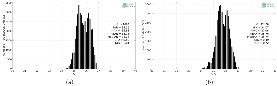
Figure 2: Histograms of SSS from TSG (LEGOS-DM) (a) and SMAP SSS L3 v5.0 - 8-Day running (JPL) (b) considering all match-up pairs per bins of 0.1 over the OTT zone Pi-MEP region and for the full satellite product period.
