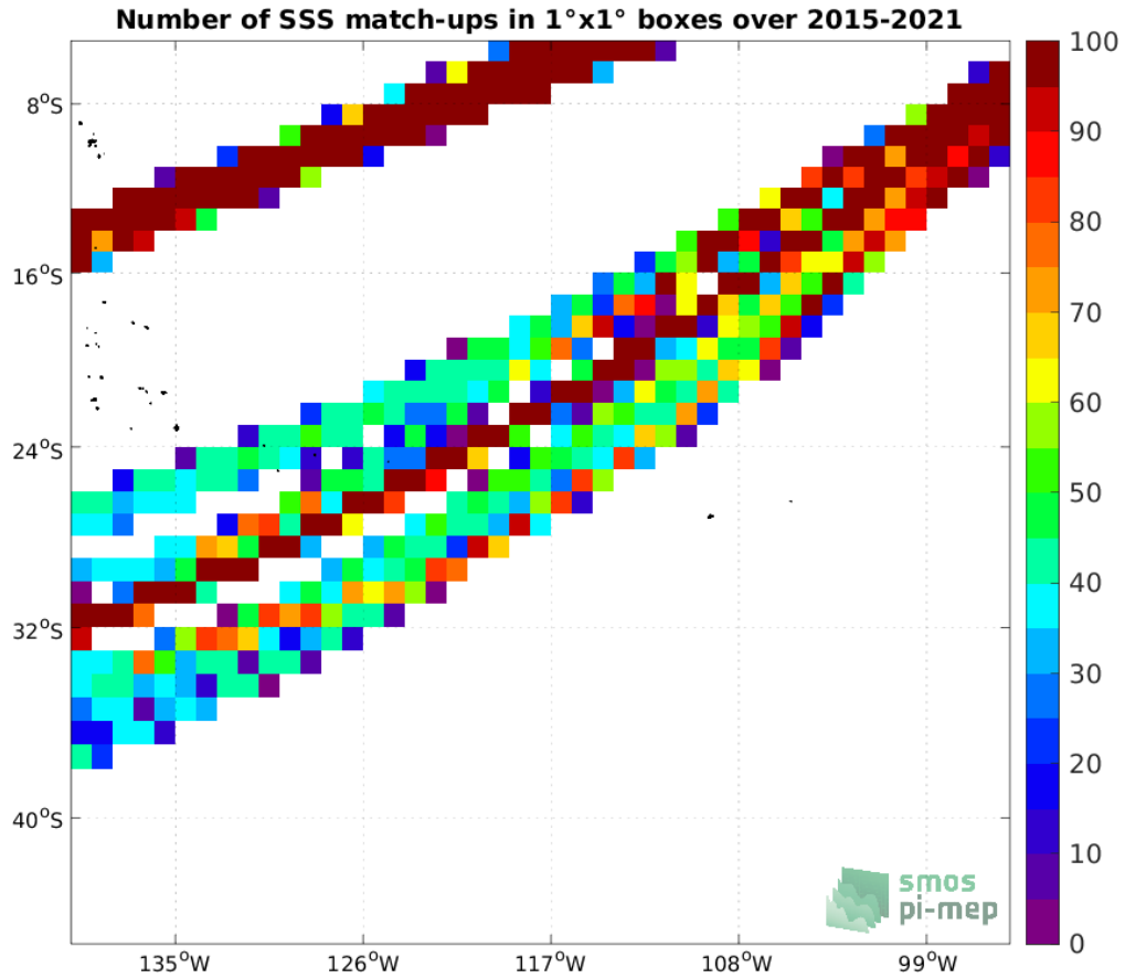
Figure 4: Number of SSS match-ups between TSG (LEGOS-DM) SSS and the SMAP SSS L3 v5.0 - 8-Day running (JPL) SSS product for the OTT zone Pi-MEP region over 1°x1° boxes and for the full satellite product period.
