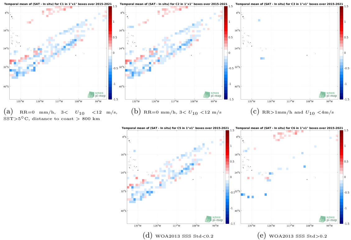
Figure 12: Temporal mean gridded over spatial boxes of size 1^\circ \times 1^\circ of \Delta SSS (SMAP SSS L3 v5.0 - 8-Day running (JPL) - TSG (LEGOS-DM)) for 5 different subdatasets corresponding to:RR=0 mm/h, 3 < U_{10} < 12 m/s, SST >5^\circ C, distance to coast > 800 km (a), RR=0 mm/h, 3 < U_{10} < 12 m/s (b), RR >1 mm/h and U_{10} < 4 m/s (c), WOA2013 SSS Std <0.2 (d), WOA2013 SSS Std >0.2 (e).
