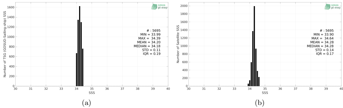
Figure 2: Histograms of SSS from TSG (GOSUD-Sailing-ship) (a) and SMAP SSS L3 v5.0 - 8-Day running (JPL) (b) considering all match-up pairs per bins of 0.1 over the OTT zone Pi-MEP region and for the full satellite product period.
