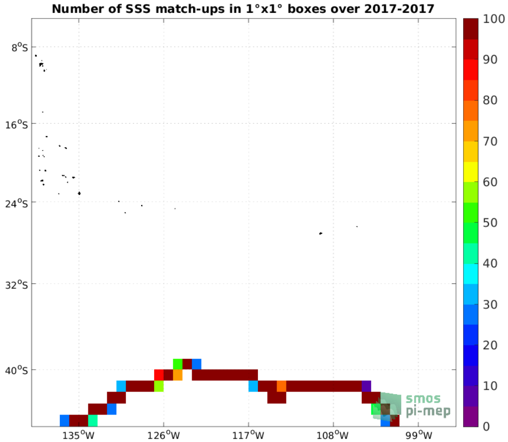
Figure 4: Number of SSS match-ups between TSG (GOSUD-Sailing-ship) SSS and the SMAP SSS L3 v5.0 - 8-Day running (JPL) SSS product for the OTT zone Pi-MEP region over 1^\circ \times 1^\circ boxes and for the full satellite product period.
