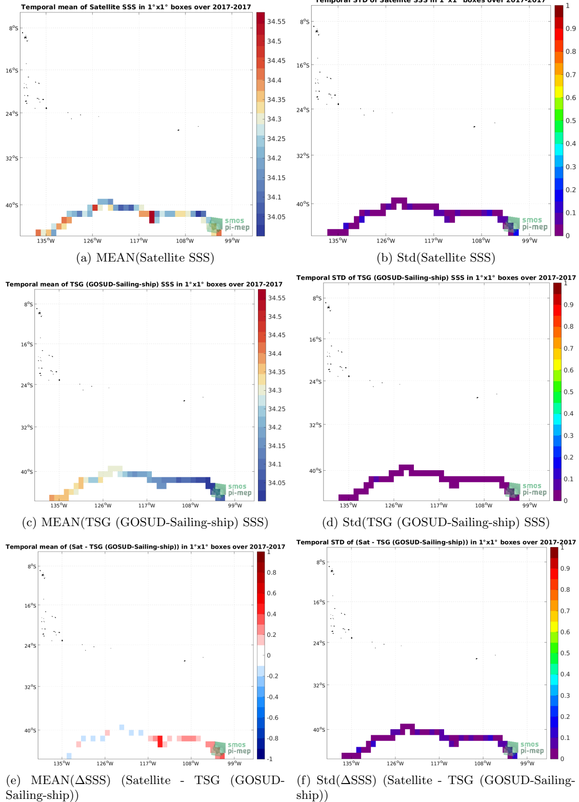
Figure 6: Temporal mean (left) and Std (right) of SSS from SMAP SSS L3 v5.0 - 8-Day running (JPL) (top), TSG (GOSUD-Sailing-ship) (middle), and of \Delta SSS (Satellite - TSG (GOSUD-Sailing-ship)). Only match-up pairs are used to generate these maps.
