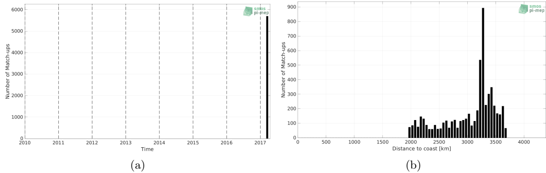
Figure 1: Number of match-ups between TSG (GOSUD-Sailing-ship) and SMAP SSS L3 v5.0 - 8-Day running (JPL) SSS as a function of time (a) and as function of the distance to coast (b) over the OTT zone Pi-MEP region and for the full satellite product period.
