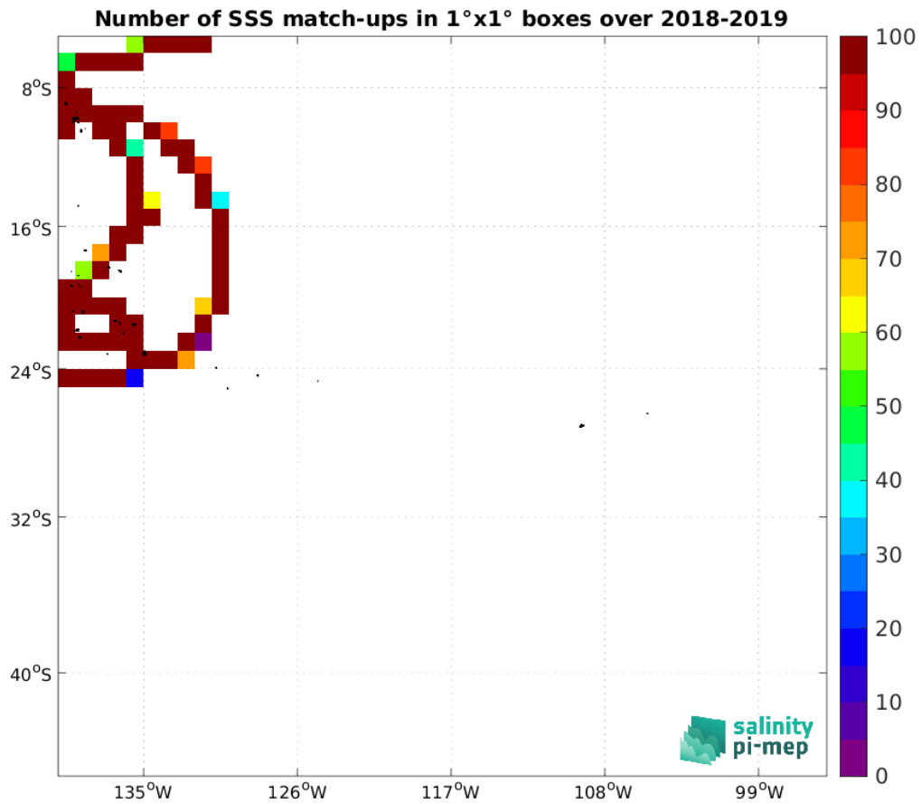
Figure 4: Number of SSS match-ups between TSG (GOSUD-Research-vessel) SSS and the SMAP SSS L3 v5.0 - 8-Day running (JPL) SSS product for the OTT zone Pi-MEP region over 1^\circ \times 1^\circ boxes and for the full satellite product period.
