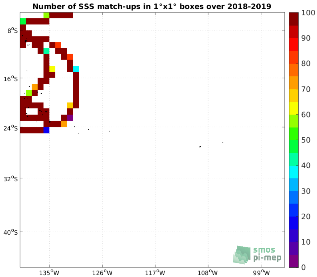
Figure 4: Number of SSS match-ups between TSG (GOSUD-Research-vessel) SSS and the SMAP SSS L3 v5.0 - 8-Day running (JPL) SSS product for the OTT zone Pi-MEP region over 1°x1° boxes and for the full satellite product period.
