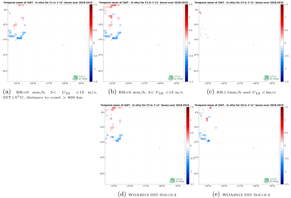
Figure 12: Temporal mean gridded over spatial boxes of size 1^{\circ}\times 1^{\circ} of \Delta SSS (SMAP SSS L3 v5.0 - 8-Day running (JPL) - TSG (GOSUD-Research-vessel)) for 5 different subdatasets corresponding to:RR=0 mm/h, 3 < U_{10} < 12 m/s, SST >5^{\circ}\text{C} , distance to coast > 800 km (a), RR=0 mm/h, 3 < U_{10} < 12 m/s (b), RR >1 mm/h and U_{10} < 4 m/s (c), WOA2013 SSS Std <0.2 (d), WOA2013 SSS Std >0.2 (e).
