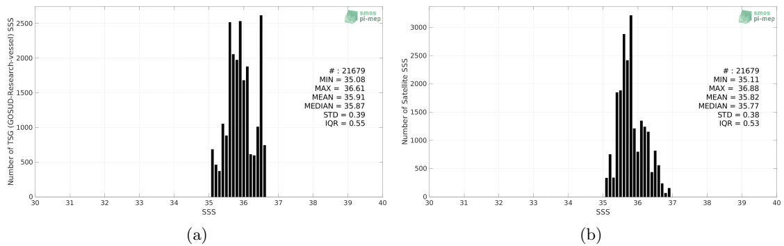
Figure 2: Histograms of SSS from TSG (GOSUD-Research-vessel) (a) and SMAP SSS L3 v5.0 - 8-Day running (JPL) (b) considering all match-up pairs per bins of 0.1 over the OTT zone Pi-MEP region and for the full satellite product period.
