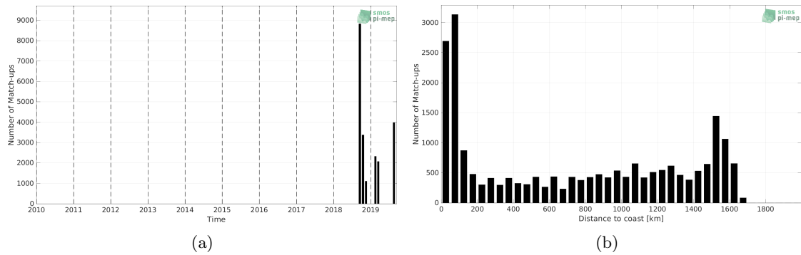
Figure 1: Number of match-ups between TSG (GOSUD-Research-vessel) and SMAP SSS L3 v5.0 - 8-Day running (JPL) SSS as a function of time (a) and as function of the distance to coast (b) over the OTT zone Pi-MEP region and for the full satellite product period.
