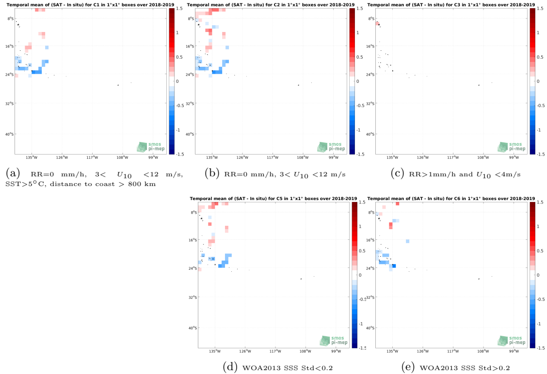
Figure 12: Temporal mean gridded over spatial boxes of size 1^\circ \times 1^\circ of \Delta SSS (SMAP SSS L3 v5.0 - 8-Day running (JPL) - TSG (GOSUD-Research-vessel)) for 5 different subdatasets corresponding to:RR=0 mm/h, 3 < U_{10} < 12 m/s, SST >5^\circ\text{C} , distance to coast > 800 km (a), RR=0 mm/h, 3 < U_{10} < 12 m/s (b), RR >1 mm/h and U_{10} < 4 m/s (c), WOA2013 SSS Std <0.2 (d), WOA2013 SSS Std >0.2 (e).
