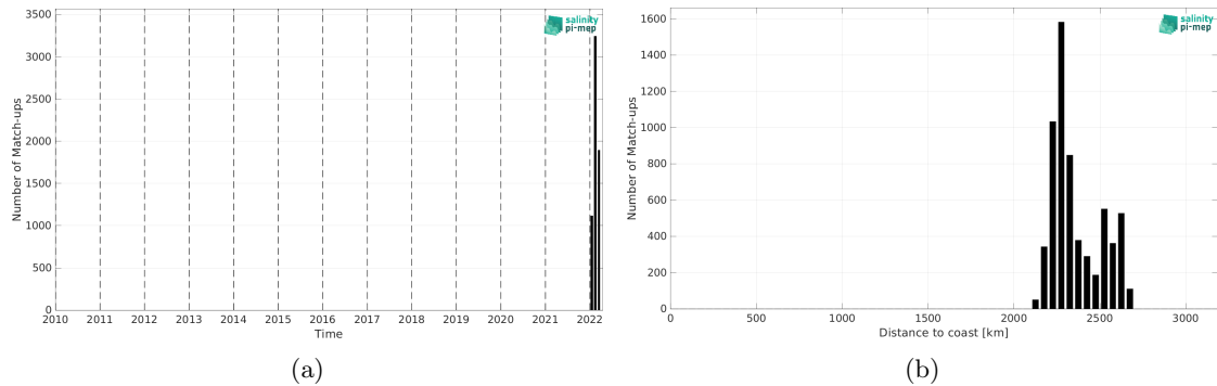
Figure 2: Number of match-ups between Sairdron and SMAP SSS L3 v5.0 - 8-Day running (JPL) SSS as a function of time (a) and as function of the distance to coast (b) over the OTT zone Pi-MEP region and for the full satellite product period.
