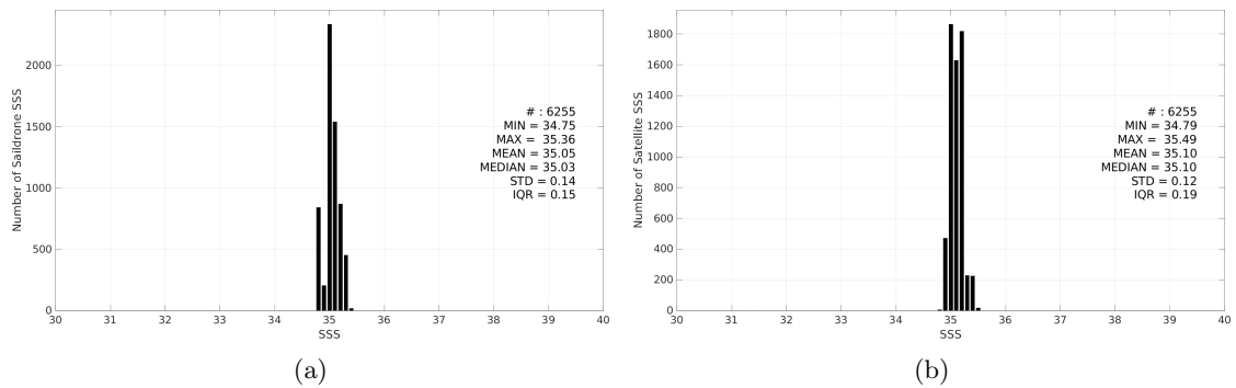
Figure 3: Histograms of SSS from Sairdron (a) and SMAP SSS L3 v5.0 - 8-Day running (JPL) (b) considering all match-up pairs per bins of 0.1 over the OTT zone Pi-MEP region and for the full satellite product period.
