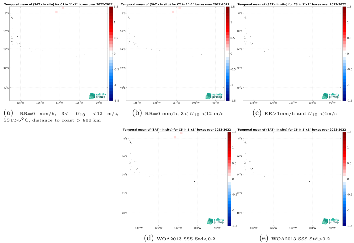
Figure 14: Temporal mean gridded over spatial boxes of size 1^\circ \times 1^\circ of \Delta SSS (SMAP SSS L3 v5.0 - 8-Day running (JPL) - Sairdrone) for 5 different subdatasets corresponding to: RR=0 mm/h, 3 < U_{10} < 12 m/s, SST > 5^\circ C , distance to coast > 800 km (a), RR=0 mm/h, 3 < U_{10} < 12 m/s (b), RR > 1 mm/h and U_{10} < 4 m/s (c), WOA2013 SSS Std < 0.2 (d), WOA2013 SSS Std > 0.2 (e).
