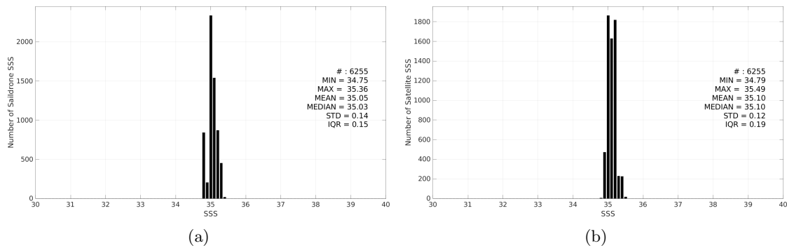
Figure 3: Histograms of SSS from Saildrone (a) and SMAP SSS L3 v5.0 - 8-Day running (JPL) (b) considering all match-up pairs per bins of 0.1 over the OTT zone Pi-MEP region and for the full satellite product period.
