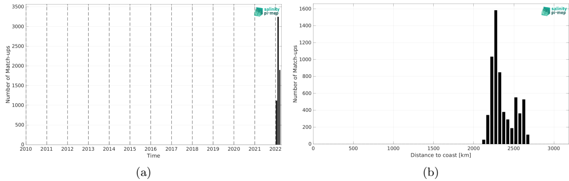
Figure 2: Number of match-ups between Saildrone and SMAP SSS L3 v5.0 - 8-Day running (JPL) SSS as a function of time (a) and as function of the distance to coast (b) over the OTT zone Pi-MEP region and for the full satellite product period.
