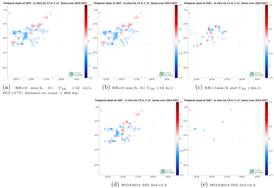
Figure 11: Temporal mean gridded over spatial boxes of size 1^\circ \times 1^\circ of \Delta SSS (SMAP SSS L3 v5.0 - 8-Day running (JPL) - Surface drifters) for 5 different subdatasets corresponding to:RR=0 mm/h, 3 < U_{10} < 12 m/s, SST >5^\circ C, distance to coast > 800 km (a), RR=0 mm/h, 3 < U_{10} < 12 m/s (b), RR >1 mm/h and U_{10} < 4 m/s (c), WOA2013 SSS Std <0.2 (d), WOA2013 SSS Std >0.2 (e).
