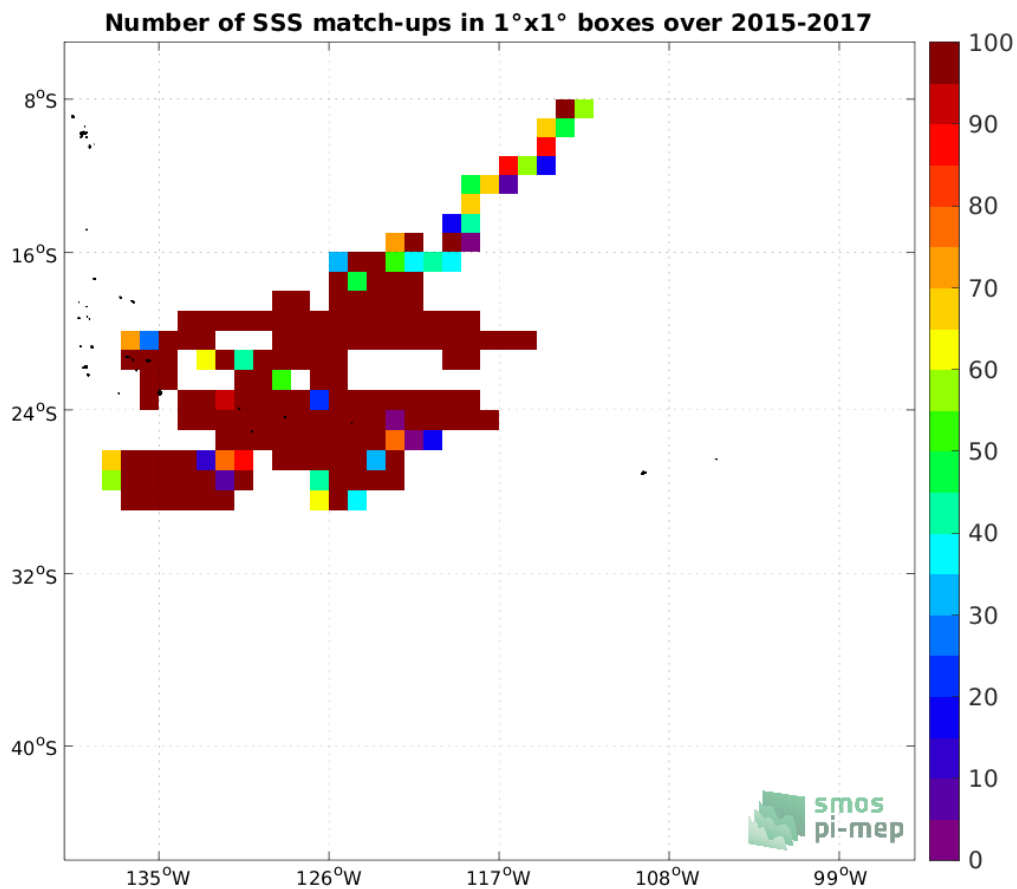
Figure 3: Number of SSS match-ups between Surface drifters SSS and the SMAP SSS L3 v5.0 - 8-Day running (JPL) SSS product for the OTT zone Pi-MEP region over 1°x1° boxes and for the full satellite product period.
