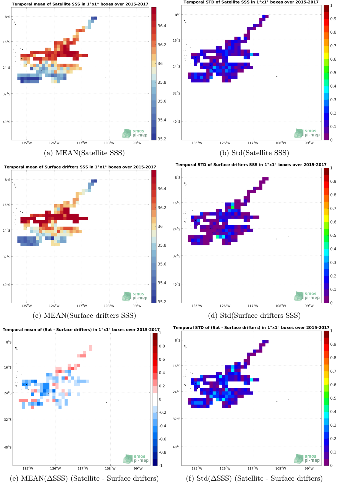
Figure 5: Temporal mean (left) and Std (right) of SSS from SMAP SSS L3 v5.0 - 8-Day running (JPL) (top), Surface drifters (middle), and of \Delta SSS (Satellite - Surface drifters). Only match-up pairs are used to generate these maps.
