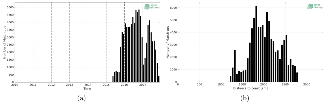
Figure 1: Number of match-ups between Surface drifters and SMAP SSS L3 v5.0 - 8-Day running (JPL) SSS as a function of time (a) and as function of the distance to coast (b) over the OTT zone Pi-MEP region and for the full satellite product period.
