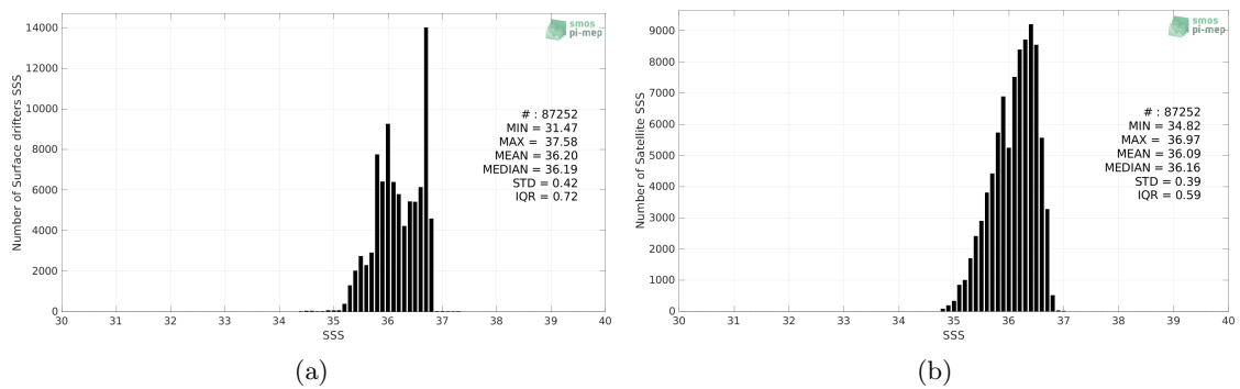
Figure 2: Histograms of SSS from Surface drifters (a) and SMAP SSS L3 v5.0 - 8-Day running (JPL) (b) considering all match-up pairs per bins of 0.1 over the OTT zone Pi-MEP region and for the full satellite product period.
