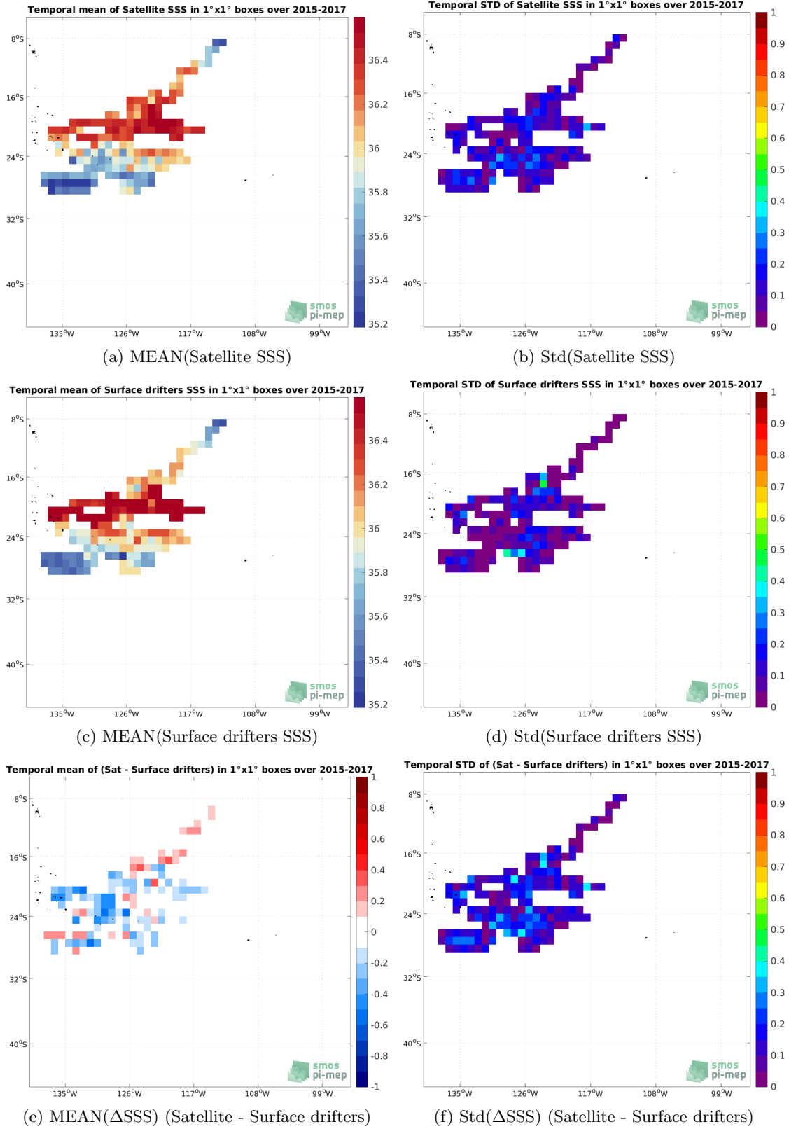
Figure 5: Temporal mean (left) and Std (right), of SSS from SMAP SSS L3 v5.0 - 8-Day running (JPL) (top), Surface drifters (middle), and of \Delta SSS (Satellite - Surface drifters). Only match-up pairs are used to generate these maps.
