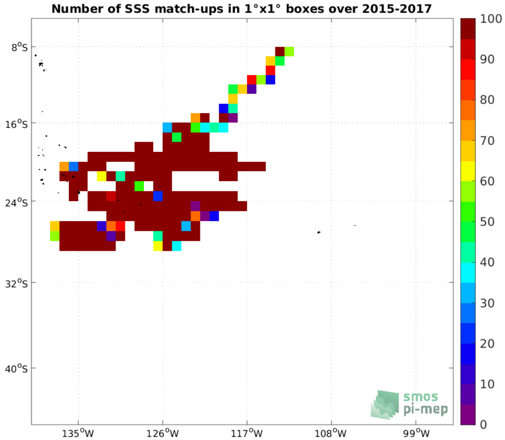
Figure 3: Number of SSS match-ups between Surface drifters SSS and the SMAP SSS L3 v5.0 - 8-Day running (JPL) SSS product for the OTT zone Pi-MEP region over 1^\circ \times 1^\circ boxes and for the full satellite product period.
