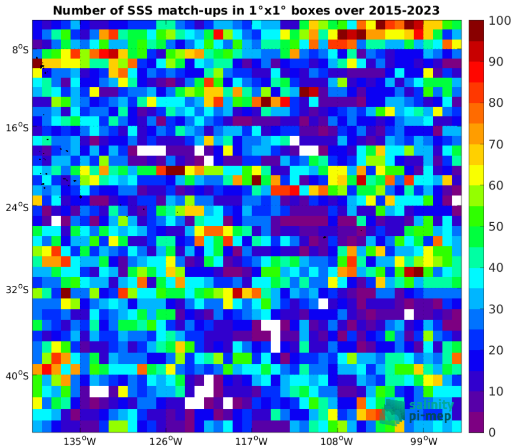
Figure 4: Number of SSS match-ups between Argo SSS and the SMAP SSS L3 v5.0 - 8-Day running (JPL) SSS product for the OTT zone Pi-MEP region over 1°x1° boxes and for the full satellite product period.
