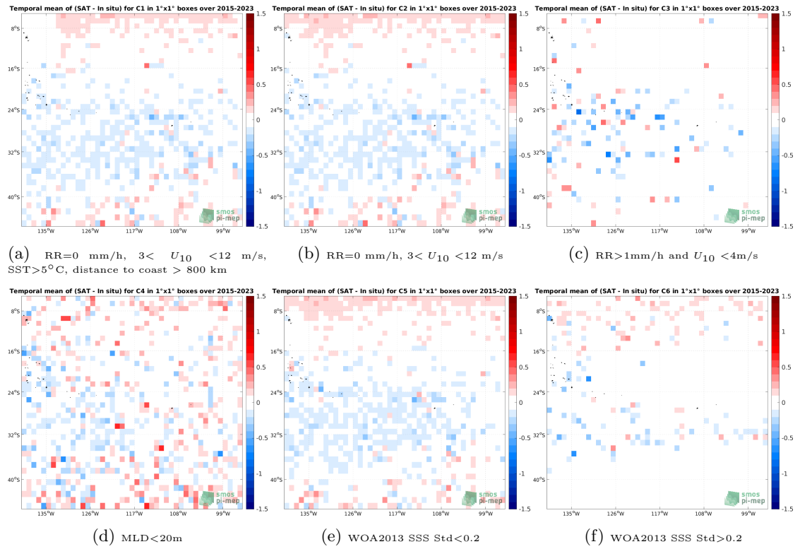
Figure 12: Temporal mean gridded over spatial boxes of size 1^\circ \times 1^\circ of \Delta SSS (SMAP SSS L3 v5.0 - 8-Day running (JPL) - Argo) for 6 different subdatasets corresponding to:RR=0 mm/h, 3 < U_{10} < 12 m/s, SST >5^\circ C, distance to coast > 800 km (a), RR=0 mm/h, 3 < U_{10} < 12 m/s (b), RR >1 mm/h and U_{10} < 4 m/s (c),MLD <20 m (d),WOA2013 SSS Std <0.2 (e),WOA2013 SSS Std >0.2 (f).
