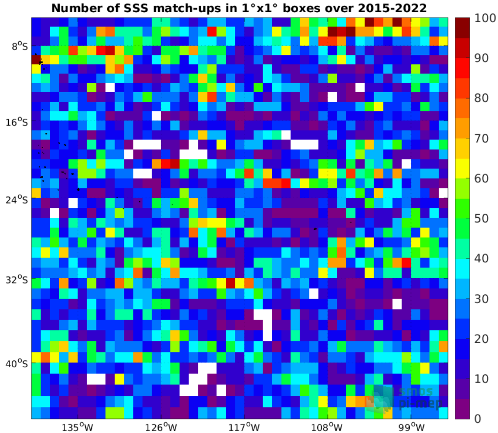
Figure 4: Number of SSS match-ups between Argo SSS and the SMAP SSS L3 v5.0 - 8-Day running (JPL) SSS product for the OTT zone Pi-MEP region over 1^\circ \times 1^\circ boxes and for the full satellite product period.
