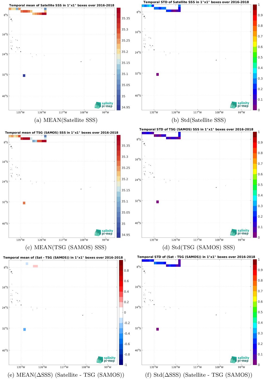
Figure 7: Temporal mean (left) and Std (right) of SSS from SMAP SSS L3 v5.0 - Monthly (JPL) (top), TSG (SAMOS) (middle), and of \Delta SSS (Satellite - TSG (SAMOS)). Only match-up pairs are used to generate these maps.
