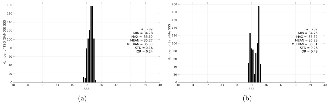
Figure 3: Histograms of SSS from TSG (SAMOS) (a) and SMAP SSS L3 v5.0 - Monthly (JPL) (b) considering all match-up pairs per bins of 0.1 over the OTT zone Pi-MEP region and for the full satellite product period.
