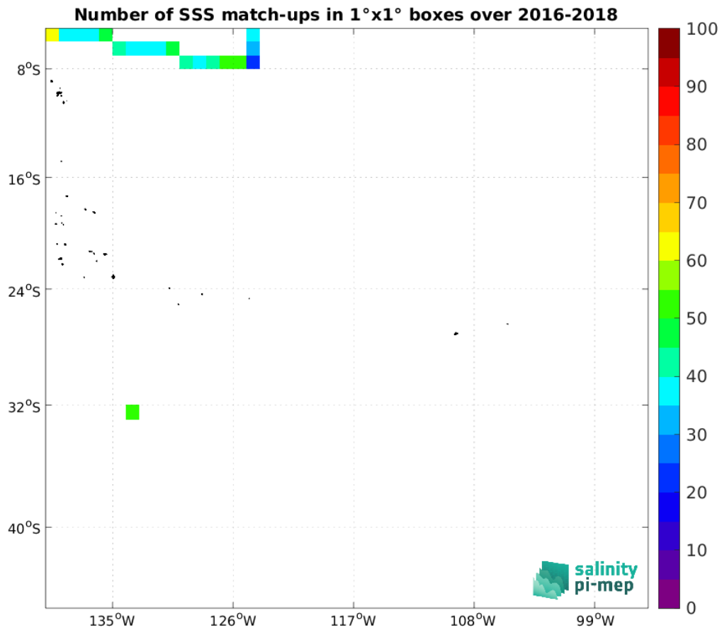
Figure 5: Number of SSS match-ups between TSG (SAMOS) SSS and the SMAP SSS L3 v5.0 - Monthly (JPL) SSS product for the OTT zone Pi-MEP region over 1^\circ \times 1^\circ boxes and for the full satellite product period.
