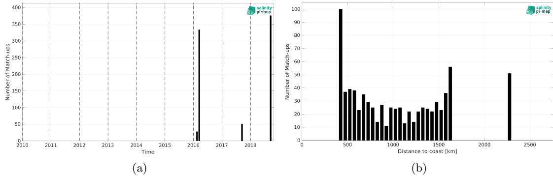
Figure 2: Number of match-ups between TSG (SAMOS) and SMAP SSS L3 v5.0 - Monthly (JPL) SSS as a function of time (a) and as function of the distance to coast (b) over the OTT zone Pi-MEP region and for the full satellite product period.
