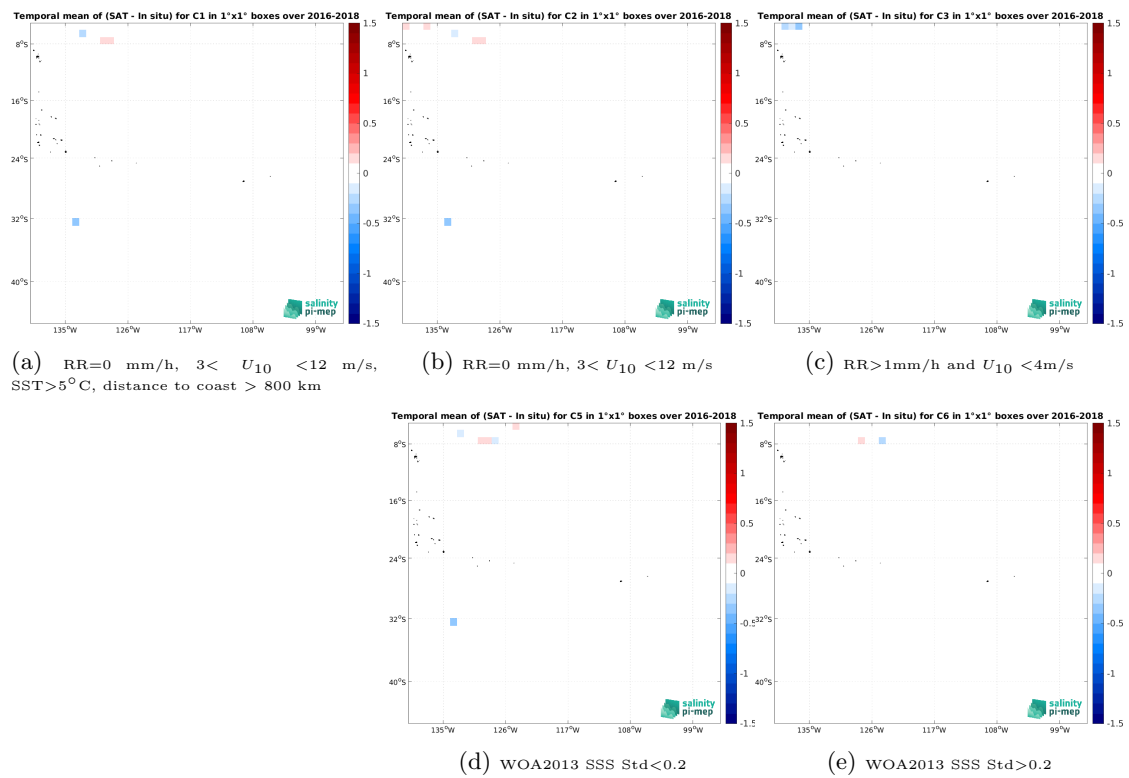
Figure 14: Temporal mean gridded over spatial boxes of size 1^\circ \times 1^\circ of \Delta SSS (SMAP SSS L3 v5.0 - Monthly (JPL) - TSG (SAMOS)) for 5 different subdatasets corresponding to: RR=0 mm/h, 3 < U_{10} < 12 m/s, SST > 5^\circ C , distance to coast > 800 km (a), RR=0 mm/h, 3 < U_{10} < 12 m/s (b), RR > 1 mm/h and U_{10} < 4 m/s (c), WOA2013 SSS Std < 0.2 (d), WOA2013 SSS Std > 0.2 (e).
