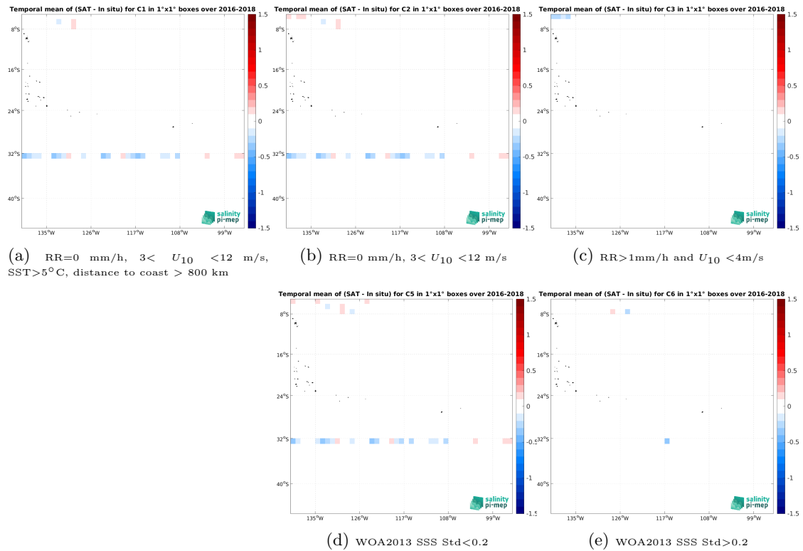
Figure 12: Temporal mean gridded over spatial boxes of size 1^\circ \times 1^\circ of \Delta\text{SSS} (SMAP SSS L3 v5.0 - Monthly (JPL) - TSG (SAMOS)) for 5 different subdatasets corresponding to: \text{RR}=0 mm/h, 3 < U_{10} < 12 m/s, \text{SST} > 5^\circ\text{C} , distance to coast > 800 km (a), \text{RR}=0 mm/h, 3 < U_{10} < 12 m/s (b), \text{RR} > 1 mm/h and U_{10} < 4 m/s (c), WOA2013 SSS Std < 0.2 (d), WOA2013 SSS Std > 0.2 (e).
