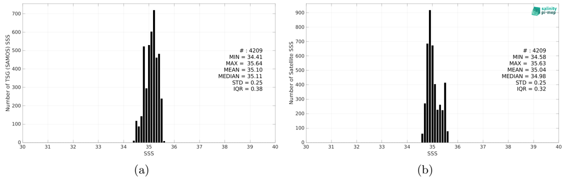
Figure 2: Histograms of SSS from TSG (SAMOS) (a) and SMAP SSS L3 v5.0 - Monthly (JPL) (b) considering all match-up pairs per bins of 0.1 over the OTT zone Pi-MEP region and for the full satellite product period.
