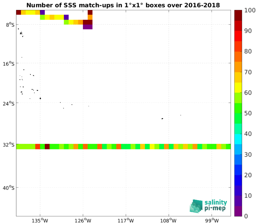
Figure 4: Number of SSS match-ups between TSG (SAMOS) SSS and the SMAP SSS L3 v5.0 - Monthly (JPL) SSS product for the OTT zone Pi-MEP region over 1^\circ \times 1^\circ boxes and for the full satellite product period.
