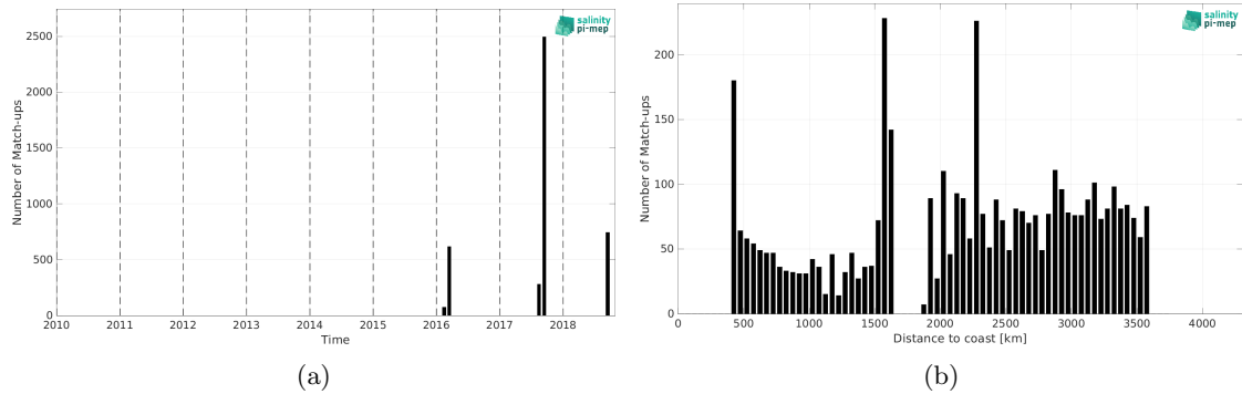
Figure 1: Number of match-ups between TSG (SAMOS) and SMAP SSS L3 v5.0 - Monthly (JPL) SSS as a function of time (a) and as function of the distance to coast (b) over the OTT zone Pi-MEP region and for the full satellite product period.
