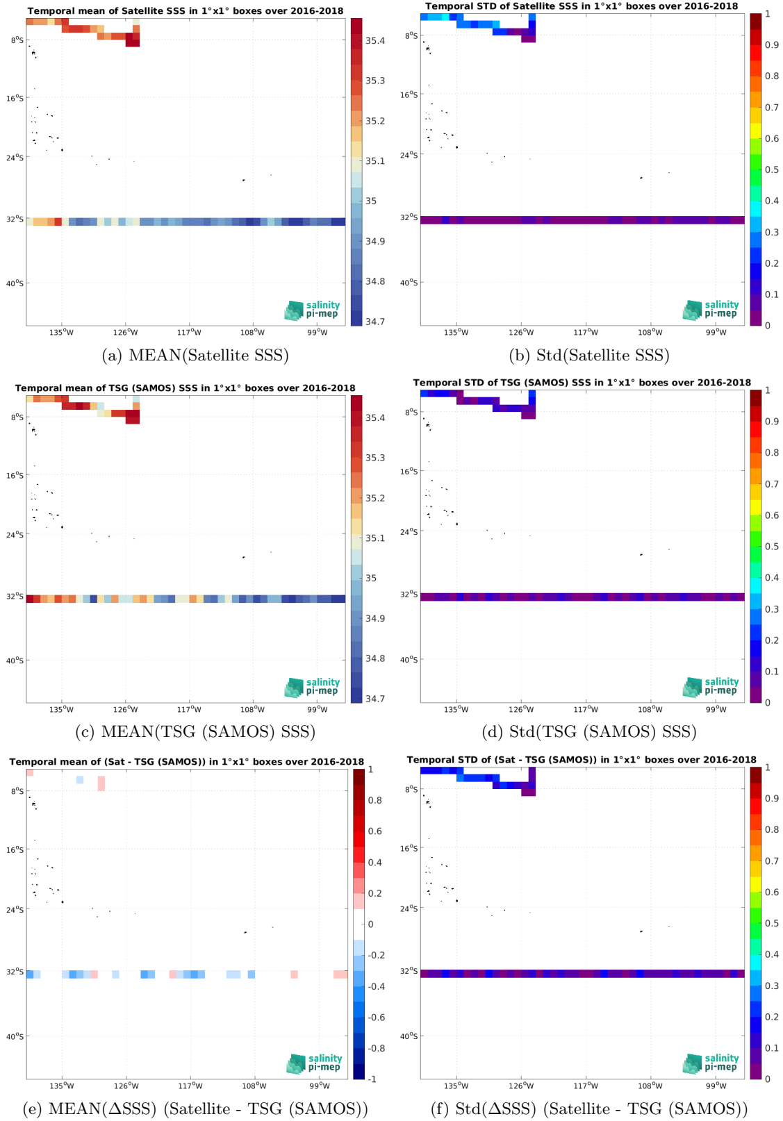
Figure 6: Temporal mean (left) and Std (right) of SSS from SMAP SSS L3 v5.0 - Monthly (JPL) (top), TSG (SAMOS) (middle), and of \Delta SSS (Satellite - TSG (SAMOS)). Only match-up pairs are used to generate these maps.
