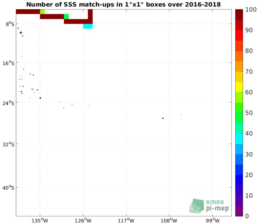
Figure 4: Number of SSS match-ups between TSG (SAMOS) SSS and the SMAP SSS L3 v5.0 - Monthly (JPL) SSS product for the OTT zone Pi-MEP region over 1°x1° boxes and for the full satellite product period.
