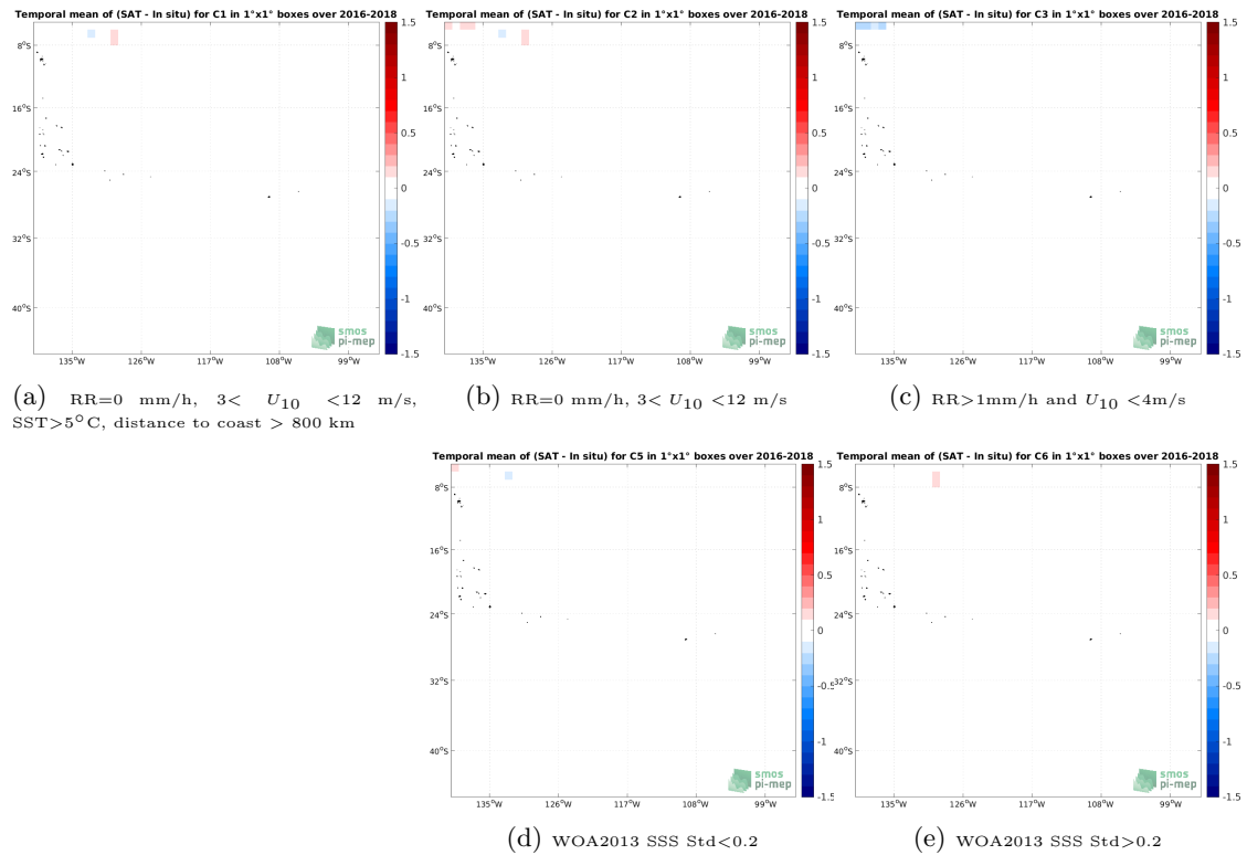
Figure 12: Temporal mean gridded over spatial boxes of size 1^\circ \times 1^\circ of \Delta SSS (SMAP SSS L3 v5.0 - Monthly (JPL) - TSG (SAMOS)) for 5 different subdatasets corresponding to:RR=0 mm/h, 3 < U_{10} < 12 m/s, SST >5^\circ\text{C} , distance to coast > 800 km (a), RR=0 mm/h, 3 < U_{10} < 12 m/s (b), RR >1 mm/h and U_{10} < 4 m/s (c), WOA2013 SSS Std <0.2 (d), WOA2013 SSS Std >0.2 (e).
