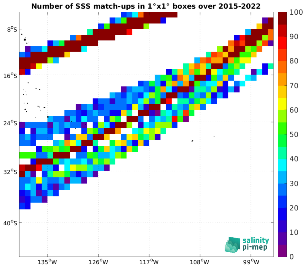
Figure 5: Number of SSS match-ups between TSG (LEGOS-DM) SSS and the SMAP SSS L3 v5.0 - Monthly (JPL) SSS product for the OTT zone Pi-MEP region over 1°x1° boxes and for the full satellite product period.
