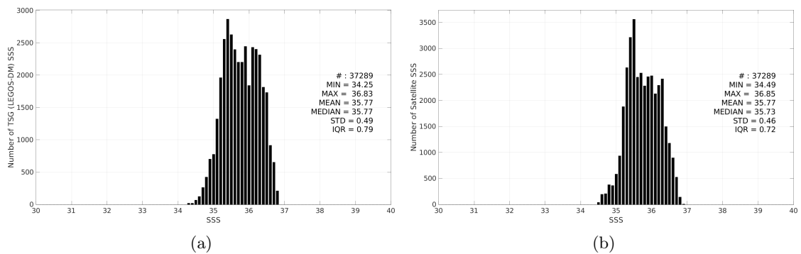
Figure 3: Histograms of SSS from TSG (LEGOS-DM) (a) and SMAP SSS L3 v5.0 - Monthly (JPL) (b) considering all match-up pairs per bins of 0.1 over the OTT zone Pi-MEP region and for the full satellite product period.
