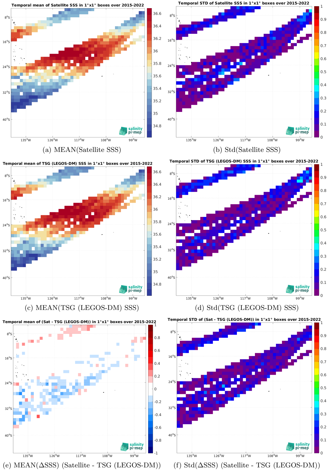
Figure 7: Temporal mean (left) and Std (right) of SSS from SMAP SSS L3 v5.0 - Monthly (JPL) (top), TSG (LEGOS-DM) (middle), and of \Delta SSS (Satellite - TSG (LEGOS-DM)). Only match-up pairs are used to generate these maps.
