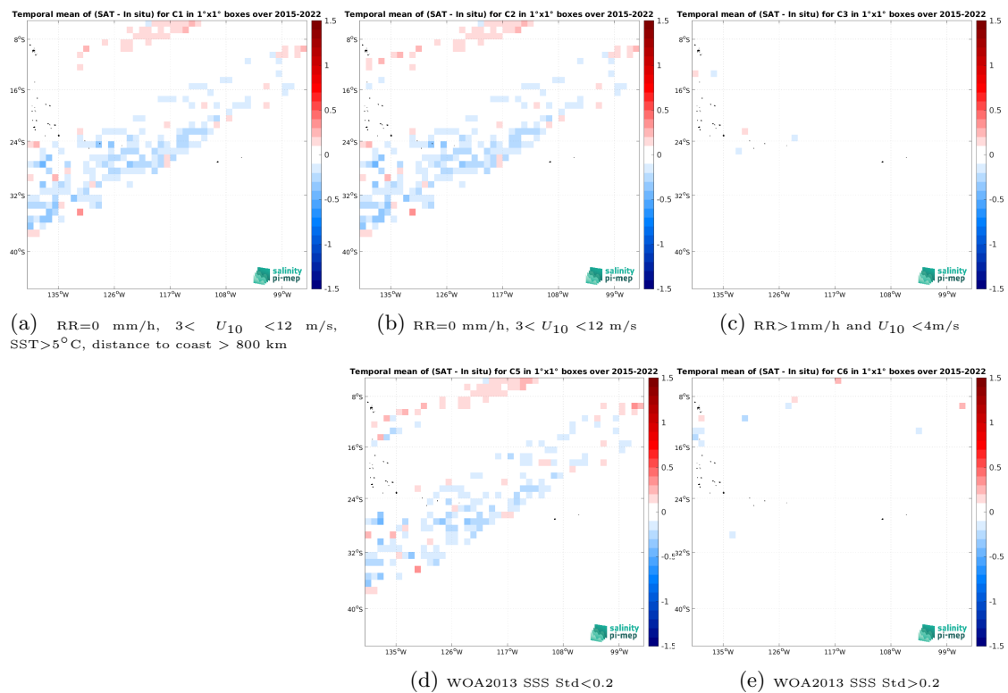
Figure 14: Temporal mean gridded over spatial boxes of size 1^\circ \times 1^\circ of \Delta SSS (SMAP SSS L3 v5.0 - Monthly (JPL) - TSG (LEGOS-DM)) for 5 different subdatasets corresponding to:RR=0 mm/h, 3 < U_{10} < 12 m/s, SST >5^\circ\text{C} , distance to coast > 800 km (a), RR=0 mm/h, 3 < U_{10} < 12 m/s (b), RR >1 mm/h and U_{10} < 4 m/s (c), WOA2013 SSS Std <0.2 (d), WOA2013 SSS Std >0.2 (e).
