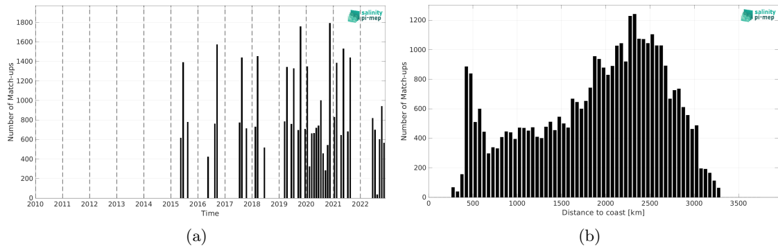
Figure 2: Number of match-ups between TSG (LEGOS-DM) and SMAP SSS L3 v5.0 - Monthly (JPL) SSS as a function of time (a) and as function of the distance to coast (b) over the OTT zone Pi-MEP region and for the full satellite product period.
