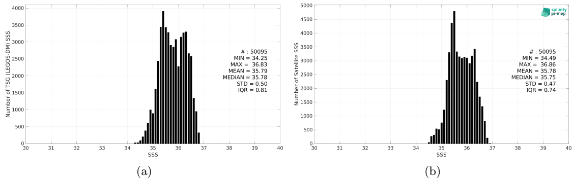
Figure 2: Histograms of SSS from TSG (LEGOS-DM) (a) and SMAP SSS L3 v5.0 - Monthly (JPL) (b) considering all match-up pairs per bins of 0.1 over the OTT zone Pi-MEP region and for the full satellite product period.
