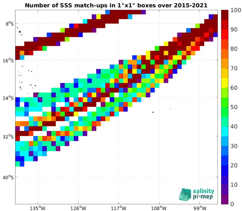
Figure 4: Number of SSS match-ups between TSG (LEGOS-DM) SSS and the SMAP SSS L3 v5.0 - Monthly (JPL) SSS product for the OTT zone Pi-MEP region over 1°x1° boxes and for the full satellite product period.
