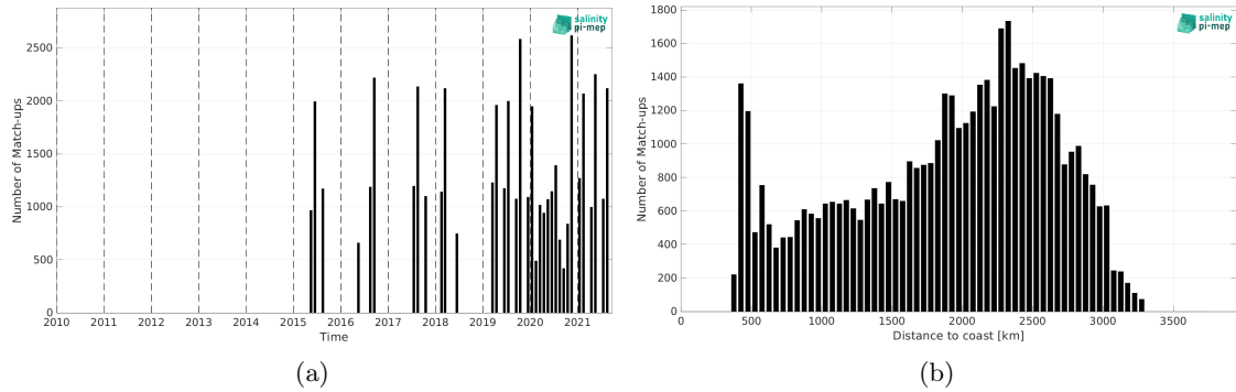
Figure 1: Number of match-ups between TSG (LEGOS-DM) and SMAP SSS L3 v5.0 - Monthly (JPL) SSS as a function of time (a) and as function of the distance to coast (b) over the OTT zone Pi-MEP region and for the full satellite product period.
