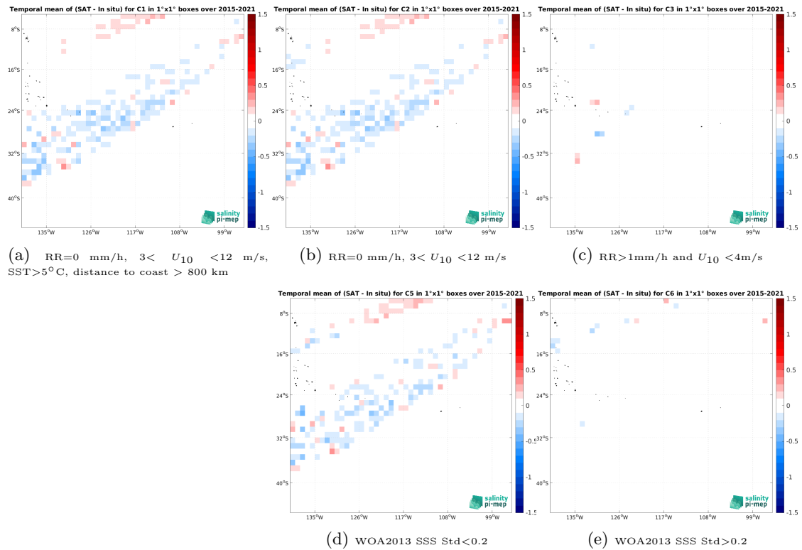
Figure 12: Temporal mean gridded over spatial boxes of size 1^\circ \times 1^\circ of \Delta SSS (SMAP SSS L3 v5.0 - Monthly (JPL) - TSG (LEGOS-DM)) for 5 different subdatasets corresponding to:RR=0 mm/h, 3 < U_{10} < 12 m/s, SST >5^\circ C, distance to coast > 800 km (a), RR=0 mm/h, 3 < U_{10} < 12 m/s (b), RR >1 mm/h and U_{10} < 4 m/s (c), WOA2013 SSS Std <0.2 (d), WOA2013 SSS Std >0.2 (e).
